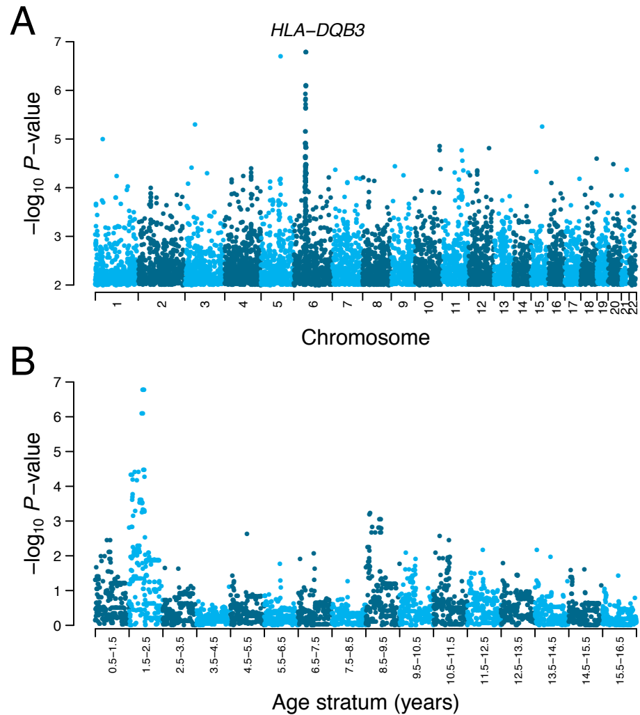
Fig 3. Genome-wide associations with BMI. A: GWAS at age stratum 1.5 – 2.5. B: Association peak of chromosome 6 across age strata. The region shown has physical coordinates 6 : 32676320 – 32683820 and was centered at the variant with the strongest association.
