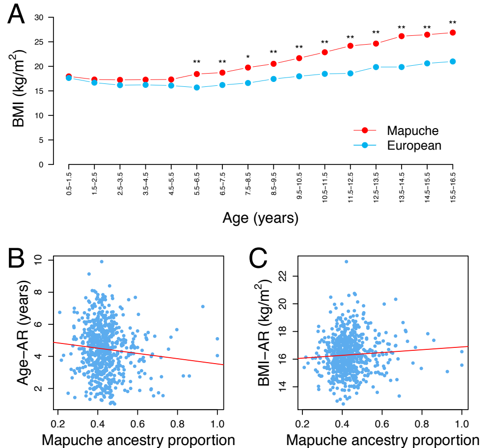
Fig 2. Effect of global Mapuche ancestry on BMI trajectory, Age-AR and BMI-AR. A: BMI (kg/m 2 ) estimated at each age stratum for predicted individuals with 100% Mapuche (red line) and 100% European global ancestry (blue line). B: Linear model of Age-AR with Mapuche ancestry as covariate. C: Linear model of BMI-AR with Mapuche ancestry as covariate.
