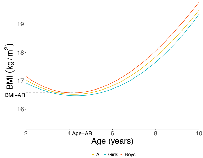
Fig 1. Estimation of Age-AR and BMI-AR. Fitted BMI ( \text{kg}/\text{m}^2 ) curves over time (years) in the whole cohort as well as in boys and girls considered separately. Vertical and horizontal dotted lines pinpoint the observed mean Age-AR and mean BMI-AR in boys and girls.
