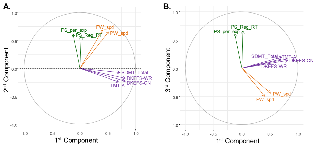
Figure 1. PCA Component loadings of variables on the first three components. A) First and second components. B) First and third components.
