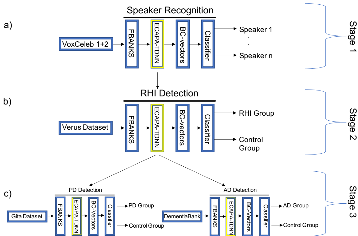
Figure 1: Depiction of the training process used in this study. a) An ECAPA-TDNN model is trained to classify speaker identities with the Voxceleb1+2 dataset. b) The pretrained ECAPA-TDNN model from “a)” is fine-tuned on the Verus dataset to differentiate the RHI from control group. c) Finally, the pre-trained ECAPA-TDNN model from “b)” is fine-tuned on either the DementiaBank or Gita dataset in order to detect AD or PD, respectively.
