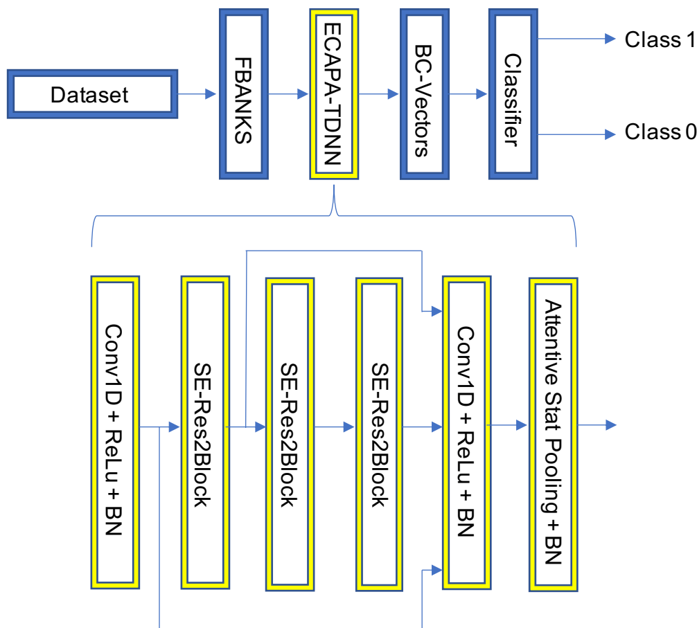
Figure 3: Simplified depiction of the ECAPA-TDNN model used in this study.
