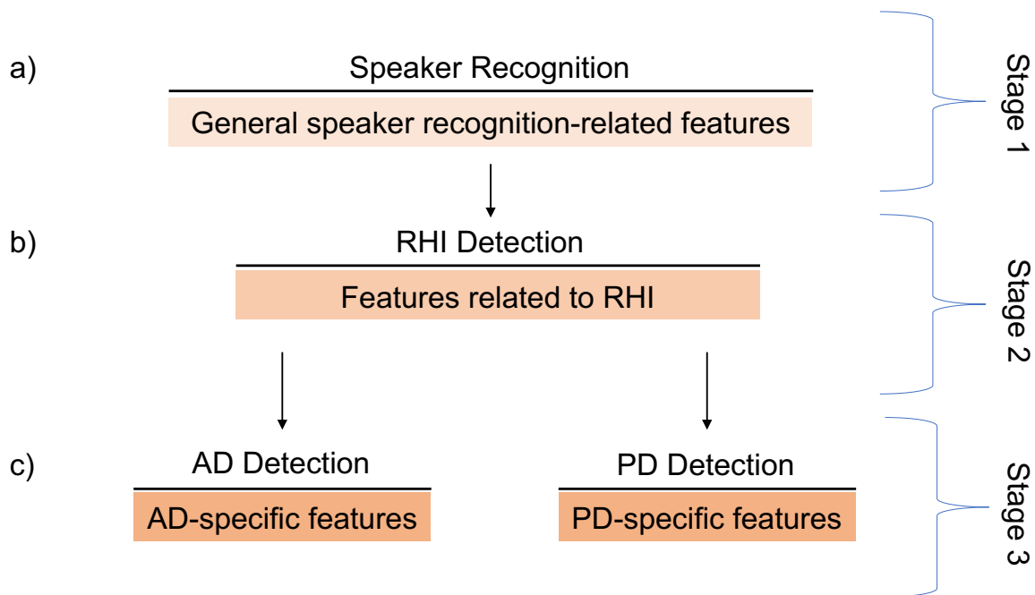
Figure 2: Depiction of the proposed feature learning resulting from the multi-step transfer learning approach. a) Stage 1 results in the learning of low-level features pertinent to speaker recognition. b) Stage 2 involves the transfer of the low-level features from Stage 1 and the learning of RHI-related features. c) Stage 3 involves the transfer of features from Stage 1 and 2 as well as the learning of AD or PD-specific features.
