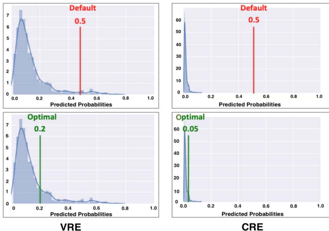
Figure 2. Threshold Value for Converting Predicted Probabilities to Binary Predictions
