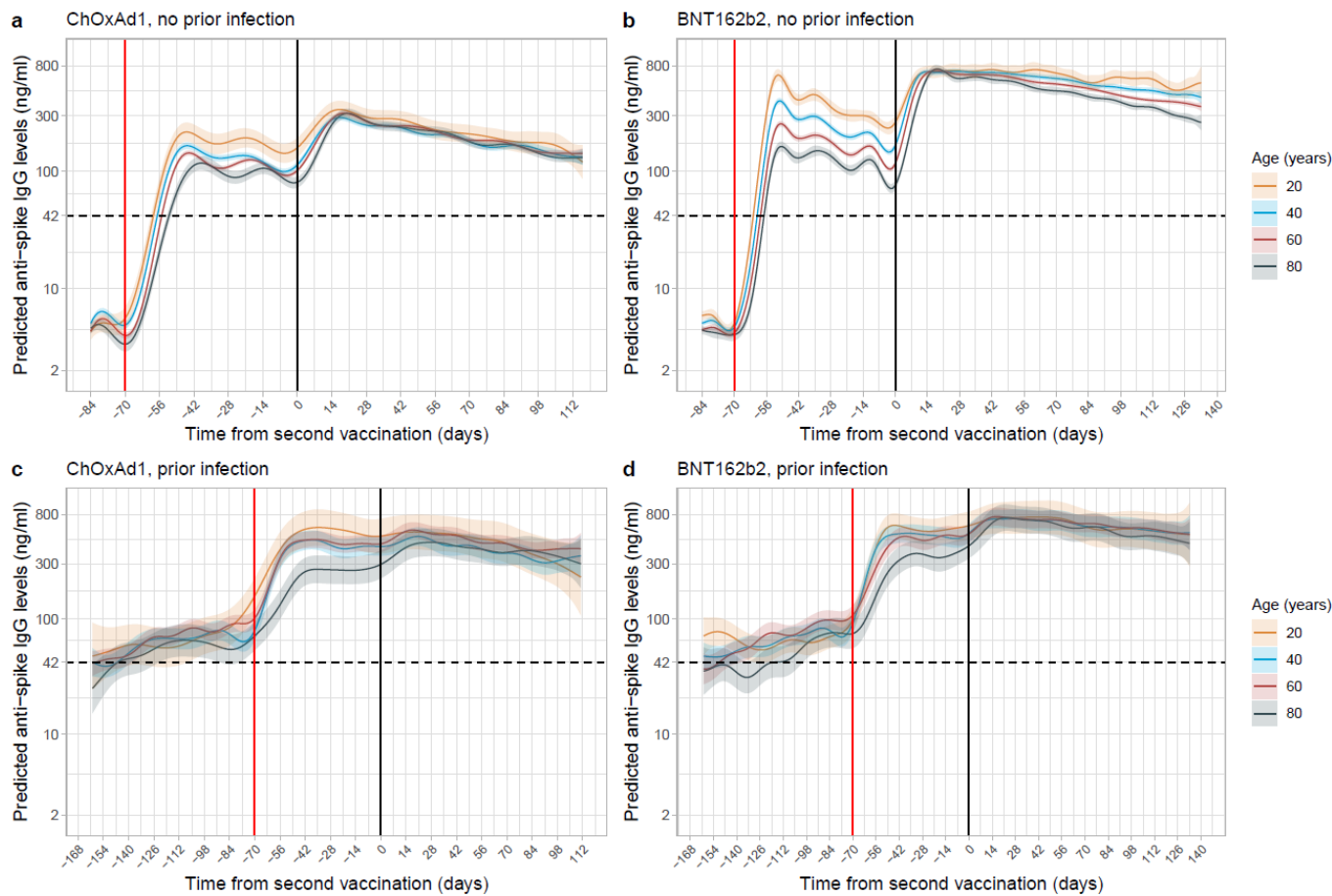
Figure 2. Predicted anti-spike IgG levels in participants with 10-week dosing interval by time from second vaccination according to age, vaccine type and prior infection status. a , Participants who received two doses of ChAdOx1 without prior infection. b , Participants who received two doses of BNT162b2 without prior infection. c , Participants who received two doses of ChAdOx1 with prior infection. d , Participants who received two doses of BNT162b2 with prior infection. Different x axis scales reflect different durations of follow-up post-vaccination in the different cohorts. Predicted levels are plotted on a log scale. Black dotted line indicates the threshold of IgG positivity (42 ng/ml). Red solid line indicates the first vaccination and black solid line indicates the second vaccination. Line colour indicates response predicted for age 20, 40, 60, and 80 years. See Figure S3, S5 for other dosing interval groups; see Figure 3 for comparison of vaccine type by age. The 95% CIs are calculated by prediction \pm 1.96 \times standard error of the prediction.
