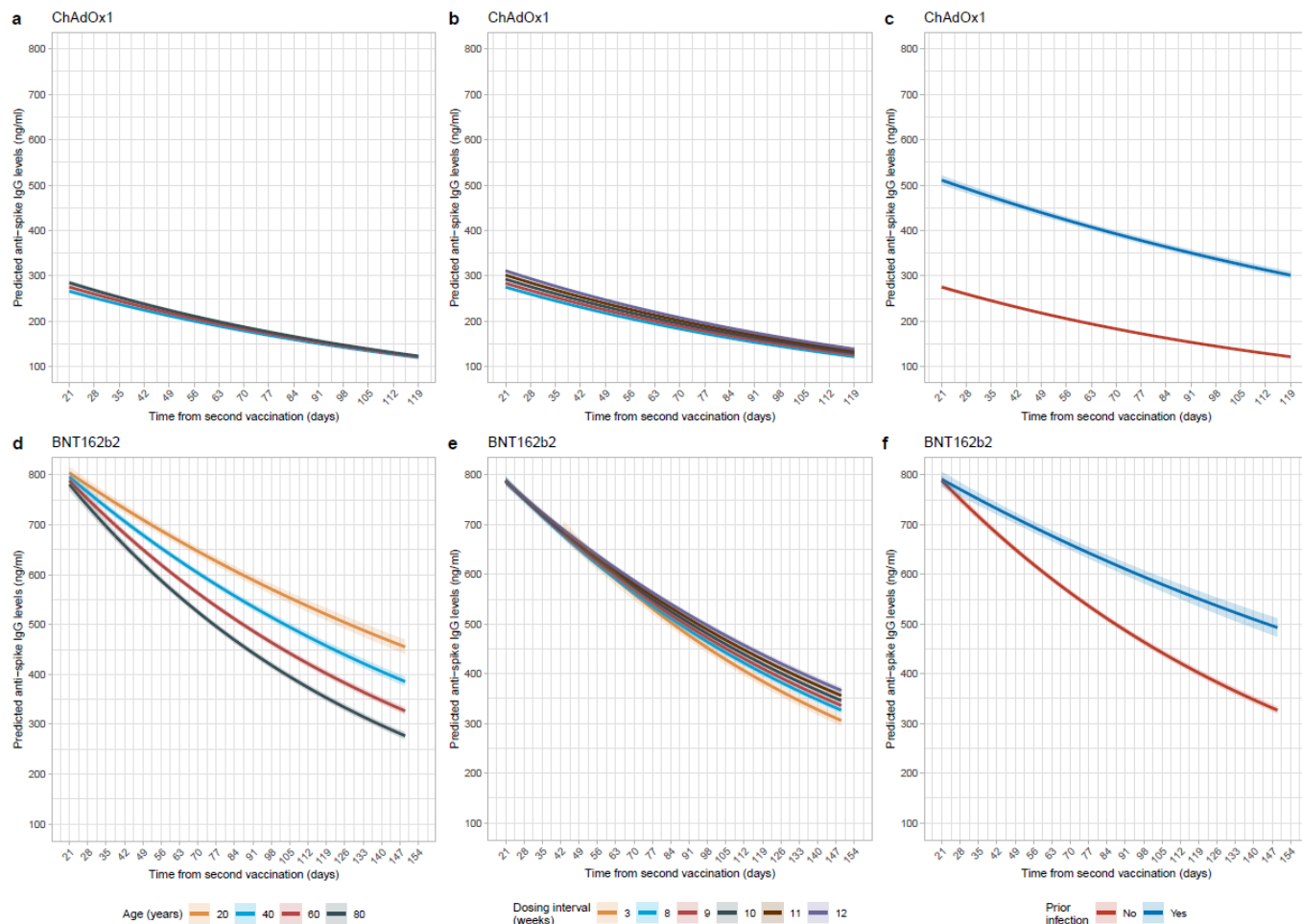
Figure 4. Posterior predicted trajectories of anti-spike IgG levels from 21 days post-second dose by age (panel a, d), dosing interval (panel b, e), and prior infection status (panel c, f). Panel a,b,c show participants who received two doses of ChAdOx1. Panel d,e,f show participants who received two doses of BNT162b2. Plotted at reference categories: 60 years, female, white ethnicity, not reporting a long-term health condition, not a healthcare worker, deprivation percentile=60, 8-week dosing interval, and no prior infection. In panel a, 20-year-old group is not plotted because the vast majority of those receiving ChAdOx1 were \geq 40 years.
