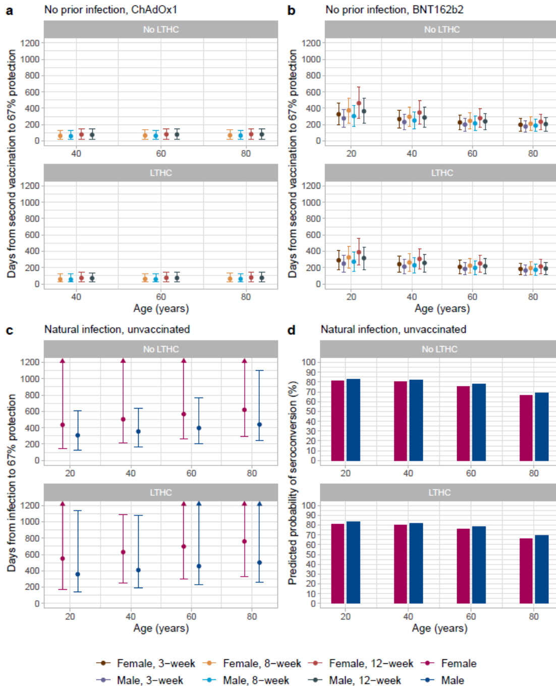
Figure 7. Posterior predicted days (95% credible interval) from the second vaccination/infection to the threshold level associated with 67% protection (ChAdOx1: 191 ng/ml, BNT162b2: 169 ng/ml, unvaccinated: 59 ng/ml). a , In participants without prior infection and vaccinated with ChAdOx1. b , In participants without prior infection and vaccinated with BNT162b2. c , In unvaccinated participants who had natural infection. d , Predicted probability of seroconverting in unvaccinated participants who had natural infection, based on a previous model on seroconversion 16 . Estimates were separated by age, sex, dosing interval, long-term health condition (LTHC), and vaccine type for vaccinated people, and by age, sex, and LTHC for unvaccinated people. y-axis is truncated at 1200 days for visualisation. For ChAdOx1, 20-year-old group is not plotted because the vast majority of those receiving ChAdOx1 were \geq 40 years. Panel a , b , c are conditional on participants having antibody response/seroconverting (see section of “Vaccine non-responders” for ChAdOx1 and BNT162b2, and discussion in a previous publication 16 for unvaccinated individuals).
