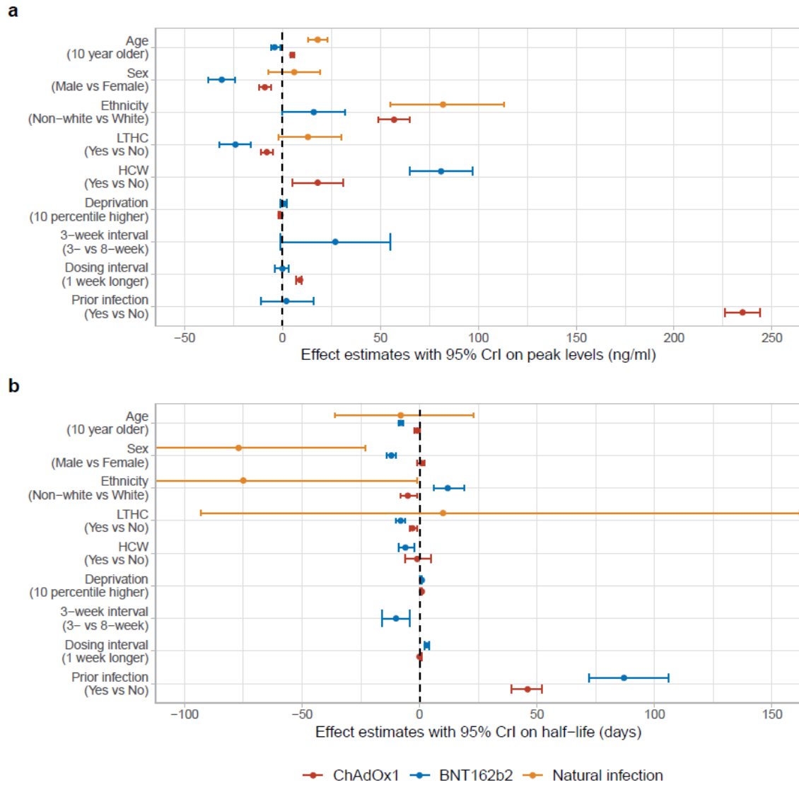
Figure 5. Comparison of effect of factors in participants who received two doses of ChAdOx1 or BNT162b2 or had natural SARS-CoV-2 infection. a , Effect on anti-spike IgG peak levels. b , Effect on anti-spike IgG half-lives. Mean estimates with 95% credible intervals are presented. In panel b, 95% credible intervals are truncated at -100 and 150 days for visualisation.
