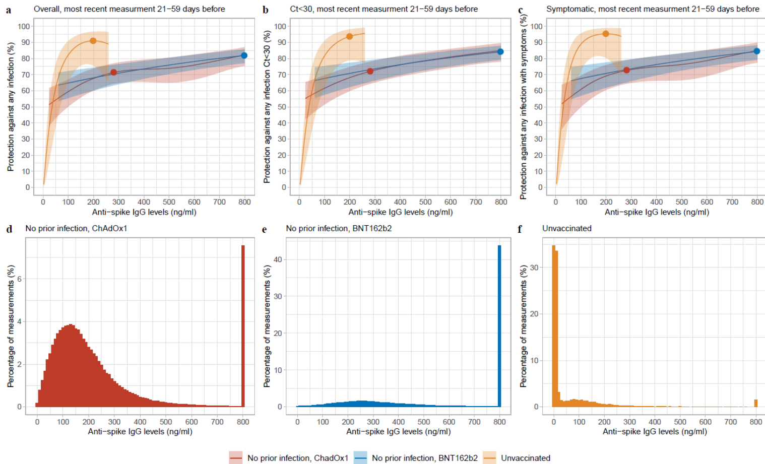
Figure 6. Association between anti-spike IgG levels and protection from SARS-CoV-2 infection using the most recent antibody measurement obtained 21-59 days prior to the current visit. a, protection against any infection; b, protection against infection with a moderate to high viral load (Ct value <30); c, protection against infection with self-reported symptoms. Three groups are investigated, unvaccinated participants with or without evidence of prior infection, participants vaccinated with ChAdOx1 without evidence of prior infection, and participants vaccinated with BNT162b2 without evidence of prior infection. Dots represent the median predicted individual peak levels from the Bayesian linear mixed models: 798 ng/ml for BNT162b2, 281 ng/ml for ChAdOx1, and 199 ng/ml for unvaccinated participants 16 . Distribution of the most recent anti-spike IgG measurements for the three population groups are shown in panel d, e, f.
