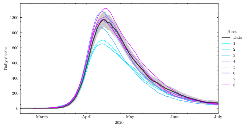
Figure 4. Daily deaths produced by the selected 8 JUNE \beta sets compared to data. The dark shading region corresponds to a 3-sigma error in the data. Both the data and the JUNE curves have been smoothed by averaging over a time period of 7 days.
