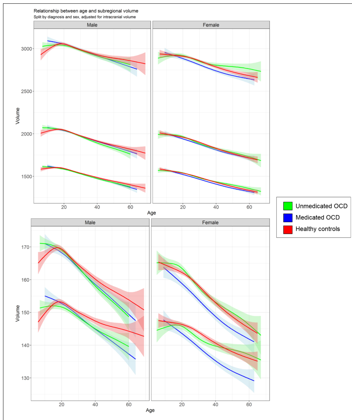
Figure 3: Age trajectory of thalamus subregion volume for medicated obsessive-compulsive patients, unmedicated patients and healthy controls, split by sex and diagnosis
