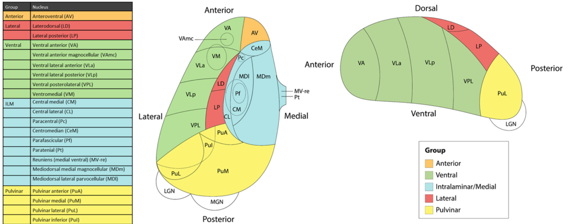
Figure 1: Schematic representation of thalamic nuclei grouping
