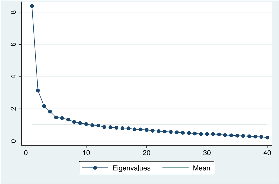
Figure S1 Scree plot showing eigenvalues for the 40 factors
