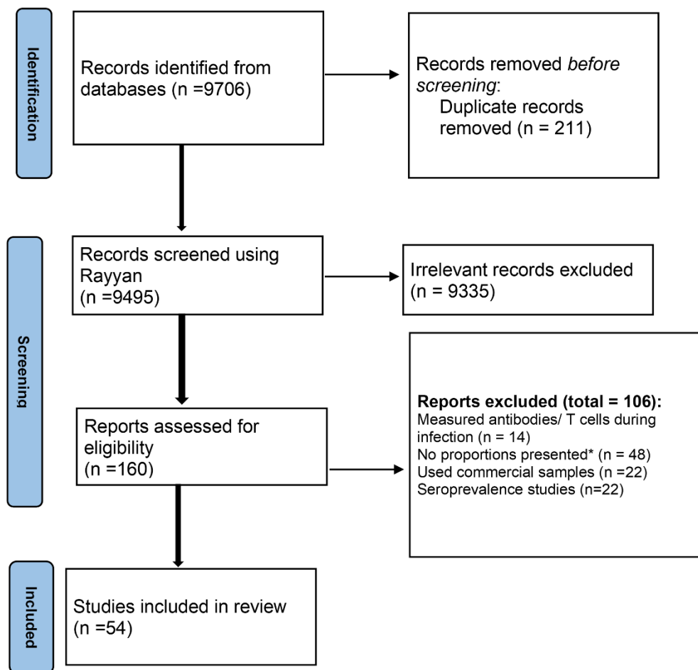
Fig.1 – Flow chart showing the search and inclusion of studies
