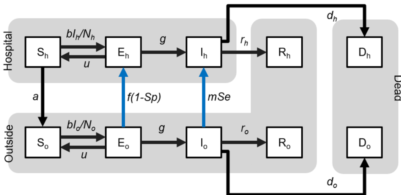
510 Figure 1: Classical SEIRD and testing-SEIRD models
