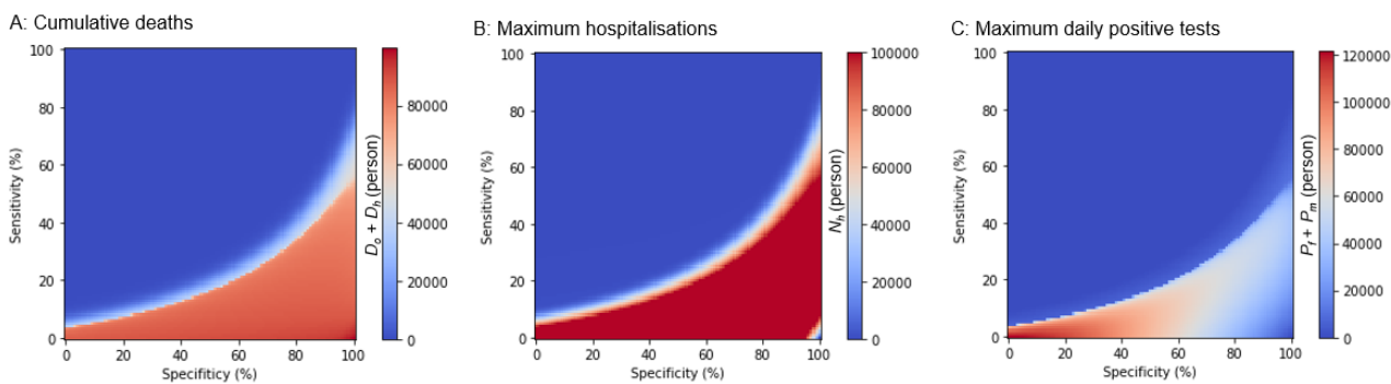
Figure 5: Infectious spread based on the testing properties
