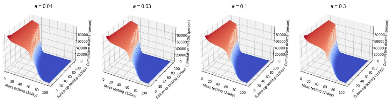
Figure S3: Sensitivity analyses of parameter a on the number of cumulative deaths Simulations were performed with different values of parameter a .
