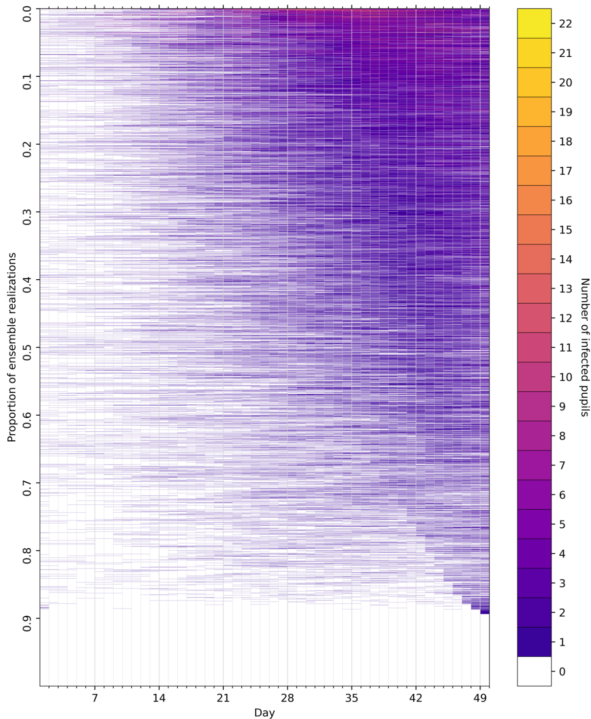
Figure 13. Time series of the number of infected pupils for each realization in an ensemble of 100,000 stochastic simulations of an isolated classroom in Term 1 of 2021 under the rapid-relaxation scenario. Each row of the heatmap corresponds to an ensemble member, with colours denoting the number of pupils in the classroom with Covid-19 infection on each day. The ensemble realizations have been sorted by the sum of the number of infected pupils over all days. Colours denote the number of infected pupils in the classroom for each day of the simulation.
