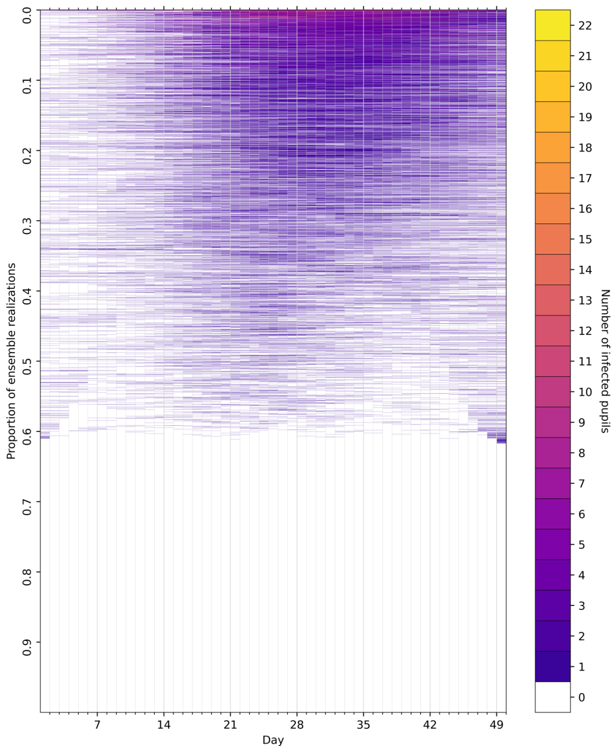
Figure 12. Time series of the number of infected pupils for each realization in an ensemble of 100,000 stochastic simulations of an isolated classroom in Term 1 of 2021 under the gradual-relaxation scenario. Each row of the heatmap corresponds to an ensemble member, with colours denoting the number of pupils in the classroom with Covid-19 infection on each day. The ensemble realizations have been sorted by the sum of the number of infected pupils over all days. Colours denote the number of infected pupils in the classroom for each day of the simulation.
