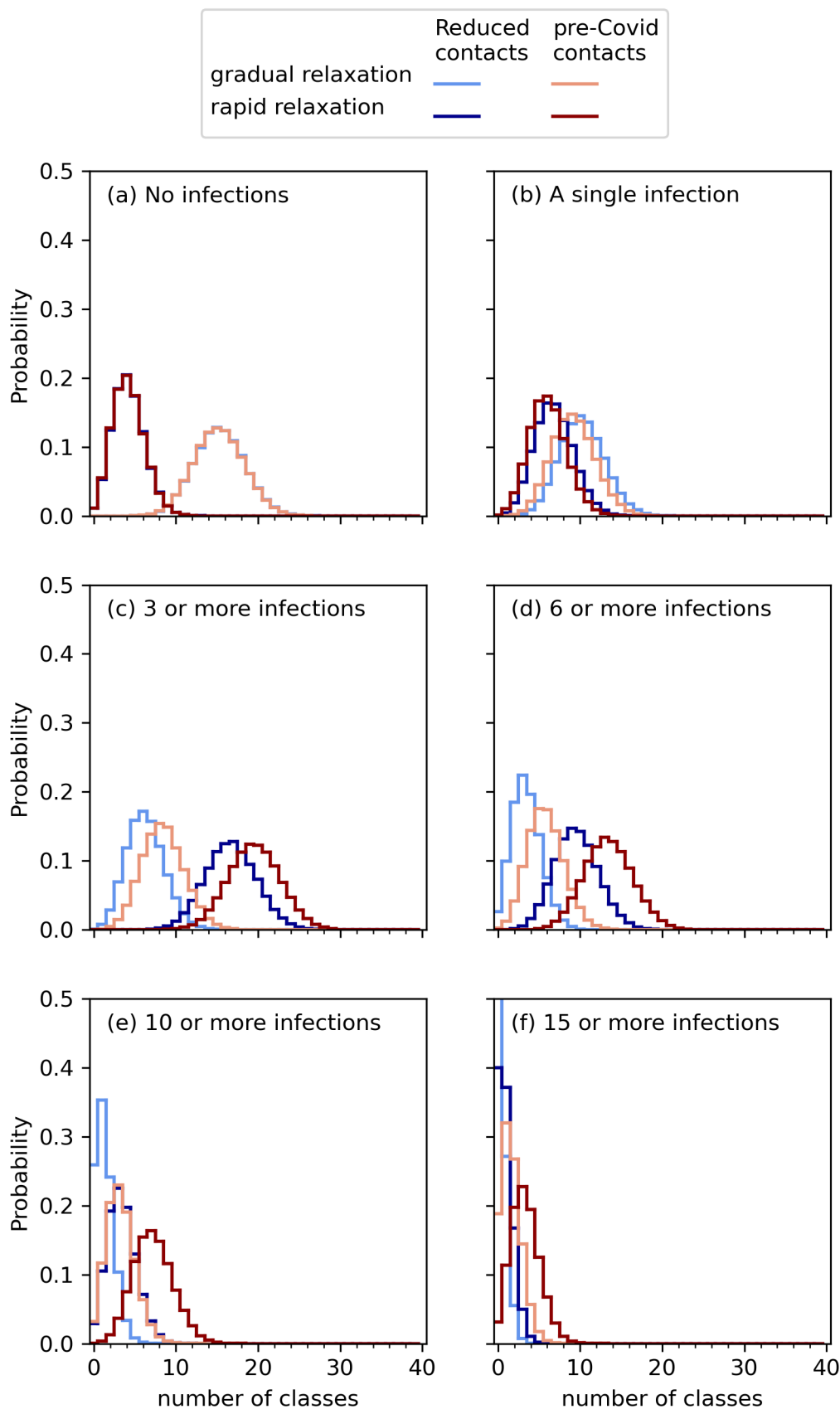
Figure 15. Histograms of the number of classes in a collection of ten schools each with four classes of 30 pupils that are forecast to experience SARS-CoV-2 infections in Term 1 of 2021 under different scenarios: gradual- and rapid-relaxation to pre-Covid societal contacts, and reduced or pre-Covid contact rates in the classroom. Six different infection levels are considered: (a) classes with no infections; (b) classes with a single infection; (c) classes with at least one infection; (d) classes with more than six infections; (e) classes with ten or more infections; and (f) classes with 15 or more infections. Note, in (f) the reduced contacts gradual-relaxation scenario has a probability of no classes with 15 or more infections of 0.66 and is curtailed in these plots to better illustrate the lower probability by high consequence outbreaks
