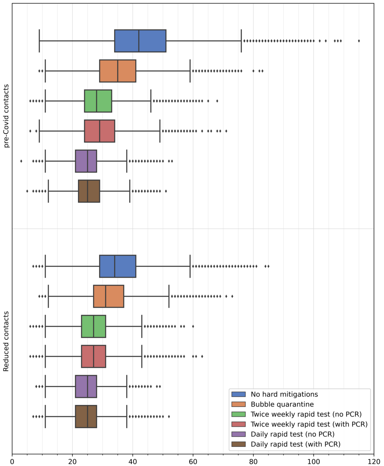
Figure 7. Comparison of the number of infected pupils in 40 primary classrooms with different mitigation measures applied. Box and whisker plots illustrate median, interquartile range, Tukey fences and outliers. Contact rate distributions for pre-Covid times and in small classes are derived from SEJ and used to construct distributions of expected contact rates for schools during Term 1 in September–October 2020. Mitigation measures simulated are: (i) ‘No hard mitigations’ where only individuals who are unwell are quarantined (blue); (ii) ‘Bubble quarantine’ where an unwell individual results in quarantine of the whole class (orange); (iii) ‘Twice weekly rapid test (no PCR)’ where each individual is tested with a rapid lateral flow test twice each week, with positive test results resulting in quarantine of the individual (green); (iv) ‘Twice weekly rapid test (with PCR)’ where each individual is tested with a rapid lateral flow test twice each week, with positive test results resulting in quarantine of the individual and a confirmatory PCR test is applied after a two-day interval (red); (v) ‘Daily rapid test (no PCR)’ where each individual is tested with a rapid lateral flow test daily, with positive test results resulting in quarantine of the individual (purple); (vi) ‘Daily rapid test (with PCR)’ where each individual is tested with a rapid lateral flow test daily, with positive test results resulting in quarantine of the individual and a confirmatory PCR test is applied after a two-day interval (brown).
