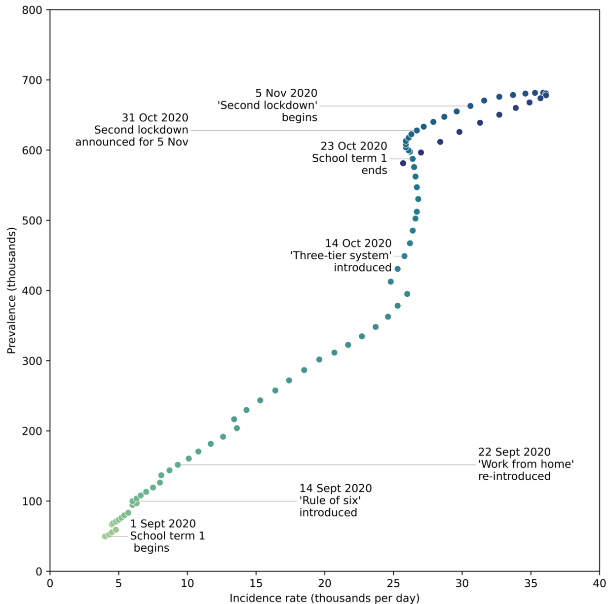
Figure 16. Estimates of the UK SARS-CoV-2 prevalence as a function of incidence rate for 1 September 2020 to 22 November 2020 (date from [24]). The colour of points indicates progression through time. Key dates for changes in social contact rates are indicated. Note, the Alpha variant (B.1.1.7) was first detected in a PCR sample taken in mid-September 2020 and may have been spreading rapidly in this time.
