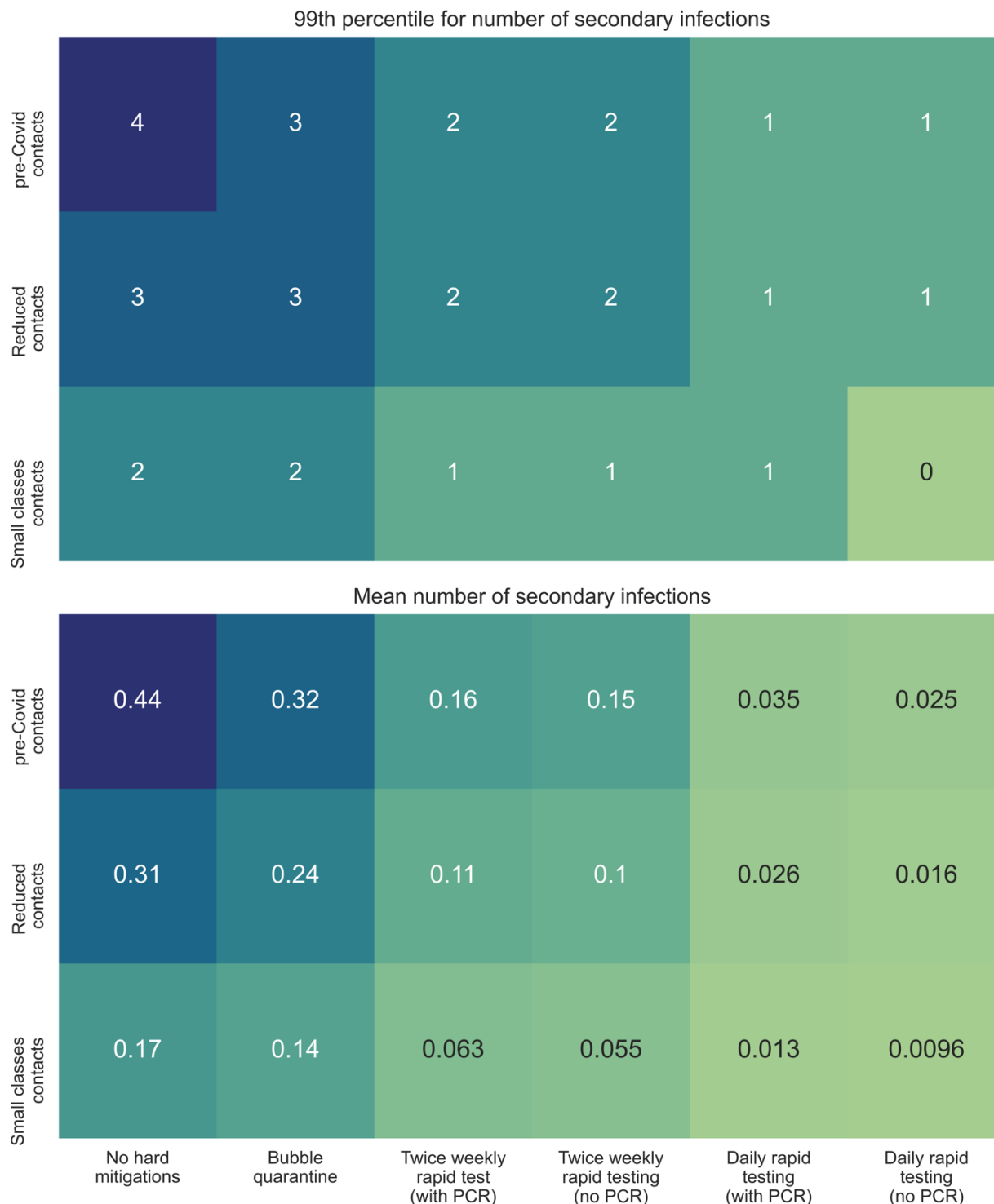
Figure 9. The number of secondary infections in classroom simulations with different contact rates distributions and mitigation measures applied. Two summary statistics to characterize the distributions are shown, with the 99 th percentile value (upper panel) and mean value (lower panel) of the number of secondary infections in all 100,000 ensemble simulations calculated. ‘Small classes contacts’ refers to simulations that adopt contact rate distributions derived from SEJ for small classes that are applied to full classroom attendance. Note, most of infections in the simulations are not transmitted in classroom contacts, so mean values are below 1.0 in all cases
