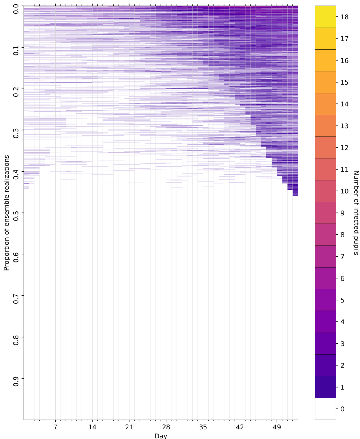
Figure 5. Time series of the number of infected pupils for each realization in an ensemble of 100,000 stochastic simulations of an isolated classroom in Term 1 of 2020. Each row of the heatmap corresponds to an ensemble member, with colours denoting the number of pupils in the classroom with Covid-19 infection on each day. The ensemble realizations have been sorted by the sum of the number of infected pupils over all days. Colours denote the number of infected pupils in the classroom for each day of the simulation.
