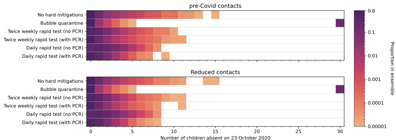
Figure 10. Number of pupils absent from school on 23 October 2020 (the last day of Term 1 in 2020) in an ensemble of 100,000 simulations of a class of 30 pupils. Two contact rates are applied: pre-Covid contact rates (top panel) and reduced contact rates (bottom panel). Six mitigation measures are modelled. Colours indicate the proportion of ensemble realizations on a logarithmic scale (white indicating no occurrence in the ensemble).
