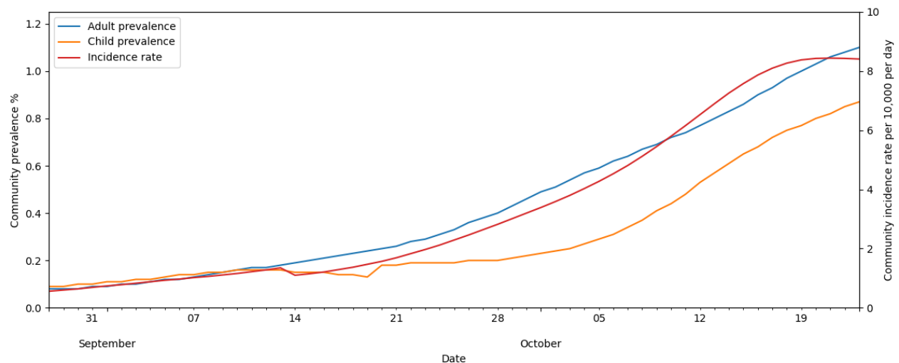
Figure 4. Time series of Covid-19 infection prevalence for adults (blue) and children (orange) and the community incidence rate (red) over Term 1 (Tuesday 1 September to Friday 23 October 2020). Data from Office for National Statistics [24].
