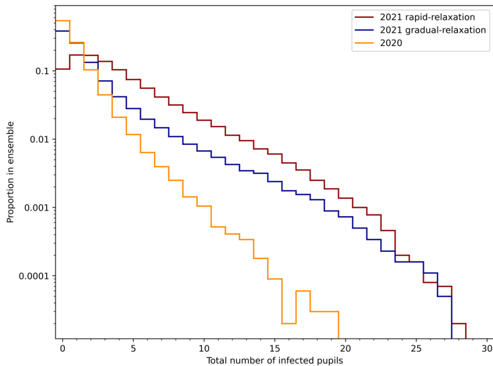
Figure 14. Histograms (empirical pdfs) of the total number of infected pupils in ensembles of 100,000 simulation of the rapid-relaxation and, gradual-relaxation scenarios for Term 1 in 2021 and the ‘no hard mitigations’ simulation with reduced contacts for Term 1 in 2020. Note the logarithmic scale on the proportion in the ensemble.
