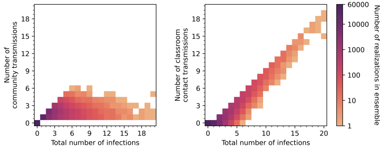
Figure 6. The number of infections caused by community transmissions and classroom contact transmissions in the ensemble simulations as functions of the total number of infections. The intensity of colour of the points indicates the frequency of occurrence within the ensemble on a logarithmic scale. Note, stochastic variations are apparent for low frequencies.
