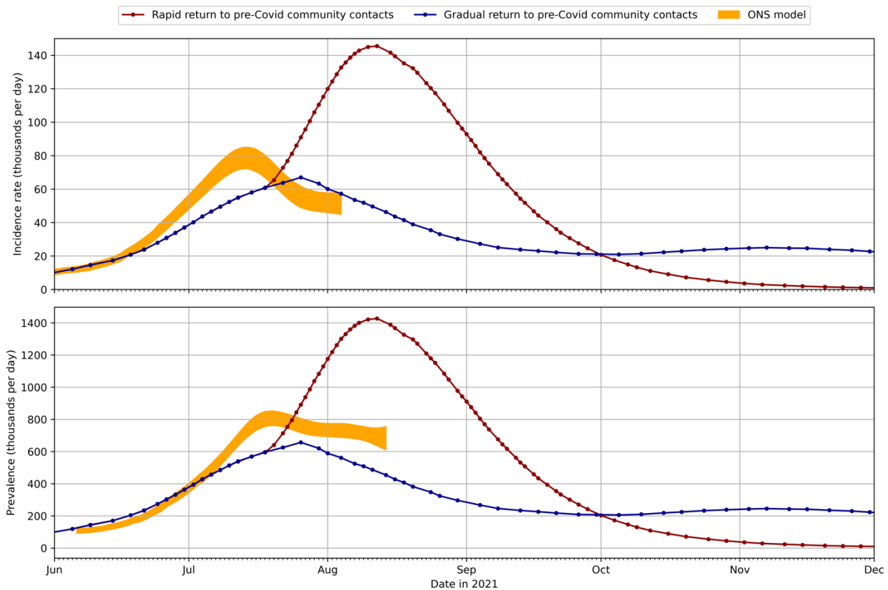
Figure 11. Projections of the incidence rate (upper panel) and prevalence (lower panel) in the UK from June to December 2021. Incidence rates are obtained from a national scale epidemiological model [15] with scenarios modelling a gradual or rapid return to pre-pandemic societal contact rates. The prevalence is modelled assuming R_0 = 5 and infection duration of 40 days (see supplementary material). Data from the Office for National Statistics Coronavirus Infection Survey [24] for the modelled incidence and prevalence with credible intervals are illustrated for the data available at the time of writing.
