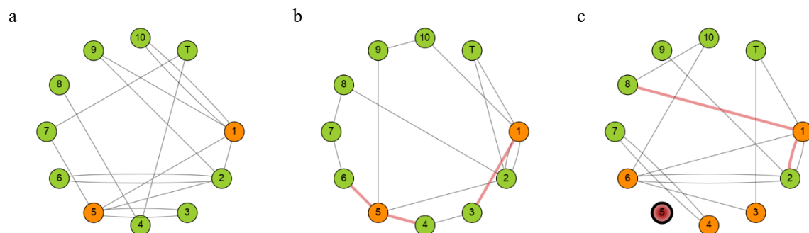
Figure 3. An example of infection transmission within a random updating contact network in a small classroom of ten pupils and one teacher. The degree distribution is fixed, and the edges are determined using the Configuration Model with self-loops removed by random rewiring. Multiple edges are allowed, as illustrated in a where e.g. there are two edges between nodes 1 and 10. The panels represent a progression over three days. Green nodes indicate Susceptible class members, orange nodes indicate Exposed members, and red nodes indicate Unwell individuals. Nodes that are bolded (node 5 in c) are quarantined. Red coloured edges indicate infection transmission between infectious and susceptible members. Note the parameters for infection transmission in this example are not representative of SARS-CoV-2.
