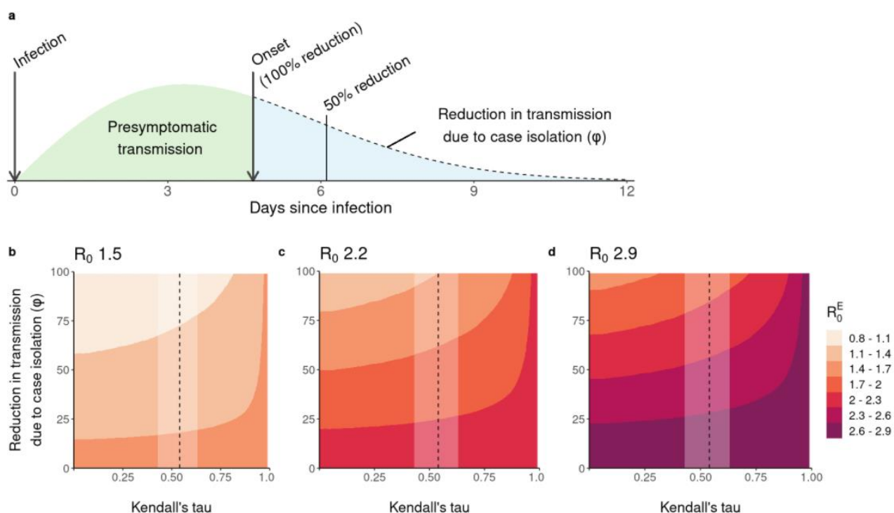
Figure 4 | Effect of stronger correlation between the generation interval and incubation period on effectiveness of isolation. The top figure, a , shows the fitted generation interval probability distribution function (4.22 days). The arrow dividing the green and blue sections indicates onset at 4.67 days (the mean incubation period). If case isolation occurs at onset this is equivalent to a 100% reduction in possible transmission for symptomatic cases. Figures b , c , and d , show the effective basic reproduction number ( R_0^E ) as a function of this reduction in transmission as well as the level of correlation between the generation interval and incubation period. The dashed line is the point estimate of Kendall's tau obtained in this study, while the shaded white rectangle shows its 95% credible interval. We assume baseline R_0 of b , 1.5, c , 2.2, and d , 2.9. As the generation interval and incubation period approach independence (Kendall's tau \rightarrow 1 ) case isolation will become ineffective—shown by the unchanging effective R_0 ( R_0^E )—as transmission will either be presymptomatic or occur nearly at the same time as symptom onset.
