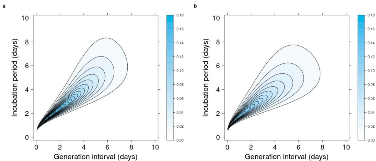
Figure 1 | Joint distribution of the generation interval and incubation period. Contour plots of the fitted distributions. For both a, the dataset of 49 transmission pairs with single dates of reported exposure, and b, the dataset of 257 transmission pairs that also includes pairs with more coarsely reported possible dates of exposure and contact, a Clayton copula with a Weibull marginal for the generation interval and lognormal marginal for the incubation period distribution was selected.
