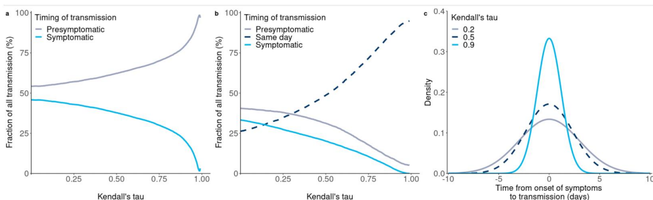
Figure 3 | Increased correlation leads to a predominance of presymptomatic transmission. From estimates made by simulating the generation interval (GI) and incubation period (IP) for 10000 pairs using the fitted Clayton copula with Weibull (GI) and lognormal (IP) marginals: a , the proportion of transmission that was symptomatic or presymptomatic for various values of Kendall's tau; b , the proportion of transmission that was symptomatic, presymptomatic, or occurred on the same day (GI-IP \in [-1, 1] ) for various values of Kendall's tau; c , the time from onset of symptoms to transmission (TOST), defined as GI-IP, fitted with a normal distribution.
