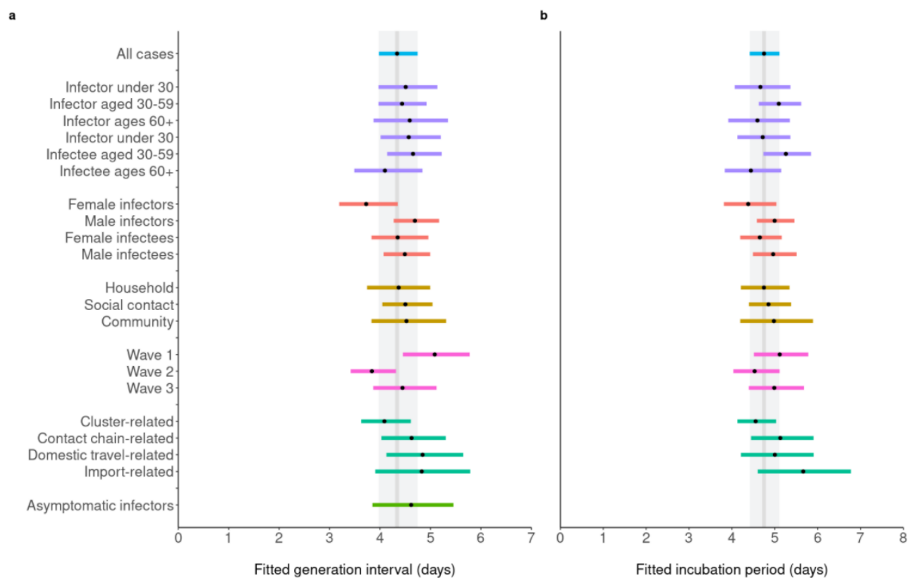
Figure 2 | Joint estimates of the generation interval and incubation period by stratum for COVID-19 transmission pairs from Japan. The joint distribution using best-fit Gaussian, Gumbel, or Clayton copula combined with gamma, lognormal, or Weibull distributions for the a , generation interval and b , incubation period are presented for the dataset of 257 transmission pairs that also includes pairs with more coarsely reported possible dates of exposure and contact. The points are point estimates for the means of each stratum, while the colored bars indicate
