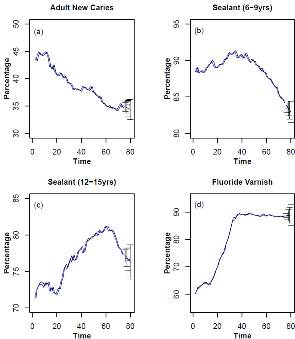
Figure 1 Forecasting DQMs (Adult New Caries, Sealants 6-9 years, Sealants 12-15 years, Fluoride Varnish) is shown in (a-d) respectively. The original monthly time series of the DQMs (blue lines) and the corresponding ARIMA model fit (black lines) along with 5-step ahead forecast and 95% confidence levels (vertical black lines) are also shown in each of the subplots.
