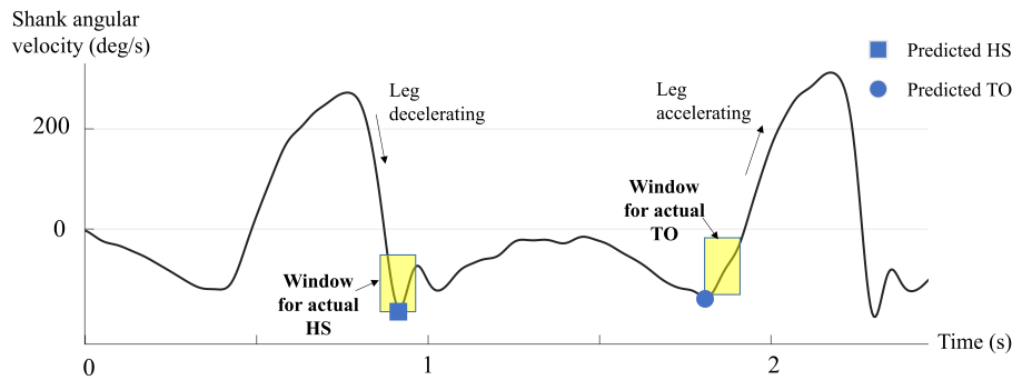
Figure 5: Typical shank velocity graph supplemented with the windows likely to contain the HS and TO events for a gait cycle based on the results of this study.
