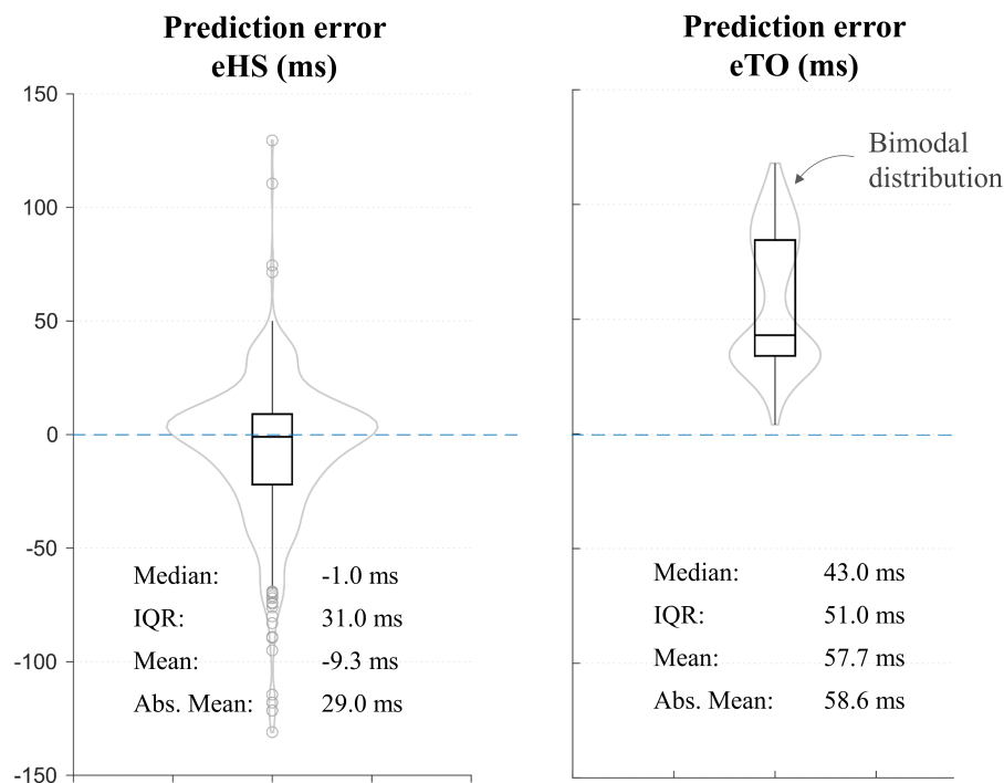
Figure 2: Heel strike (left) and Toe-off (right) error plots for all 2595 walking cycles. Boxplots (black) are superimposed with violin plots (in grey) indicating error distribution. Key statistics are also indicated below each plot. The box indicates the lower and upper quartiles with the central line showing the median. The top and bottom lines of the box represent, respectively, the medians for the upper and lower halves of the data and the whiskers represent the highest and lowest values of the distribution, excluding outliers. Outliers are also presented as circles
