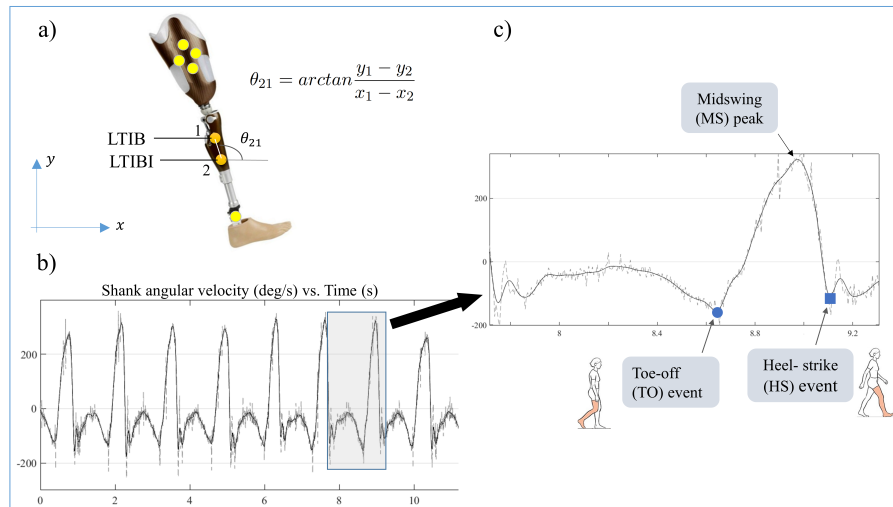
Figure 1: a): Placement of tibia markers for leg orientation and velocity calculation, b) A typical shank velocity signal with raw (grey) and filtered (black) data, c) Enlarged view of one gait cycle from the velocity signal. The algorithm starts with the detection of the largest positive peaks in the signal (marked as MS) which define the intervals for gait events. TO is identified as the last negative peak (or minima) just before the MS (circle) while HS is defined as the negative peak just after the MS (square)
