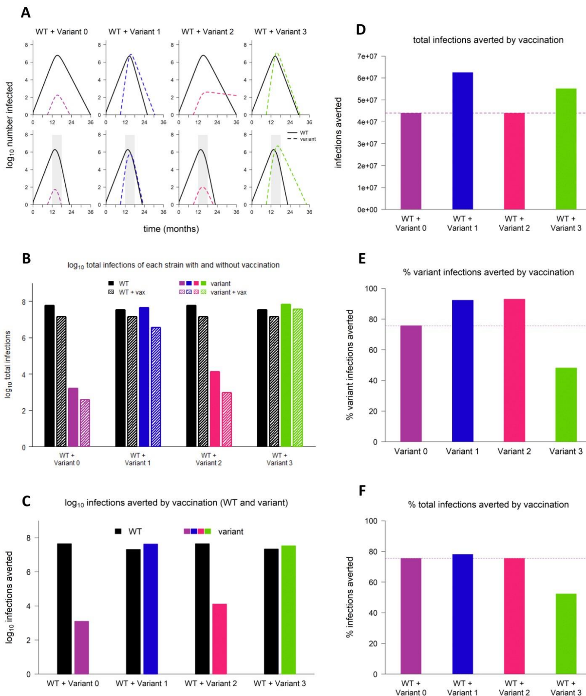
Fig 1. Sample dynamics of hypothetical variants. (A) Dynamics of WT and variant strains without vaccination (top row) and with vaccination (bottom row), shown on log scale. Solid/black lines, WT; dashed/colored lines, variants; gray shading, vaccine rollout. Subsequent panels reference the simulations depicted in (A). (B) Total infections with WT and variant strains with and without vaccination (log scale). Black bars, WT; colored bars, variants; solid bars, without vaccination; hatched bars, with vaccination. (C) WT and variant infections averted by vaccination (log scale). Black bars, WT; colored bars, variants. (D) Total infections (WT + variant) averted by vaccination (linear
