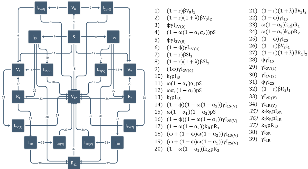
Fig 7. Diagram and rates of movement between compartments for alternative model with all-or-nothing immunity.
