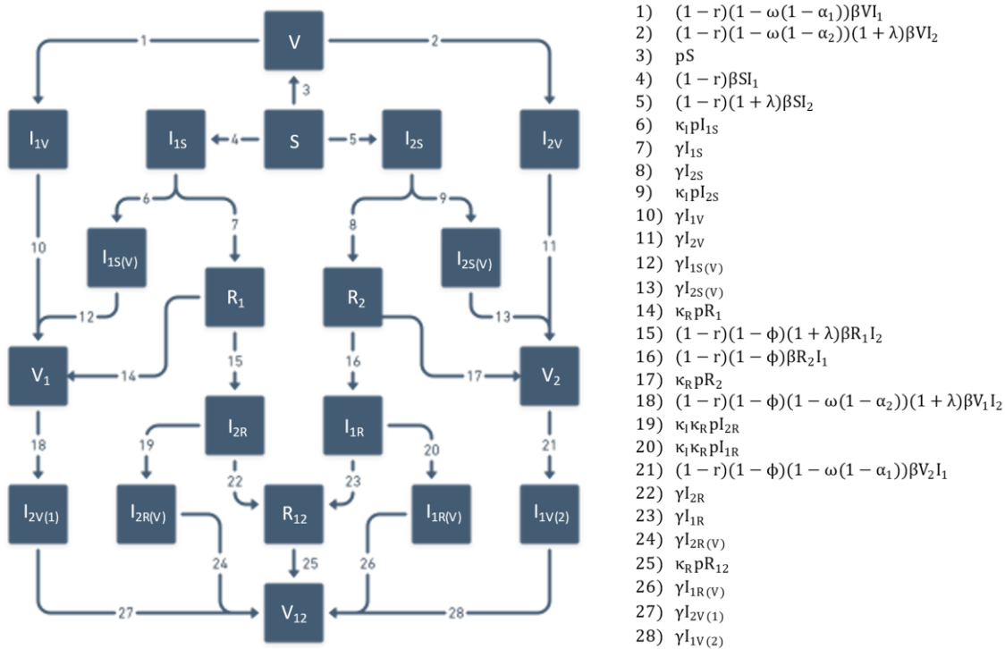
Fig 6. Model diagram and rates of movement between compartments, corresponding to labeled arrows.
