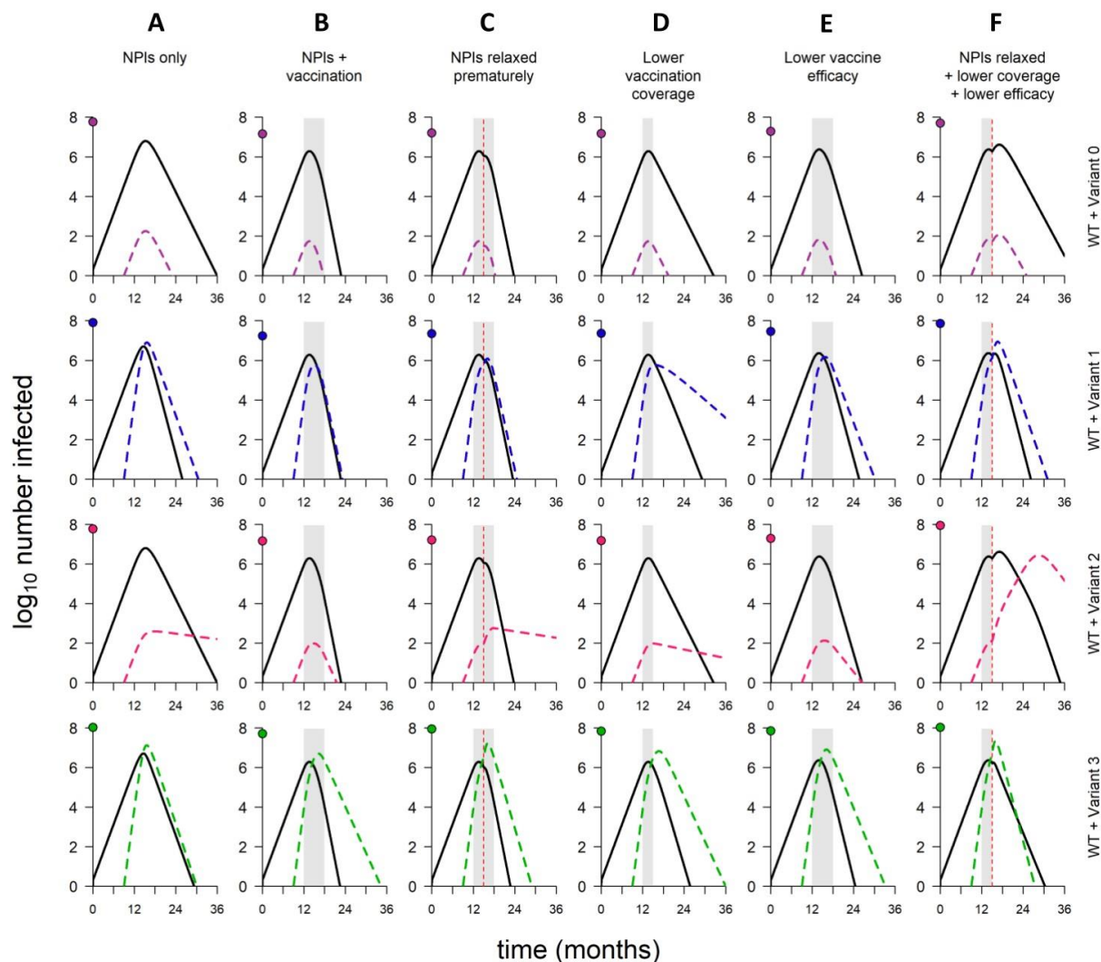
Fig 5. Dynamics of WT and variants in simulations with varying combinations of control measures. (A) No vaccination but NPIs in place throughout. (B) Default model conditions (NPIs in place throughout, 100% vaccination coverage, 95% vaccine efficacy against WT). (C) NPIs lifted when vaccination coverage reaches 50% (other model conditions as in B). (D) 50% vaccination coverage (other model conditions as in B). (E) 70% vaccine efficacy (other model conditions as in B). (F) Combination of conditions C through E (NPIs relaxed, 50% vaccination coverage, and 70% vaccine efficacy). In each panel, point on y-axis indicates the total number of infections over the entire
