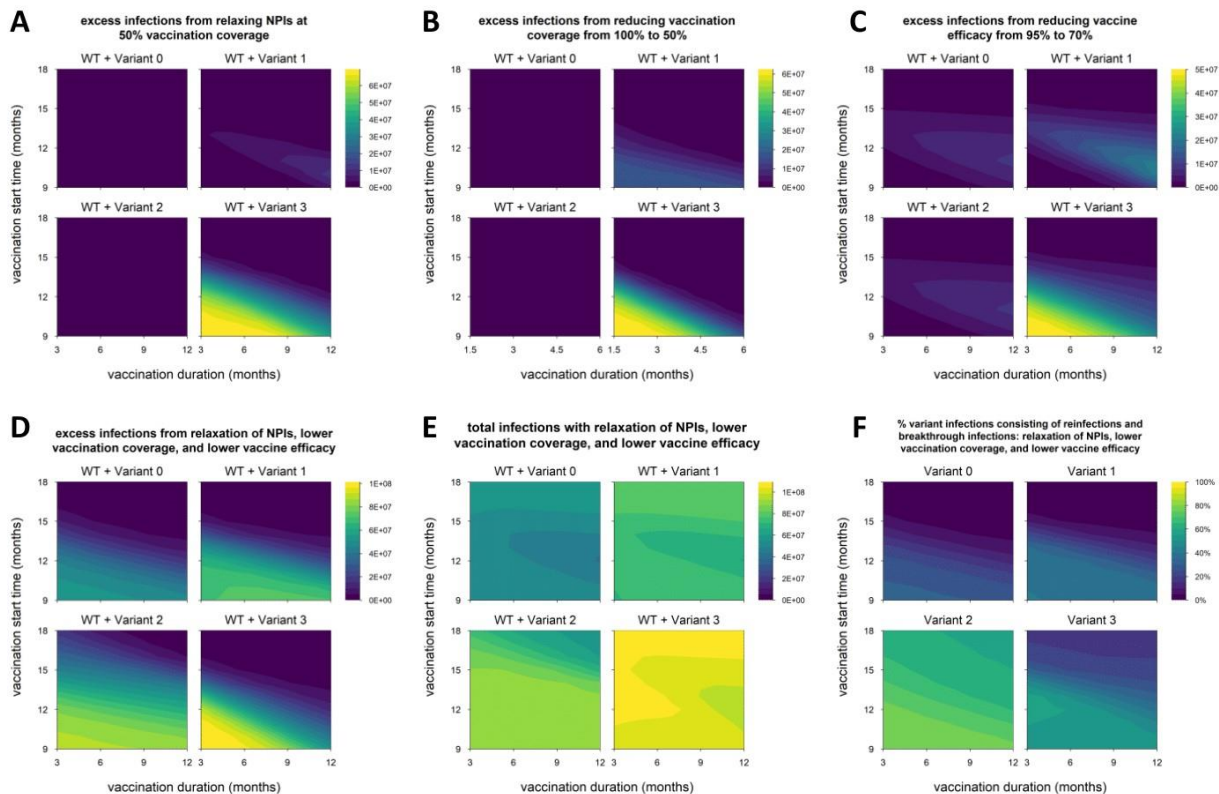
Fig 4. Impact of reduced control measures on epidemic size. (A) Excess infections from lifting nonpharmaceutical interventions (NPIs) when vaccination coverage reaches 50% (default condition is NPIs continued indefinitely); shading represents excess infections compared to default conditions/parameters. (B) Excess infections from reducing vaccination coverage from 100% to 50%. (C) Excess infections from reducing baseline vaccine efficacy (against WT) from 95% to 70%. (D) Excess infections from the combination of conditions A through C (lifting NPIs, reduced coverage and reduced efficacy). (E) Total infections (WT + variant) under the combined conditions of panels A through C; shading represent total infections. (F) Percentage of variant infections composed of reinfections and breakthrough infections under the combined conditions of panels A through C; shading represent percentage of variant infections occurring in recovered/vaccinated individuals. Variant introduced at 9 months in all simulations. Variant phenotypes are as follows: variant 0, identical to WT; variant 1, 60% greater transmissibility; variant 2, 40% immune escape; variant 3, 60% greater transmissibility and 40% immune escape.
