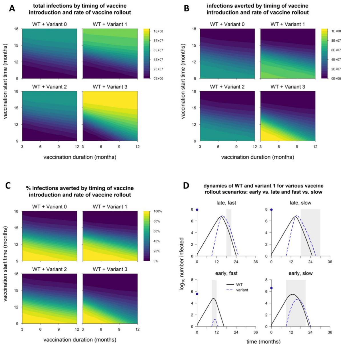
Fig 2. Epidemic size and vaccination impact vary with the time of vaccine introduction and rate of vaccine rollout. (A) Total infections (WT + variant) in simulations with each hypothetical variant, for varying rates of vaccination (vaccination duration, x-axis) and time of vaccine introduction (vaccination start time, y-axis); shaded contours represent total infections. (B) Number of infections (WT + variant) averted by vaccination; shading represents number of infections averted. (C) Percentage of infections (WT + variant) averted by vaccination; shading represents % infections averted. Variant introduced at 9 months in all simulations. (D) Dynamics of WT and variant 1 in simulations with the minimum and maximum values for vaccination duration (fast = 3 months, slow = 12
