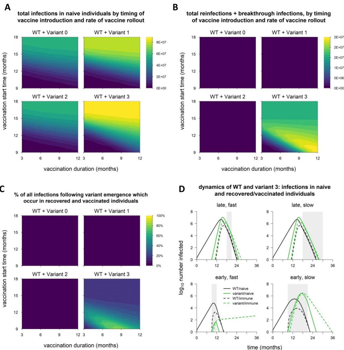
Fig 3. Breakdown of infections by immune status (naïve vs. recovered/vaccinated). (A) Total infections in naïve individuals, in simulations with each variant, for varying rates of vaccination (x-axis) and time of vaccine introduction (y-axis); shaded contours represent total infections. (B) Total infections in recovered and vaccinated
