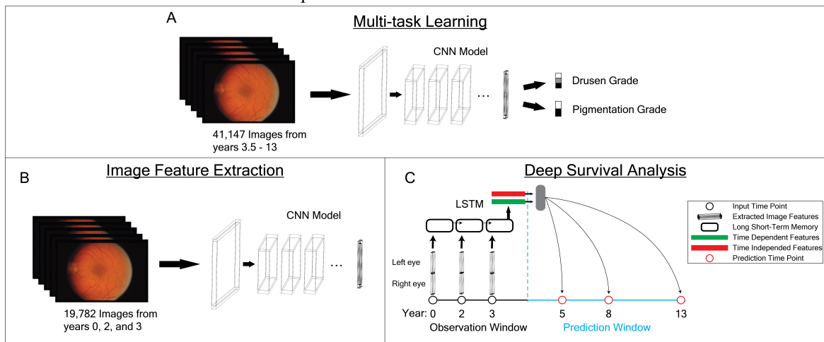
Figure 1: Model Architecture.
