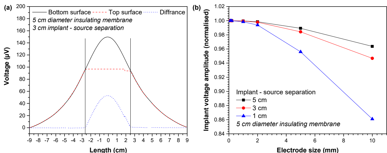
Figure 7: (a) Impact of electrode diameter. Voltage along two surfaces of the implant. Bottom surface is facing the dipole signal source while the top surface is facing the scalp. (b) Variation in the differential recording with different electrode sizes.
