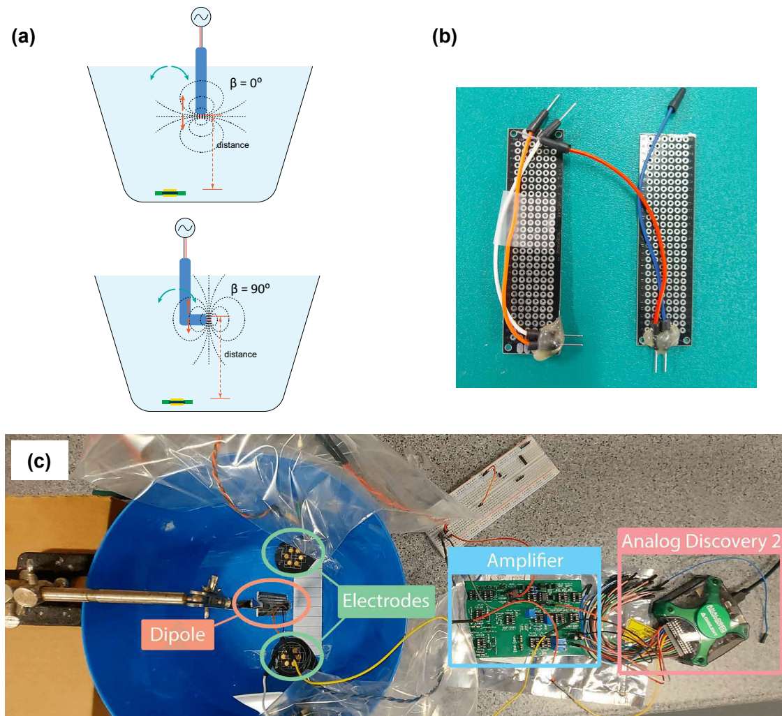
Figure 3: Experiment with a phantom. (a) Saline solution was used as a phantom model. The device with the top and bottom electrodes was placed at a 3 mm distance with the bottom of the tank. (b) The dipole electrodes were positioned 2.5 mm apart. The dipole configuration produces an electric field tangential or perpendicular to the surface of the electrodes. (c) It shows the setup and recording readout circuitry. Note that only a small part of the large amplifier board is used to host our low-noise amplifier components in this experiment
