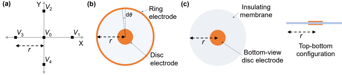
Figure 6: (a) Approximation of the Laplacian at the point v_0 on a regular square grid plane using the five-point method (FPM). (b) A bipolar electrode configuration approximation of the FPM with a concentric disc and ring electrodes. (c) Bottom- and side-view of our proposed electrode architecture.
