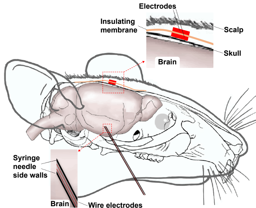
Figure 4: Electrical measurements with sensors implanted in a mouse cadaver. The subcutaneous implant consisted of two 2\text{ mm} \times 2\text{ mm} electrodes fabricated using 12\text{ }\mu\text{m} thick brass sheets. They were attached at the center of a 12\text{ }\mu\text{m} thick sheet of polyimide with a dimension of 2\text{ cm} \times 2\text{ cm} using epoxy resin. The dipole signal source was constructed with a pair of enameled coated copper wires (diameter of 0.3\text{ mm} ) inserted into a 20-gauge needle (internal diameter of 0.91\text{ mm} ). The dipole signal had an amplitude of 20\text{ mV} and a frequency range of 1.3\text{ Hz} to 1\text{ kHz} .
