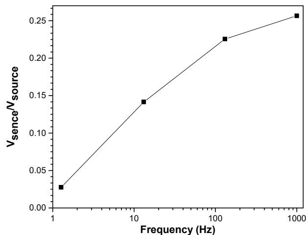
Figure 9: Recorded signal measurements across a frequency range of 1.3 Hz to 1 kHz from the mouse cadaver experiment.
