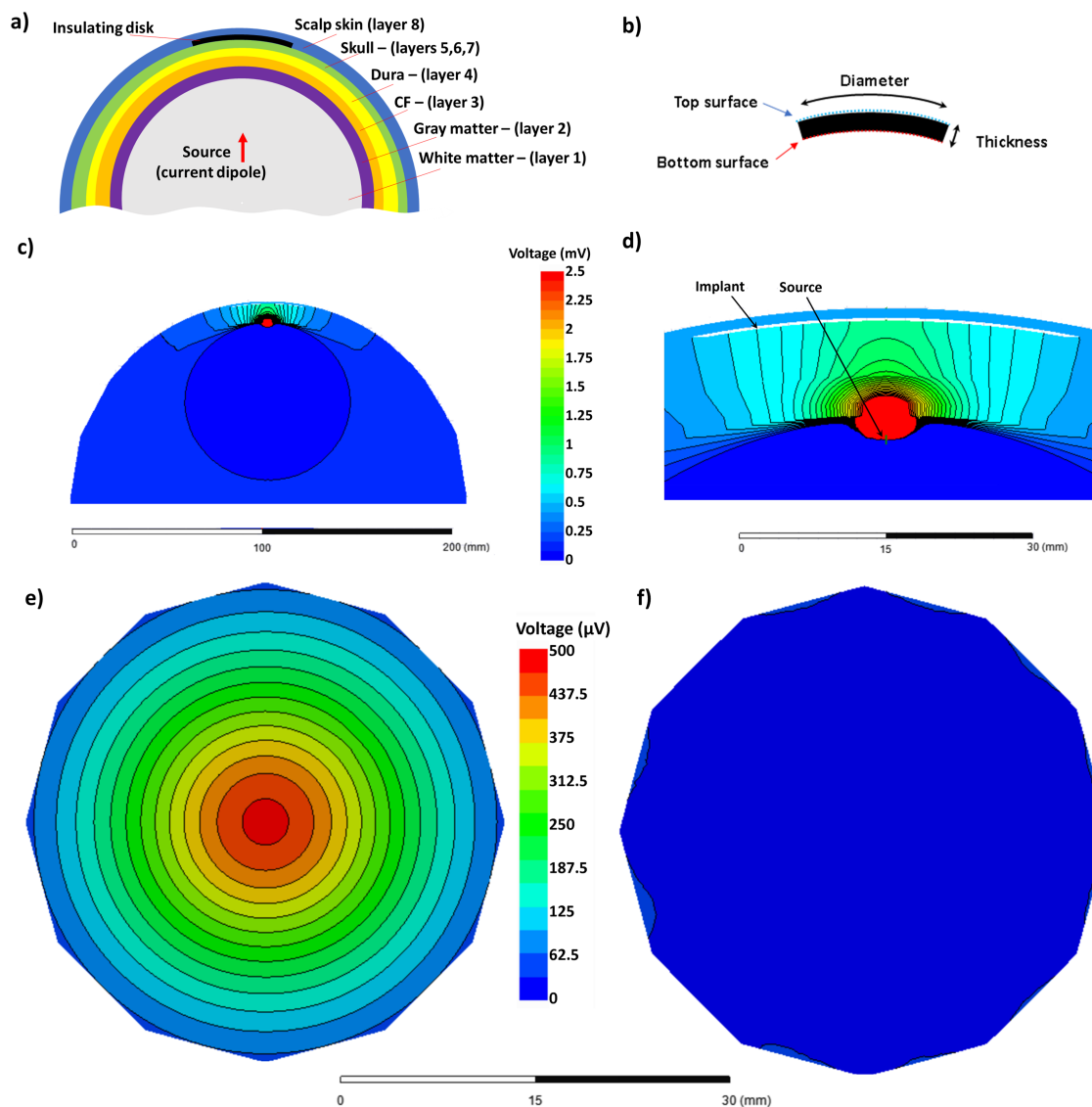
Figure 2: (a) Electrostatic finite element modeling setup showing the eight layers used in the model as well as the relative placement of the source (current dipole) and the insulating disk (implant model). (b) The insulating membrane's cross-section is showing the top and bottom surfaces used to extract the differential voltage values. (c) A typical finite element method (FEM) simulation result highlighting the voltage variation. (d) Zoomed-in version of (c) highlighting the location of the implant and signal source. (e) and (f) voltage variation over the bottom and top surfaces of the insulating membrane. Throughout the FEM analyses, the voltage at the center of the insulating membrane, over a diameter of 0.1 mm, is used in the calculations.
