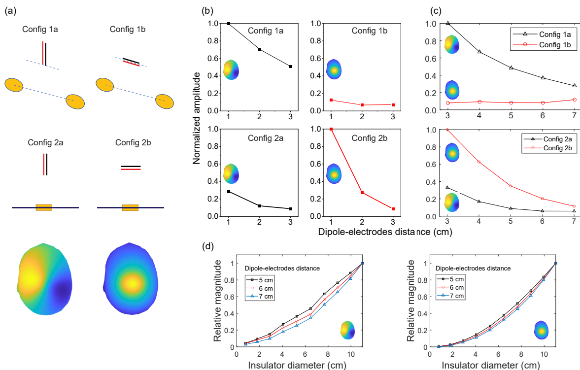
Figure 5: Comparison between side-by-side (configurations 1a and 1b) and top-bottom (configurations 2a and 2b) placements of electrodes in terms of recorded signals. (a) Dipole electrodes setups. Config 1a: tangential dipole is placed on top of the centerline of the electrodes. Config 1b: radial dipole is placed on top of the centerline of the electrodes. Config 2a: tangential dipole with top-bottom placement. Config 2b: radial dipole with top-bottom placement. (b) Measurements of recorded signals from the phantom experiment. Signals are normalized by dividing with the max amplitude per each electrode placement (side-by-side or top-bottom. (c) Matlab simulation results of recorded signals. Similarly, values are normalized by dividing with the max value per each placement. (d) Matlab simulation of the impact of the insulating membrane diameter to recorded signals when the dipole is tangential (left) and radial (right).
