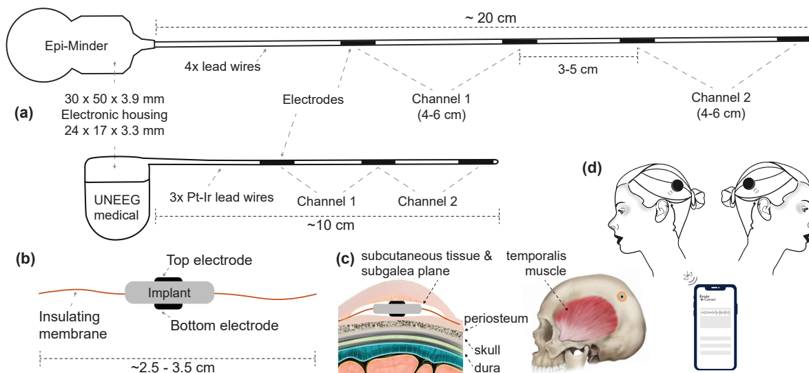
Figure 1: Current solutions for subscalp and subcutaneous EEG and our proposed solution. (a) Illustrates two examples of subscalp and subcutaneous technologies. Epi-Minder bilateral subscalp EEG device with four lead wires, with the longest being more than 20 cm. The Epi-Minder’s implantable body is comprised of four electrodes positioned along a length of the implantable body and using a cochlear implant system housing. Note that the channel arrangements may be different from one that is shown here. The leading solution from UNEEG medical’s unilateral SubQ device with two channels, a hearing-aid electronic housing, and three electrodes. Here we only show the implantable parts [7]. We estimate the Minder’s and SubQ’s implant volumes at \sim 6,000 \mu\text{l} (with \sim 96\% rigid parts) and \sim 1,500 \mu\text{l} (with \sim 92\% rigid parts), respectively. (b) Shows a simplified illustration of our proposed solution with novel electrode architecture. The two electrodes are placed on the top and bottom of the implant body, where electronic housing is. The insulating membrane, such as medical-grade silicone, extends around the rigid core of the implant’s body. The insulating membrane helps to achieve a few cm sensing distance with sub-mm physical distance between the two electrodes. We estimate the total implant volume to be \sim 1,000 \mu\text{l} (with \sim 32\% rigid parts), with an outer insulating membrane to be flexible and foldable when necessary. (c) Shows how the implant body subgaleal and possible positioning of the device on a human head. (d) Illustrates the external units. One of each side and uniquely tagged for communication.
