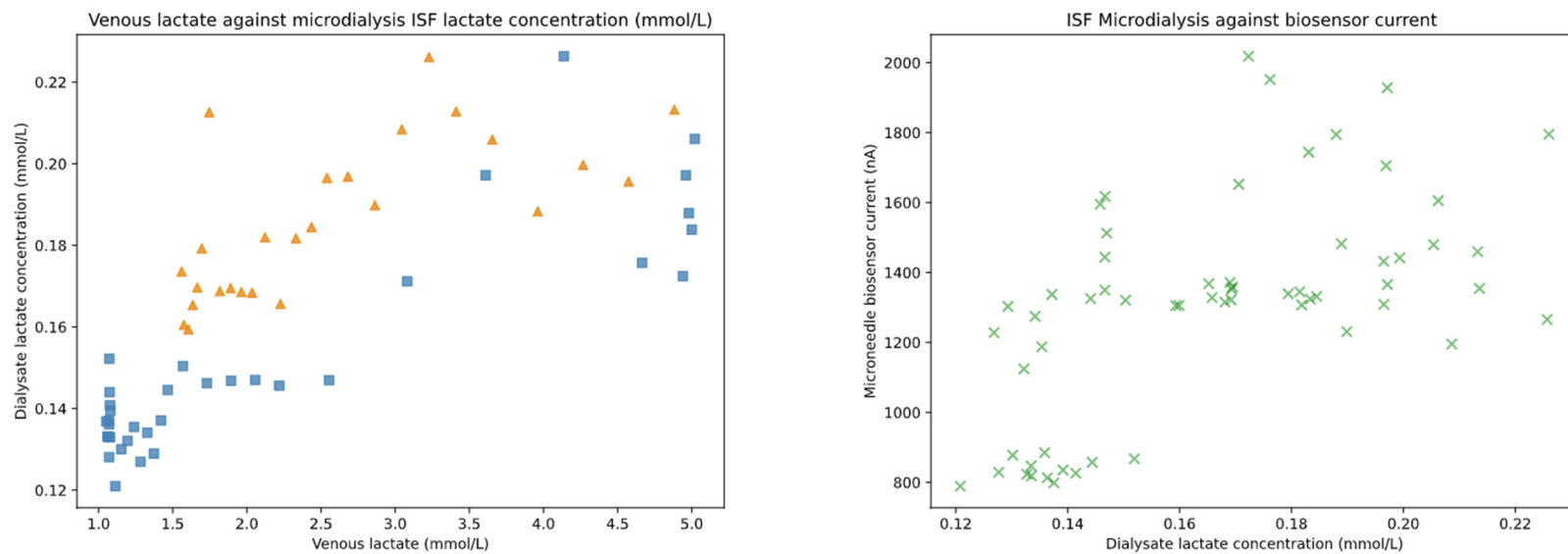
Figure 3 – Left: Venous lactate plotted against dialysate lactate concentrations from microdialysis. Blue squares represent the exercise phase and the orange triangles represent the rest phase of the study. Right: Green crosses represent dialysate lactate concentrations against microneedle biosensor current downsampled to 1-minute intervals.
