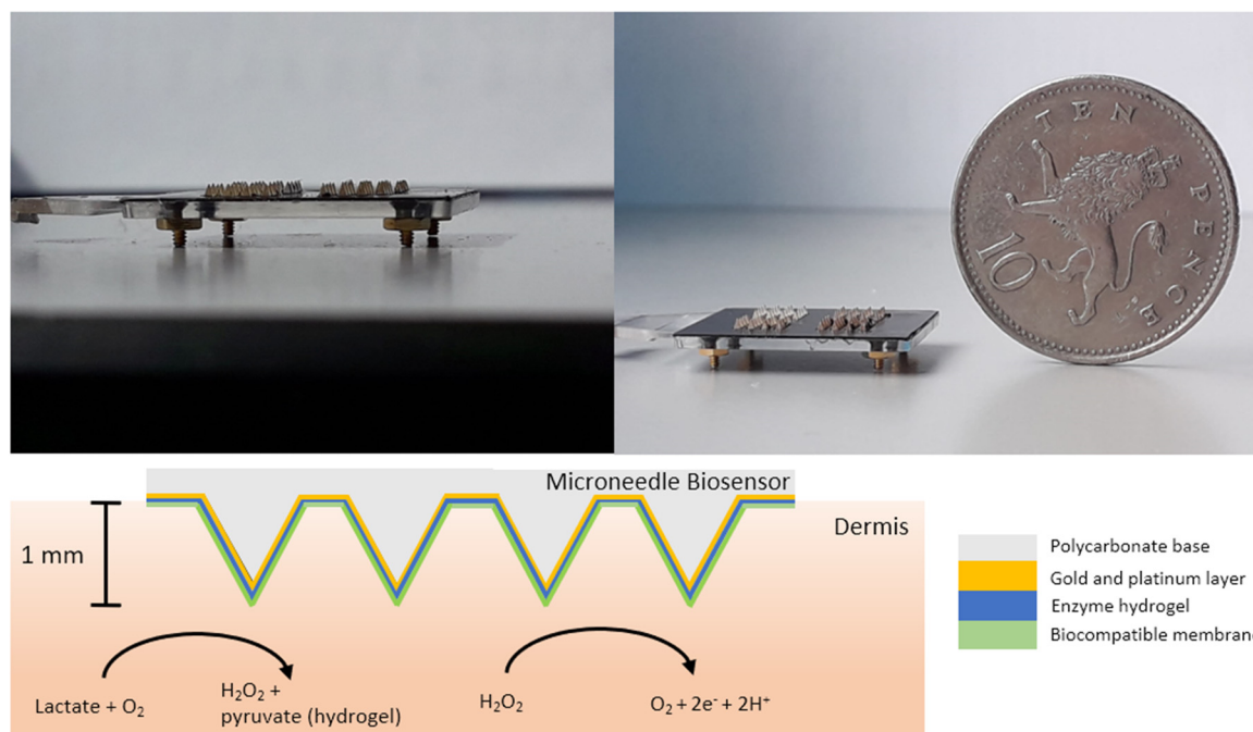
Figure 1 – Top left and right: the microneedle biosensor measures less than 2 \times 2 cm and consists of small 1 mm protrusions which penetrate the stratum corneum in the epidermis to come into direct contact with tissue interstitial fluid. Bottom: lactate in the interstitial fluid is converted to pyruvate and hydrogen peroxide, with the latter being oxidised at the biosensor electrode surface, which is held at +0.7 V vs Ag|AgCl reference electrode. The resulting current is proportional to ISF lactate concentration.
