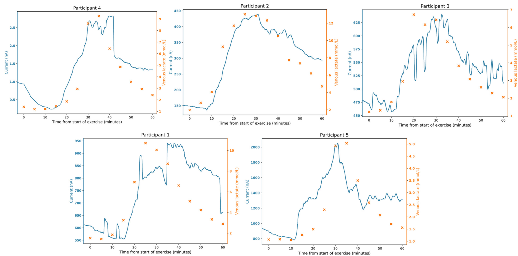
Figure 2 – Microneedle biosensor current (blue continuous), venous lactate sampling (orange crosses) against time for individual participants (n=5). Exercise commenced at 0 minutes and stopped at 30 minutes, followed by a rest phase until the end of the study at 60 minutes.
