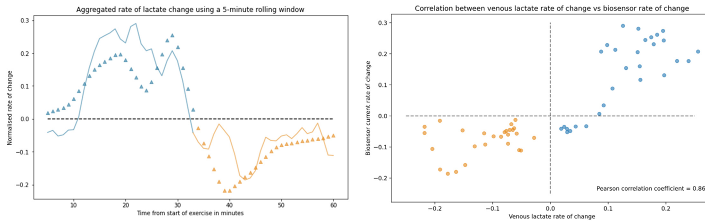
Figure 5 - Left: normalised rate of change for all participants using a rolling window against time. The continuous line shows rate of change for the biosensor and triangles show venous lactate change at 1-minute intervals. The blue plots represent exercise phase and orange represents rest phase. The mean lactate peak occurred after 32 minutes after start of exercise. Right: Correlation scatterplot showing correlation between two measurements with a r of 0.86.
