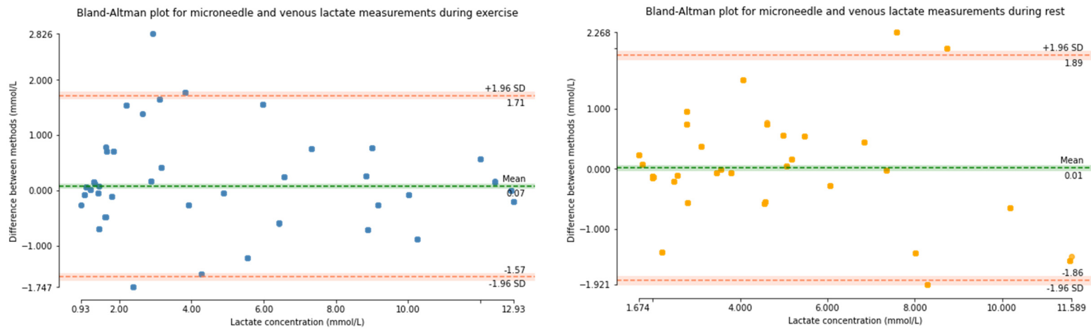
Figure 4 – Bland-Altman plots of agreement between biosensor and venous blood lactate aggregated for all 5 participants. Analyses were separated by phase of the study between exercise and rest. The left plot shows data obtained during exercise (0-30 minutes), and the right plot shows data during rest (30-60 minutes). The horizontal axes show the range of lactate observed in the study and vertical axes difference in agreement between measurements. The 95% confidence interval (+/- 1.96 of standard deviation) is shown in orange horizontal lines.
