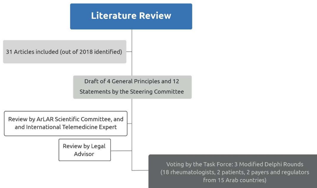
FIGURE 2 STUDY FLOWCHART
