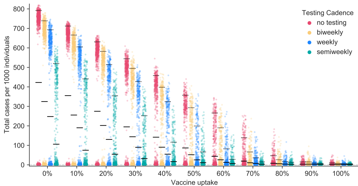
Figure C1: Outbreak sizes when vaccine effectiveness is 70% Here we illustrate the outcome of 1000 simulations for each combination of testing cadence and vaccination uptake, when 10% of the population have previously been infected, vaccines are on average 70% effective at preventing infection and transmission, and R_0 = 4.0 . Solid black lines mark the mean outbreak sizes and dashed black lines mark the 95th percentile outbreak sizes for each parameter combination.
