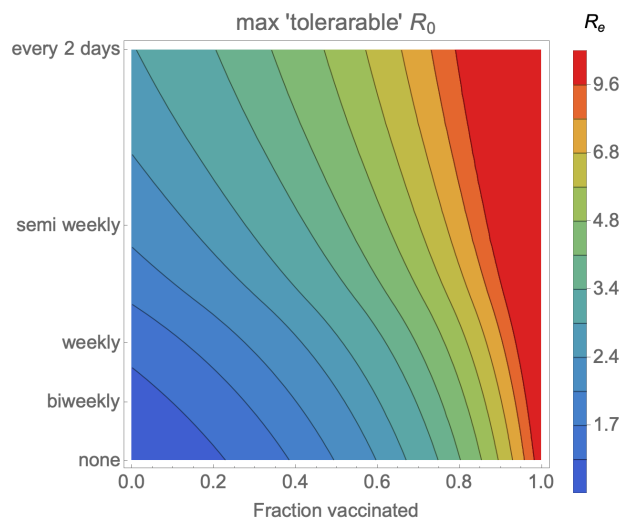
Figure 3: Maximum controllable R_0 depends on vaccination and testing rates. Contour plot illustrates the highest R_0 for which R_e can be brought down below 1.0 by means of the specified combination of vaccination coverage (horizontal axis) and testing cadence (vertical axis). Here 10% of the population has been previously infected and vaccines average 90% effectiveness.
