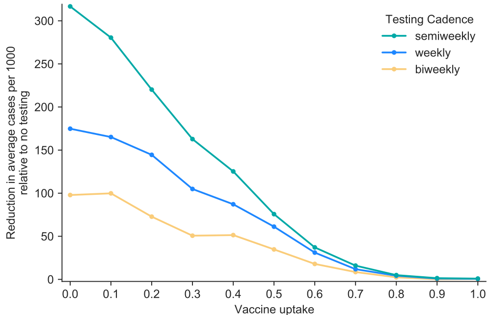
Figure C2: Value of testing when vaccine effectiveness is 70%. Here we show how many cases per 1000 individuals are prevented on average when using a given testing cadence relative to not testing, where R_0 = 4.0 , 10% of the population have previously been infected, and vaccines are on average 70% effective at preventing infection and transmission. As vaccination uptake increases, the benefits of testing here, with 70% effectiveness, decline less rapidly than the benefits with 90% effectiveness as shown in Figure 5. Differences between the values for 0% vaccine uptake here and those in Figure 5 are merely stochastic.
