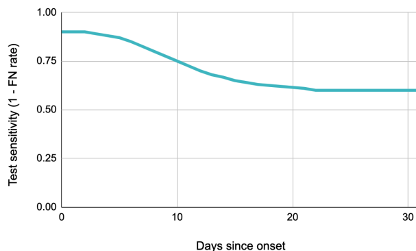
Figure B1: Test sensitivity in the SEIRS+ model. The probability of returning a positive test results when testing an infected, symptomatic individual as a function of the number of days since entering that state. The test sensitivity is equivalent to 1 minus the false negative rate.
