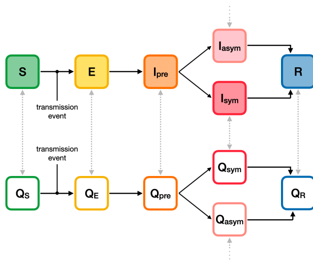
Figure 1: The SEIRS+ model extends the structure of a basic SEIR compartment model. In addition to the traditional S , E , and R states, the I state is split into three separate compartments: presymptomatic I_{pre} , asymptomatic I_{asym} , and symptomatic I_{sym} . In addition, each primary compartment (shaded) has a parallel compartment Q (unshaded) representing individuals at the same disease stage but in quarantine.
