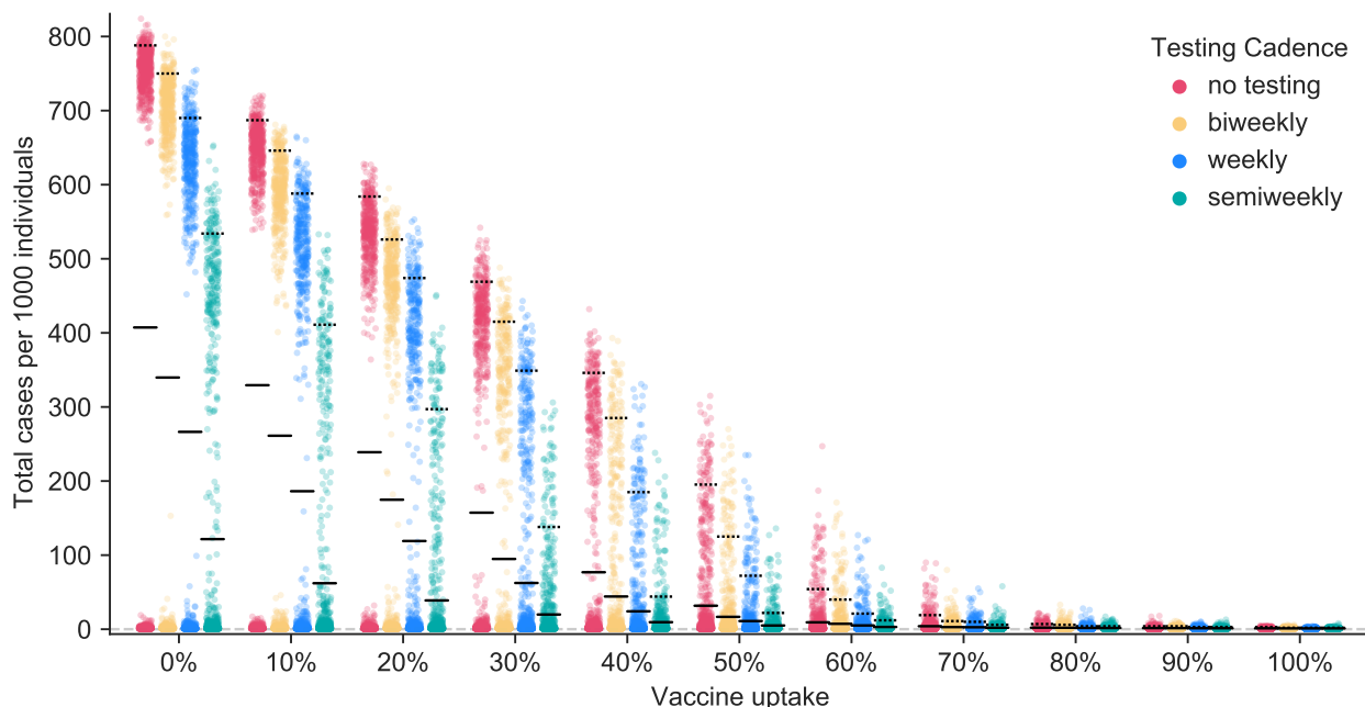
Figure 4: Outbreak sizes in the stochastic network simulation model. Here we illustrate the outcome of 1,000 simulations for each combination of testing cadence and vaccination uptake, when 10% of the population have previously been infected, vaccines are on average 90% effective at preventing infection and transmission, and R_0 = 4.0 . Each colored dot represents the outcome of a single simulation run. Solid black lines mark the mean outbreak sizes and dashed black lines mark the 95th percentile outbreak sizes for each parameter combination.
