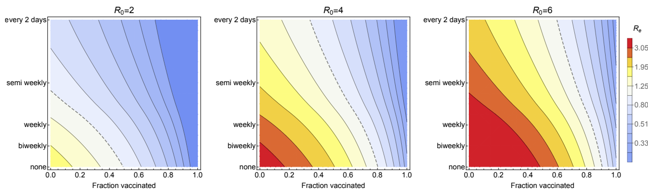
Figure 2: Effects of NPIs, vaccination, and testing. Contour plots of the effective reproduction number R_e show how mitigation efforts depend on NPIs via their effects on R_e , on vaccination coverage (horizontal axis), and on testing cadence (vertical axis). The dashed line in each panel shows the combinations of vaccination and testing that are sufficient to drop R_e to unity for a given R_0 value. (a) When R_0 = 2.0 , as we might expect for less transmissible variants with active NPIs, the effective reproduction number can be brought below unity with semi-weekly testing, by vaccinating half of the population, or some combination of those interventions. (b) With more transmissible variants and NPIs relaxed so that R_0 rises to 4.0, broad vaccination coverage is an essential component to any control strategy and testing can help get down below the R_e = 1 threshold when vaccinate rates are in the range of 50-80%. (c) With highly transmissible variants and minimal NPIs, reducing R_e below one is impossible without very high levels of vaccination. In all three panels, we illustrate a situation in which 10% of the population has been previously infected and vaccines average 90% effectiveness. Additional parameters are summarized in Table B.2.
