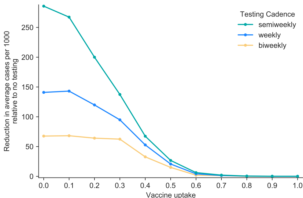
Figure 5: Value of testing in the stochastic network simulation model , as more of the population becomes vaccinated. Here we show how many cases per 1000 individuals are prevented on average when using a given testing cadence relative to not testing, where R_0 = 4.0 , 10% of the population have previously been infected, and vaccines are on average 90% effective at preventing infection and transmission.
