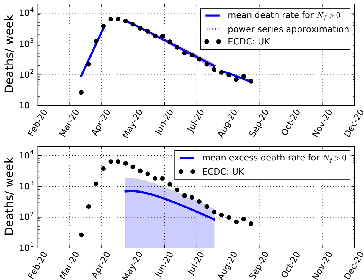
Figure 4: Upper panel: Weekly death rates in the UK. Black data points: the rates reported by the ECDC. Solid blue lines: Mean weekly deaths predicted for D_f = 0.41 d and assuming a uniform prior for N_f and a prior for R_{t,ld} after lockdown based on the CoMix study. Also shown is the 68% range of uncertainty in the mean predicted number of deaths during lockdown (shaded region). Red dotted line: Power series approximate solution during the lockdown period (see Appendix). Bottom panel: Blue solid line: Mean predicted excess deaths per week arising from fomites, along with the 95% upper limit (shaded region).
