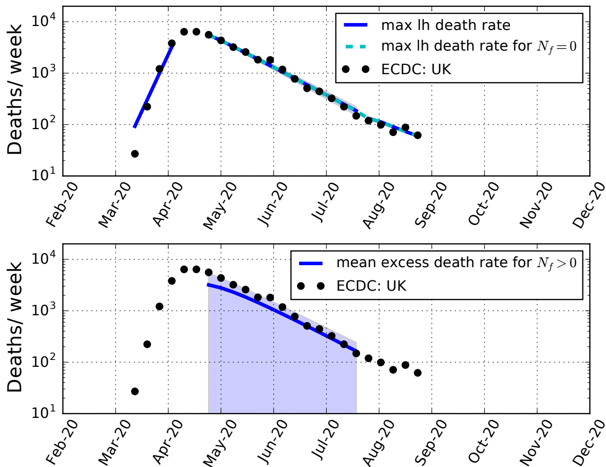
Figure 1: Upper panel: Weekly death rates in the UK. Black data points: the rates reported by the ECDC. Solid blue lines: Mean weekly deaths predicted for D_f = 0.41 d and assuming uniform priors for N_f and R_{t,ld} after lockdown. Also shown is the 68% confidence range of uncertainty in the mean predicted number of deaths during lockdown (shaded region). Broken cyan line: Maximum likelihood fit without a fomite contribution. Bottom panel: Solid blue line: Mean predicted excess deaths per week arising from fomites along with the 95% confidence upper limit (shaded region), assuming uniform priors for N_f and R_{t,ld} .
