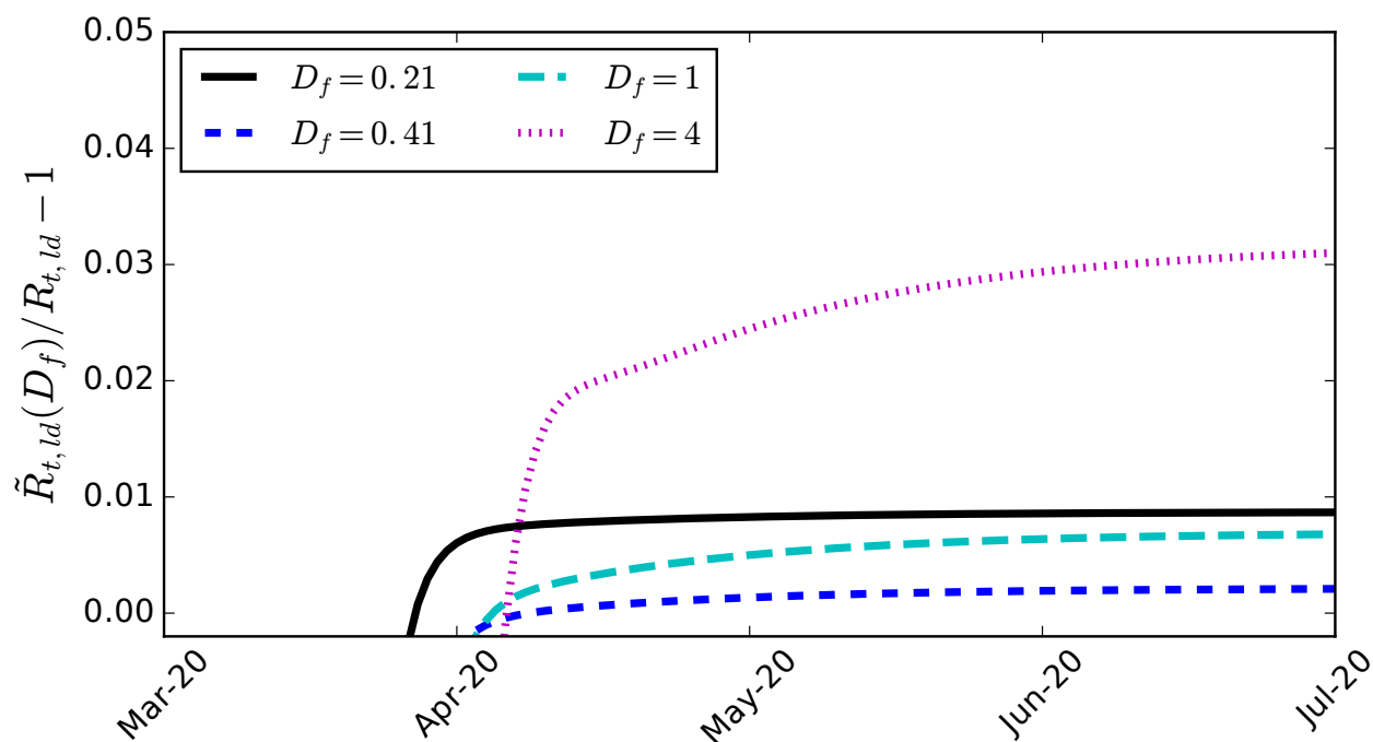
Figure 3: Relative difference between the effective reproduction number \tilde{R}_{t,ld} for models with N_f \simeq 0.14 , R_{t,ld} \simeq 0.04 , corresponding to the 95% confidence upper limits on N_f , that would be inferred from the death rates assuming a counterfactual model with N_f = 0 , compared with the maximum likelihood value for R_{t,ld} for a model with N_f = 0 . Shown for various values of D_f .
