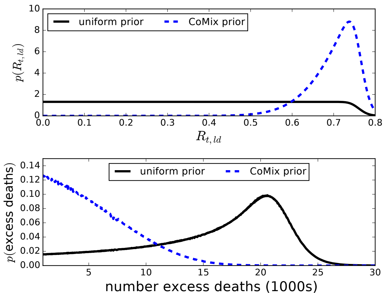
Figure 2: Upper panel: Posterior probability density for R_{t,ld} , marginalised over N_f , both for a uniform prior for R_{t,ld} (solid black line) and a prior based on the CoMix study (dashed blue line). Shown for D_f = 0.41 d. Lower panel: Probability density for excess number of deaths from fomites for D_f = 0.41 d over lockdown period, both for uniform and the CoMix prior on R_{t,ld} .
