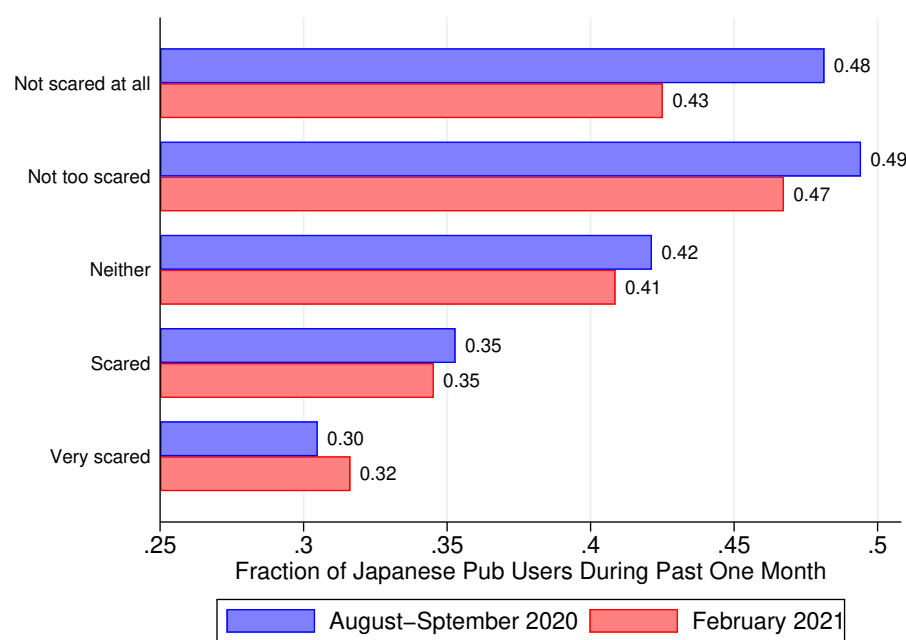
Figure SI1: Utilization Rate of Japanese Pubs and Bars by the Extent of Fear for SARS-CoV-2
