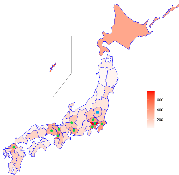
Figure 1: Infection Rate across Prefectures. The infection rate is per 100,000 persons. Note; Circles represent the 10 prefectures that declared SE in January and continued till the end of February. The square represents Tochigi prefecture, which declared the SE in January but lifted it on February 7th.
