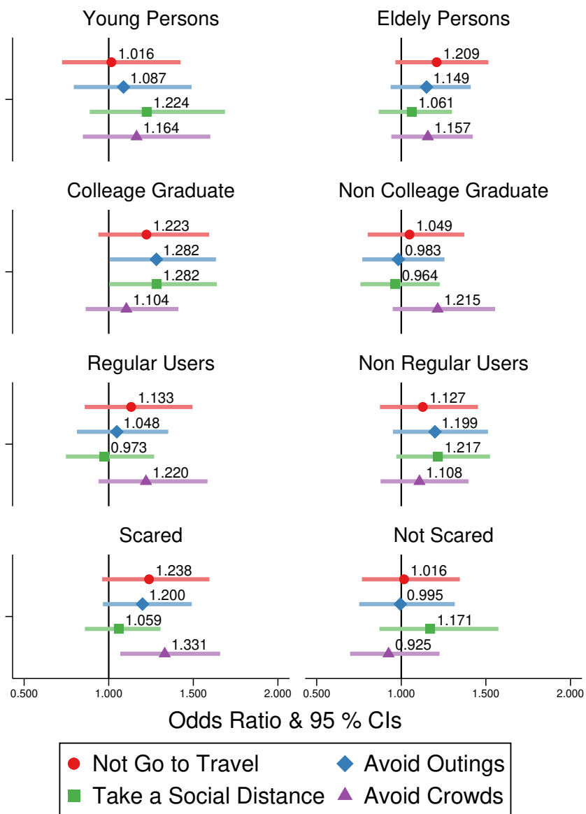
Figure SI2: Effects on Going Out Behaviors.
