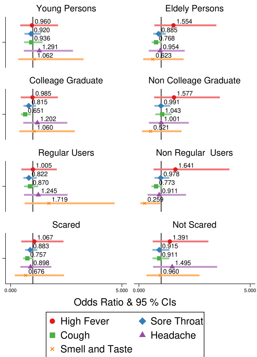
Figure 4: Effects on Symptoms of COVID-19
