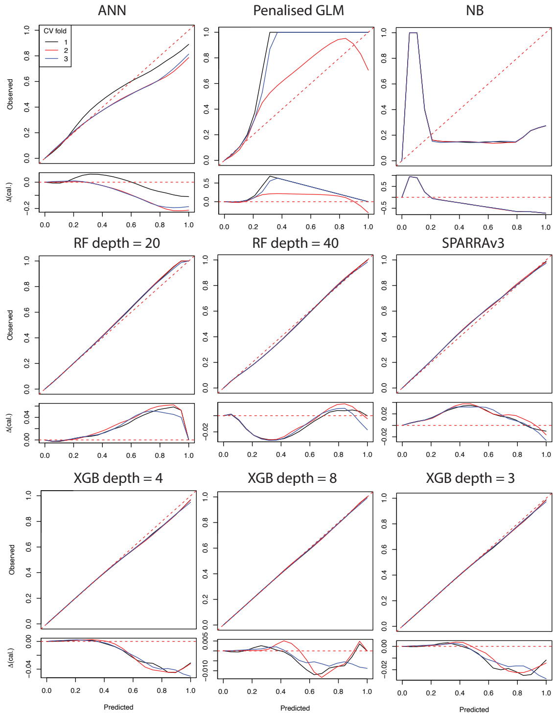
Figure S3. Calibration curves for SPARRAv4 model constituents. Estimates obtained for the test set within each CV iteration are shown in different colours (legend shown in top left panel). Bottom sub-panels show departure from perfect calibration.
