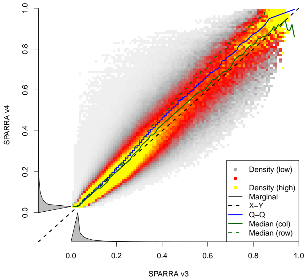
Figure S2. Density plot comparing SPARRAv3 and SPARRAv4 scores. The test datasets used within each CV iteration were combined in order to generate this plot (i.e. all samples are included once). Joint density (low to high: white-grey-red-yellow) of individual SPARRAv3 and SPARRAv4 scores. The density is normalised to uniform marginal on the Y axis, then the X axis; true marginal distributions of risk scores are shown alongside in grey.
