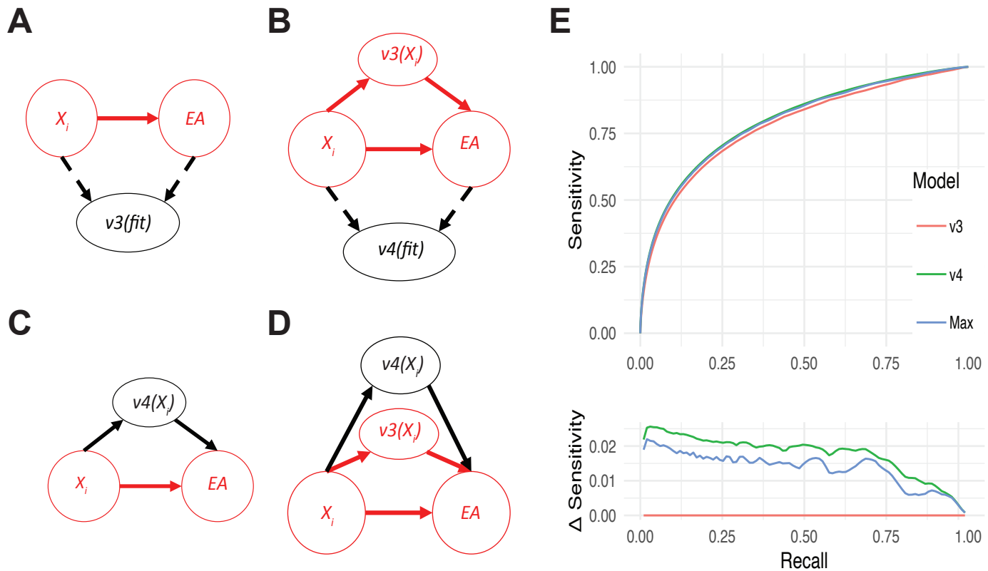
Figure S6. Model updating in the presence of performative effects. (A-D) Causal structure for the training and deployment of SPARRAv3 and SPARRAv4. X_i represents covariates for a patient-time pair; v3(\text{fit})/v4(\text{fit}) and v3(X_i)/v3(X_i) represent the fitting and deployment of v3 and v4 respectively. (A) Training setting for SPARRAv3. (B) Training setting for SPARRAv4. (C) Deployment setting if SPARRAv4 were to naively replace SPARRAv3. (D) Deployment setting in which SPARRAv4 is used as an adjuvant to SPARRAv3. (E) Comparison of predictive performance between SPARRAv3, SPARRAv4 and the maximum between both scores.
