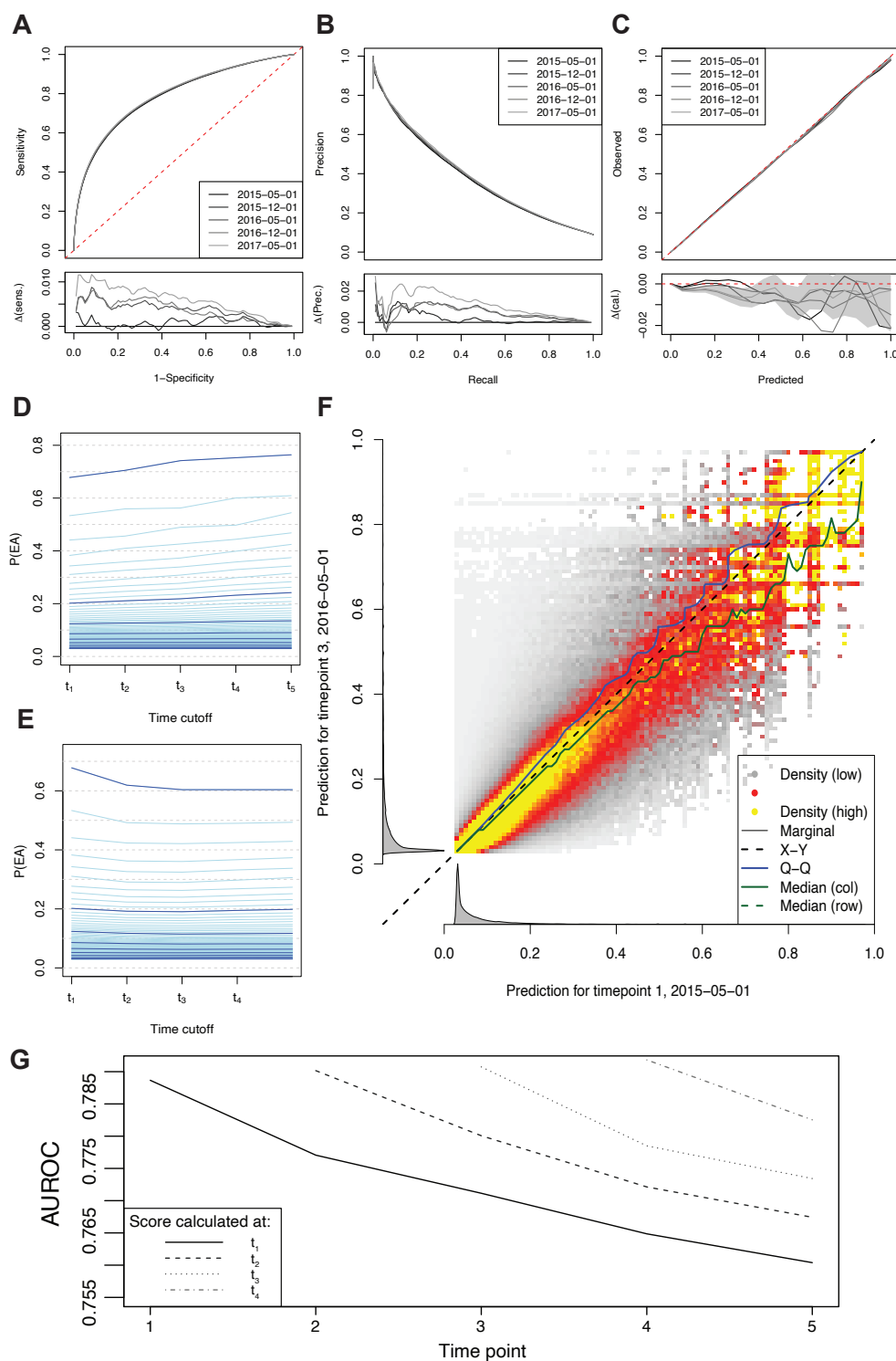
Figure S4. Performance of a static model and static predictions used to predict risk at future time points. (A-C) A model M_0 fitted to an early time point ( t_0 : 2 May 2014) was evaluated at later time points. (A) ROC curves. (B) PR curves. (C) Calibration curves. (D) Centiles (light blue) and deciles (dark blue) of risk scores (calculated using M_0 ) over time, across all individuals with data available at all time points. (E) Average score over time for groups of individuals defined by risk centiles (light blue) and deciles (dark blue) at the first t_0 (2 May 2015). (F) Density (low to high: white-grey-red-yellow) of scores generated using the static model M_0 to predict EA risk at t_1 (2 May 2015) and t_3 (1 May 2016). The density is normalised to uniform marginal on the Y axis, then the X axis; true marginal distributions of risk scores are shown alongside in grey. Plots for different time points combinations are available at https://github.com/jamesliley/SPARRAv4/tree/master/Analysis/time_attenuation/cohort/crosstime . (G) AUROCs for predictions calculated at each time point (based on M_0 ) for prediction in subsequent time points.
