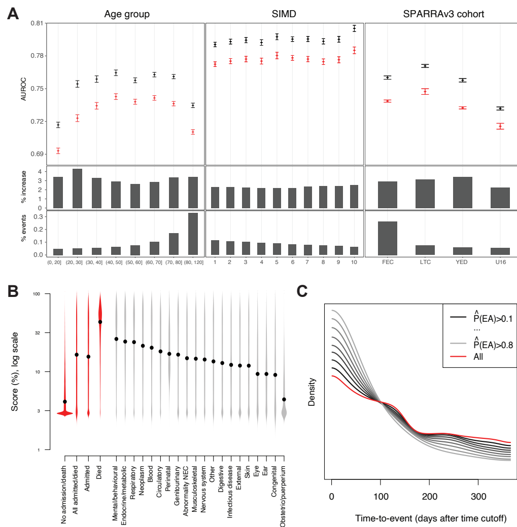
Figure 3: Stratified performance of SPARRAv3 and SPARRAv4. (A) Performance of SPARRAv3 and SPARRAv4 in subcohorts defined by age, SIMD and the original subcohorts defined during SPARRAv3 development (Methods). Top: AUROC (red: SPARRAv3; black: SPARRAv4). Vertical bars denote plus/minus 3 standard deviations. Middle: AUROC increase for SPARRAv4 with respect to SPARRAv3. For context, bottom sub-panels show the proportion of samples with an event within each group. (B) Distribution of SPARRAv4 scores (in log-scale) for different group of samples. Black points indicate the associated medians. Groups were defined according to whether an event was observed (red violin plots) or, for those with an EA, based on the diagnosis recorded during the admission. (C) Distribution of time-to-event after the first time cutoff amongst cohorts of individuals who had an EA in the year following the time cutoff and had a SPARRAv4 score above a given cutoff.
