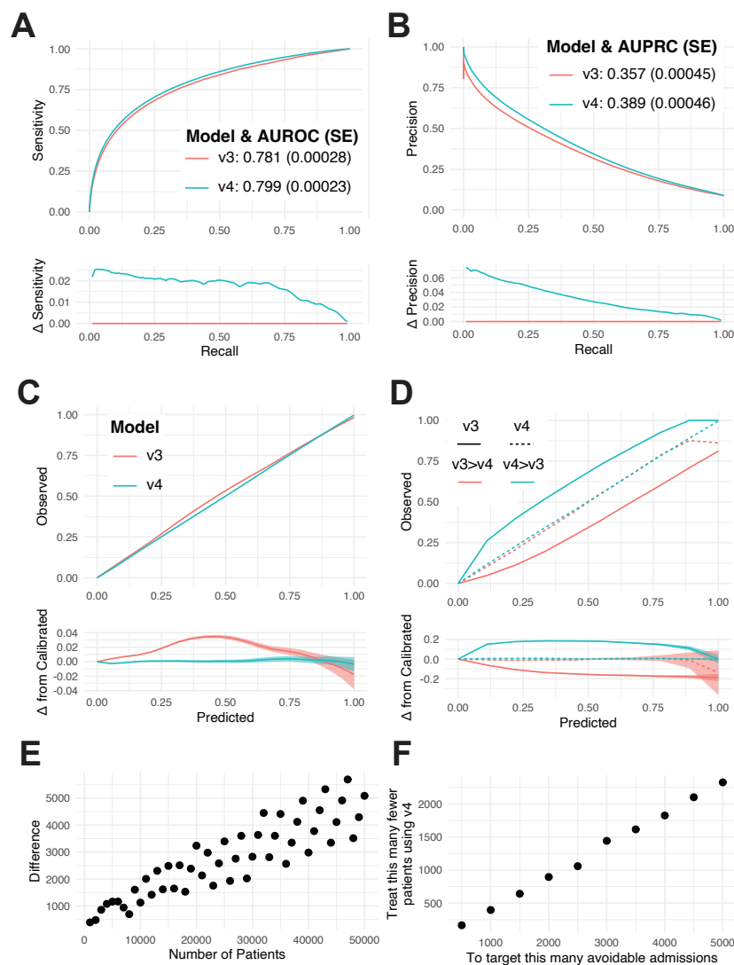
Figure 2: Comparison of overall predictive performance between SPARRAv3 and SPARRAv4. (A) ROC. (B) PRC. Lower sub-panels show differences in sensitivity and precision, respectively. Confidence intervals are negligible. (C) Calibration curves. (D) Calibration curves for samples in which |v4 - v3| > 0.1 . Lower sub-panels show the difference between curves and the y = x line (perfect calibration). Confidence envelopes are pointwise (that is, for each x -value, not the whole curve). Predicted/true value pairs are combined across cross-validation folds in all panels for simplicity. (E) Difference in the number of individuals who had an event amongst individuals designated highest-risk by v3 and v4. The repeating pattern is a rounding effect of v3. (F) Difference in the number of highest-risk individuals to target to avoid a given number of admissions.
