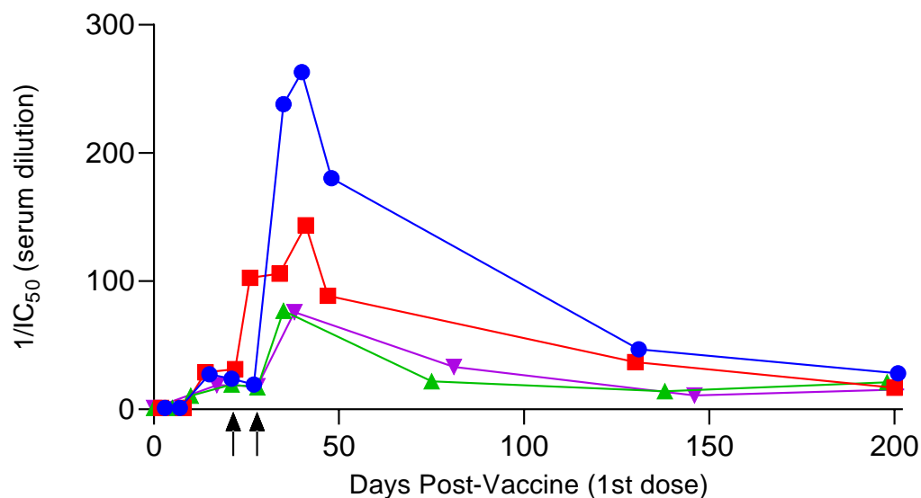
Figure 6. Changes in serum surrogate neutralizing activity over time after COVID-19 mRNA vaccination. The IC_{50} values for serial samples collected pre and up to 200 days post vaccination were calculated using the RBD-ACE2r competitive ELISA assay. Each symbol is a different individual previously described in Wisniewski et al Plos One 20201 [21]. Arrows on X-axis indicate timing of booster shots for subjects that received Pfizer-BioNTech (square), or Moderna (circle, triangle and inverted triangle). Note all samples were tested in duplicate and %CV < 10%.
