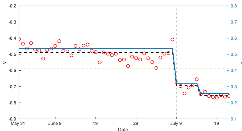
FIG. 6. (Left scale) Average of the non-residential mobility data v (red dots) and the average constant value (black dashed) over the time periods described in Table I. (Right scale) The value of p derived from the mobility data for each time period (blue line). The green line shows the threshold value for p = 0.41258 that gives R_0 = 1 .
