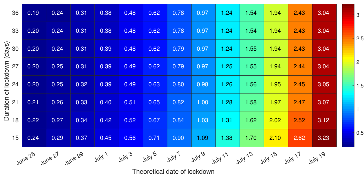
FIG. 3. Total number of cases in HCMC by August 31 as a function of when a full lockdown would have been enforced and the duration d of the full lockdown, rescaled by the total number of cases given a lockdown of length d = 21 days starting July 9 (approximately 8.2 \times 10^4 cases).
