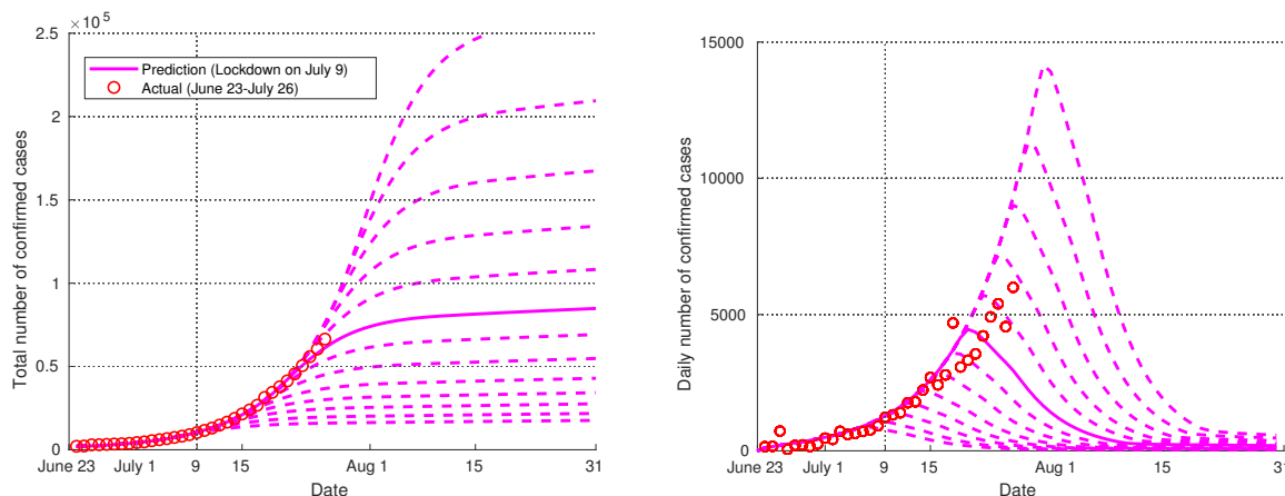
FIG. 5. The total (left) and daily (right) number of confirmed cases as a function of the length of the lockdown of when the lockdown is enforced, in increments of 2 days (June 25 to July 19). The solid line denotes the case when it is enforced on July 9. Earlier(later) implementation of Directive 16 results in lower(higher) numbers of confirmed cases.
