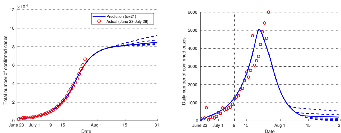
FIG. 4. The total (left) and daily (right) number of confirmed cases as a function of the length of the lockdown d , from 15 to 36 days in increments of 3. The solid line denotes the case d = 21 . Higher(lower) values of d give lower(higher) numbers of confirmed cases.
