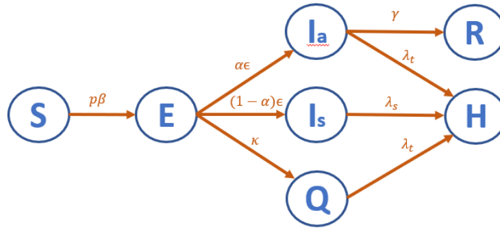
FIG. 1. A schematic of the model used
