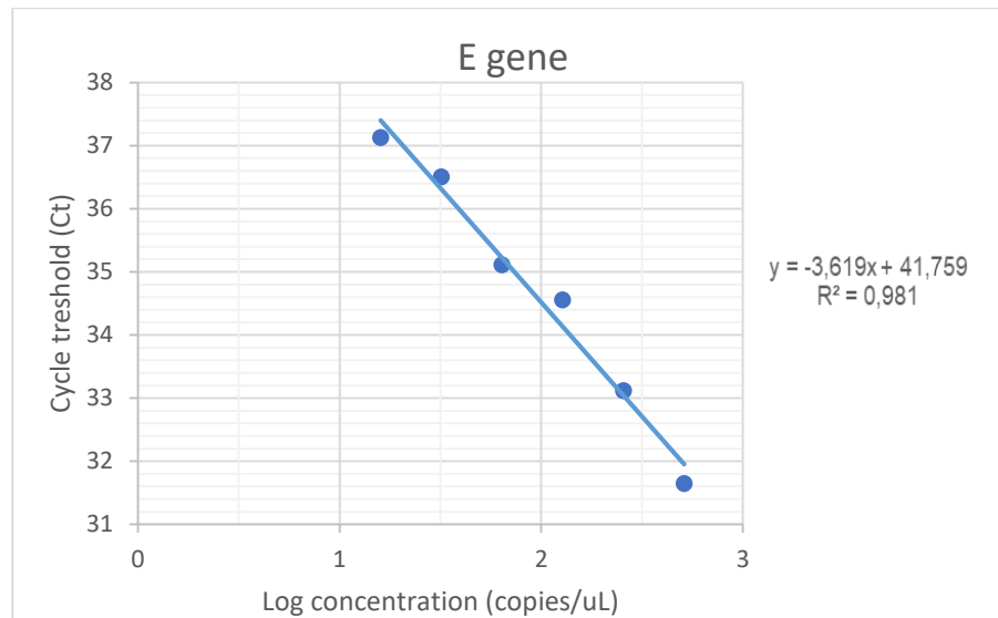
168 Figure 2. Standard curve plot of E gene from 2-fold serial dilutions of RNA standardization solution (512, 256, 128, 64, 169 32, 16 copies/uL). Primers' efficiency = 94.45 %, slope -3.619 and R2 = 0.981.
