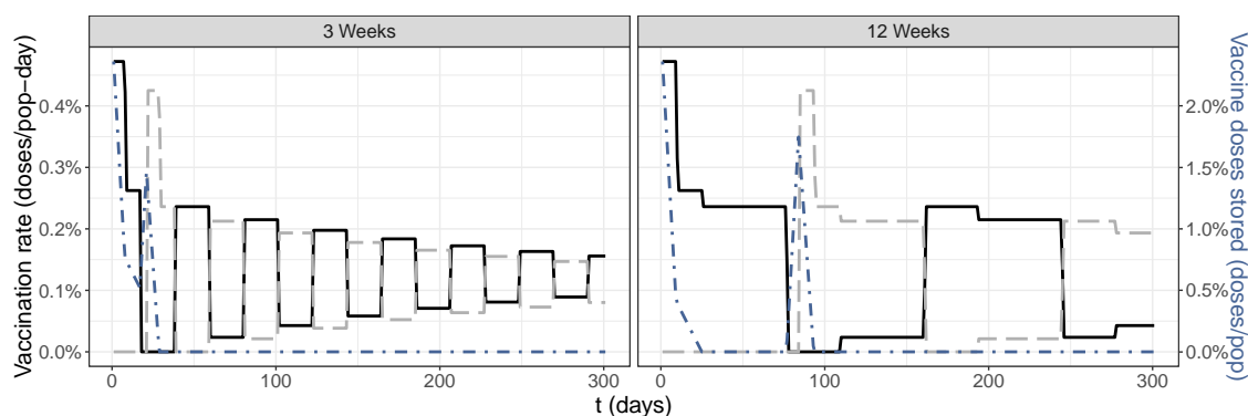
Fig. 2: Vaccination rate as a function of time for first (solid, black) and second doses (dashed, grey) – scale is given by the left y-axis. Number of stored vaccine doses as function of time (dot-dashed, blue), scale in the right y-axis. Taking into account 3 or 12 weeks (panels) as separation between doses. V_0 = 2.83\% of population in doses, \rho(t) = 0.23\% of population in doses/day, v_{max} = 0.45\% of population in doses/day.
