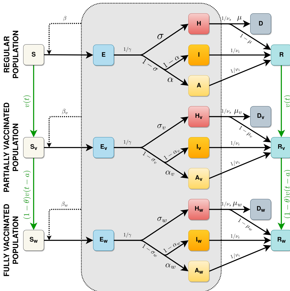
Fig. 1: Diagram representing the full model structure. Subscripts v and w indicate the first- and second-dose vaccinated classes, respectively. Black arrows indicate transitions between epidemiological stages, green arrows indicate vaccination. All classes pictured inside the gray box are infectious. Because epidemiological progressions happen at time-scales shorter than those related to vaccine effects, infectious classes are not vaccinated in the model.
