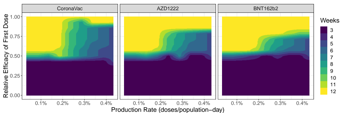
Fig. 4: Best window (color) for reduction of deaths as function of production rate ( x axis) and relative efficacy of first dose ( y axis). Each panel represents a different vaccine with the respective second dose parameters. The initial R_t is 1.1, V_0 is set to zero, vaccination rate limited to approximately 0.45% of population in doses per day.
