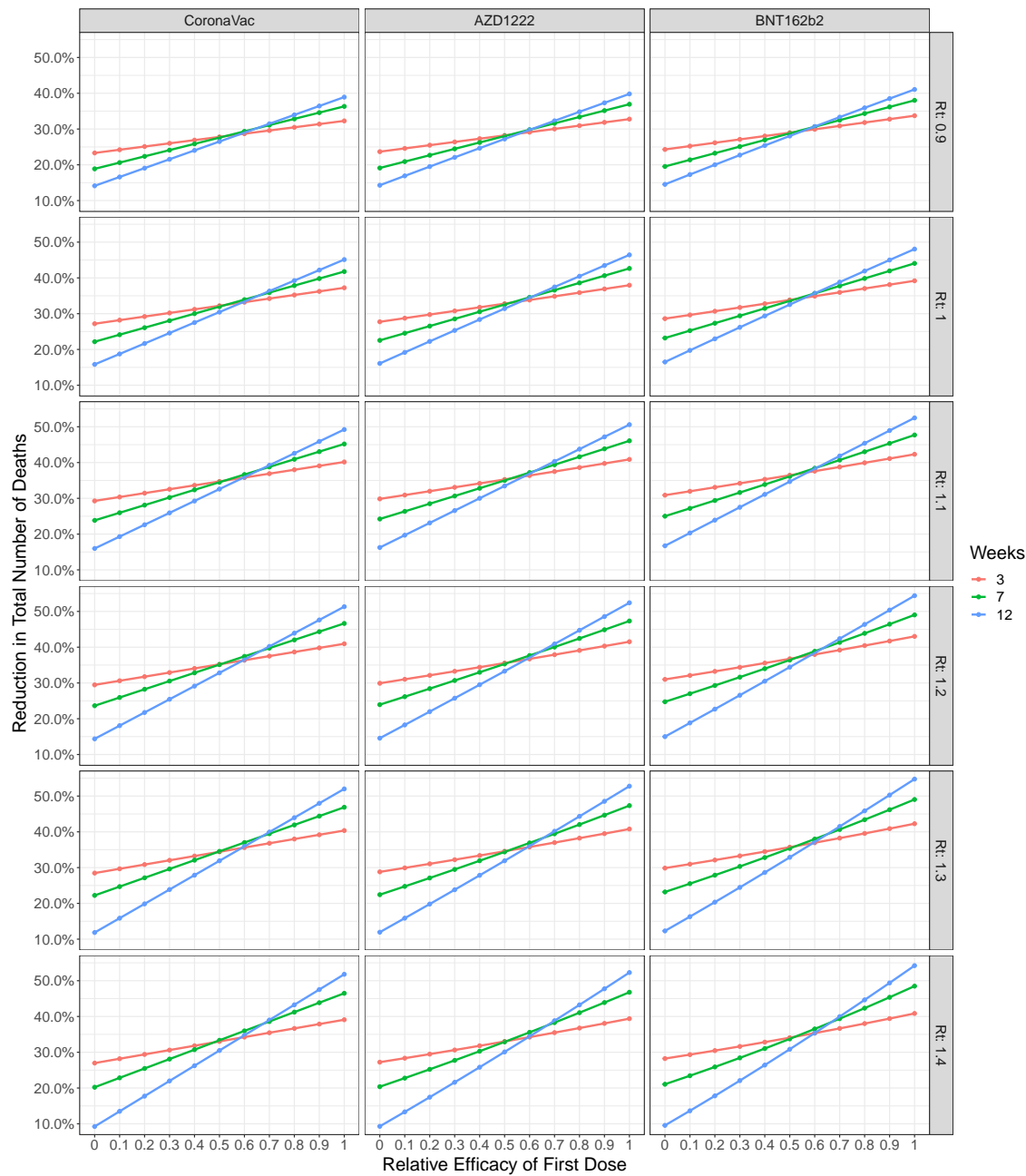
Fig. 3: Reduction in total number of deaths as function of the first dose relative efficacy, considering three time windows between doses: 3,7 and 12 weeks (colors); varying vaccine type (columns); and effective reproduction number at the start of simulation (rows). V_0 = 2.83\% of population in doses, \rho(t) = 0.23\% of population in doses/day, v_{max} = 0.45\% of population in doses/day.
