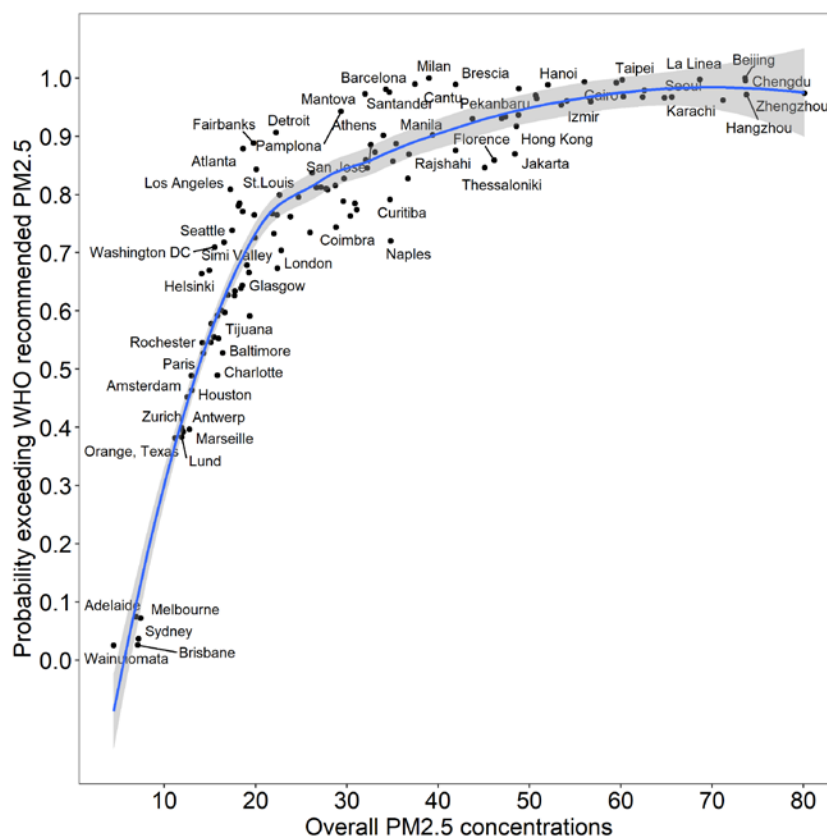
Figure 2: Probability of exceeding WHO-recommended PM 2.5 if traffic emissions are removed
