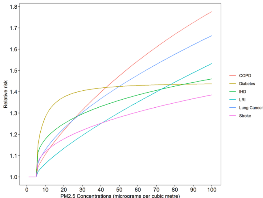
Figure 1: Integrated exposure response function (age group 55-60 years for IHD and stroke)
