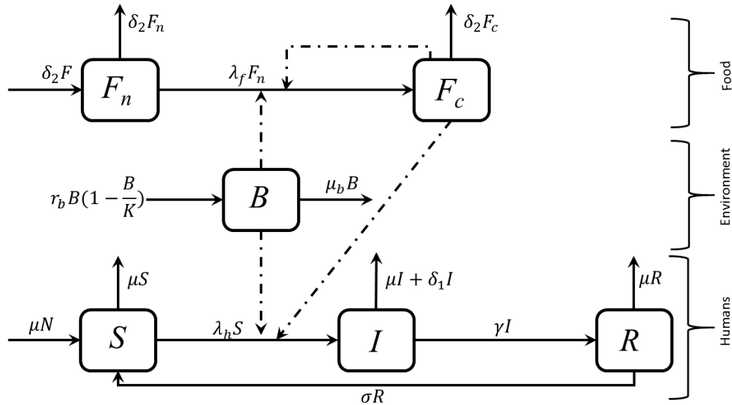
Figure 1: Model flow chart for Listeriosis disease transmission dynamics. The dotted and solid line shows the contributing factors for the human and food products to become contaminated as well as infection links respectively.
