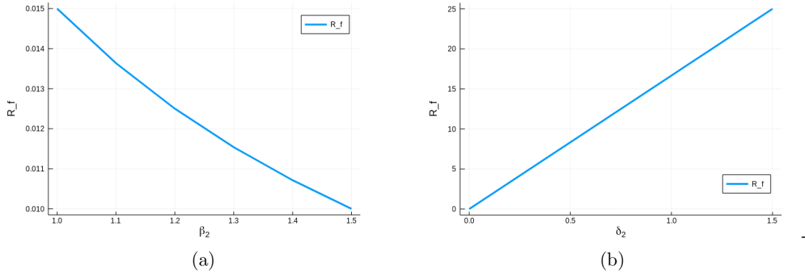
Figure 4: (a) The contamination threshold R_f with parameter values, \delta_2 = 0.015 , \hat{\beta}_2 = 1.0, 1.1, 1.2, 1.3, 1.4, 1.5 . (b) The contamination threshold R_f with parameter values, \hat{\beta}_2 = 0.06 , \delta_2 = 0.0, 1.0, 1.1, 1.2, 1.3, 1.4, 1.5 .
