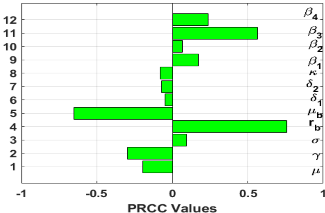
Figure 3: Tonardo plot showing different parameter PRCC values. Note that \hat{\beta}_1, \hat{\beta}_2, \hat{\beta}_3 and \hat{\beta}_4 are represented by \beta_1, \beta_2, \beta_3 and \beta_4 respectively as Matlab do not compile the \hat{\ } command.
