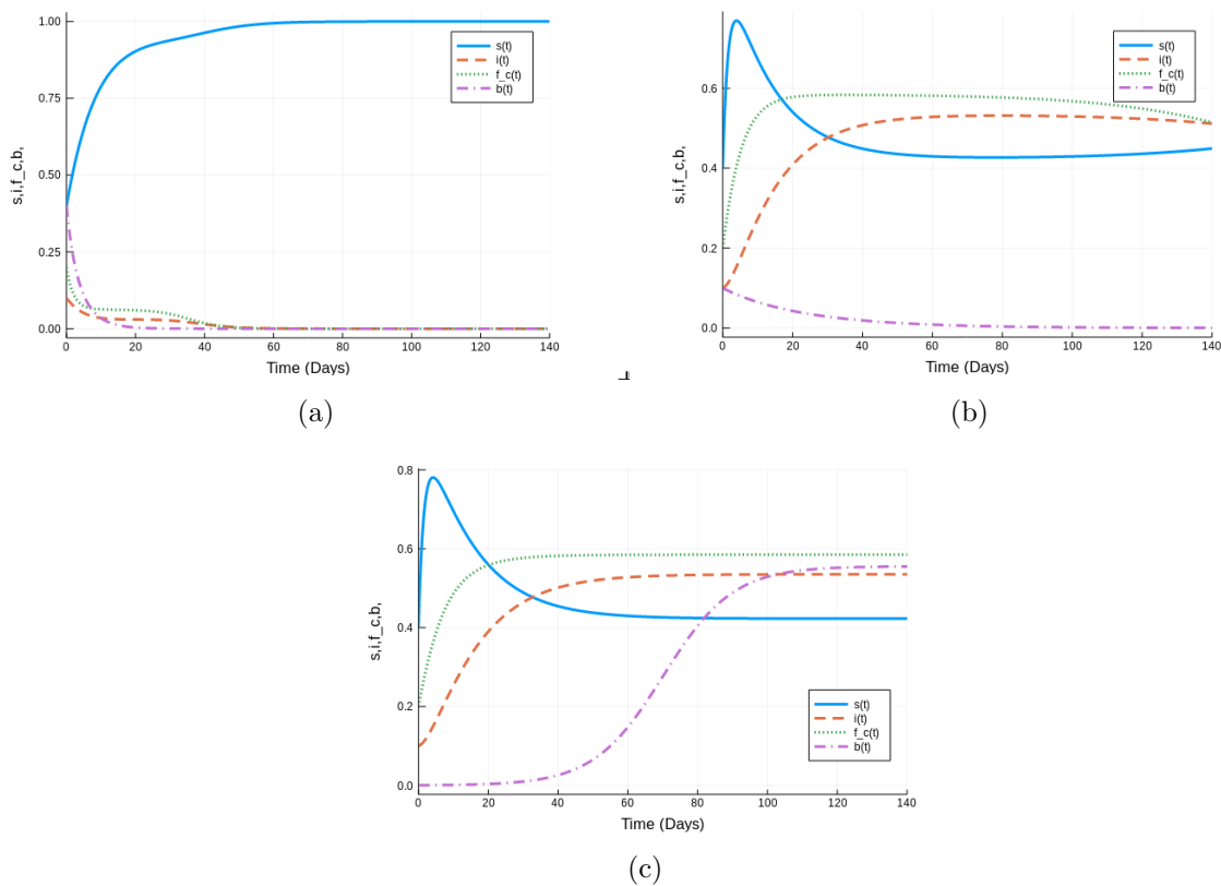
Figure 2: (a) The steady state E_0^* with parameter values \mu = 0.028, \sigma = 0.1, \gamma = 0.08, \delta_1 = 0.1, \delta_2 = 0.5, r_b = 0.18, \mu_b = 0.4, \beta_1 = 0.004, \hat{\beta}_2 = 0.006, \beta_3 = 0.03, \hat{\beta}_4 = 0.05, \hat{\kappa} = 0.0002 and initial conditions s(0) = 0.4, i(0) = 0.1, f_c(0) = 0.2, b(0) = 0.4 . (b) The steady state E_1^* with parameter values, \mu = 0.028, \sigma = 0.6, \gamma = 0.004, \delta_1 = 0.0035, \delta_2 = 0.1, r_b = 0.05, \mu_b = 0.089, \beta_1 = 0.004, \hat{\beta}_2 = 0.16, \beta_3 = 0.1, \hat{\beta}_4 = 0.07, \hat{\kappa} = 0.0002 and initial conditions s(0) = 0.4, i(0) = 0.1, f_c(0) = 0.2, b(0) = 0.1 . (c) The steady state E_2^* with parameter values in Table 2
