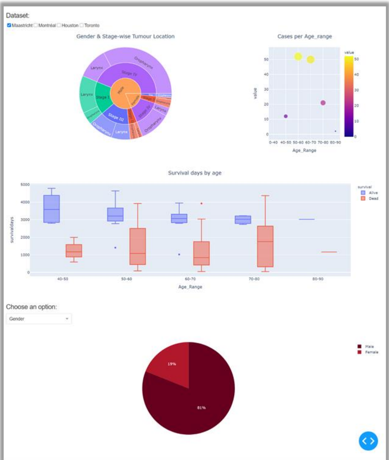
Fig 8. Visualization Dashboard
