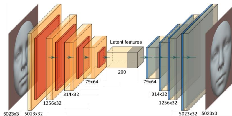
Figure 2: Framework of the auto-encoder. Red: down-sample process; Blue: up-sample process.
