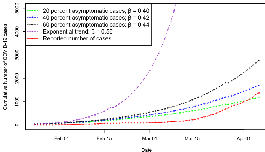
Fig. 8: SEAIHRD model simulation results
