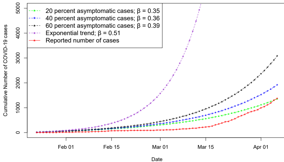
Fig. 7: SEIHRD model simulation results
