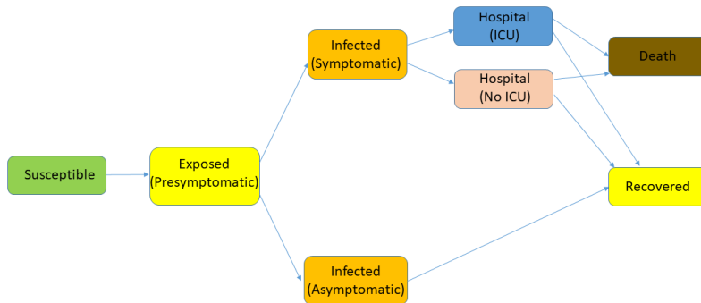
Fig. 5: SEIHRD model with asymptomatic and presymptomatic infections
