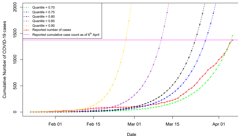
Fig. 6: Exponential model simulation results
