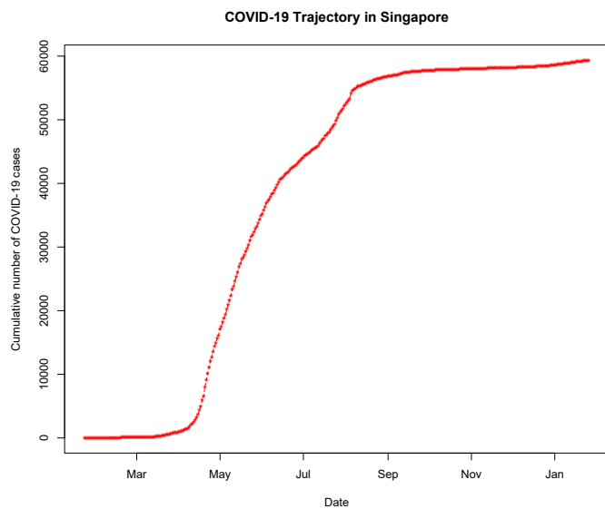
Fig. 1: Reported cumulative COVID-19 case counts in Singapore
