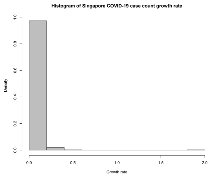
Fig. 2: Histogram of COVID-19 case count growth rates from 23 rd January 2020 to 26 th January 2021
