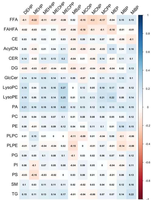
Figure 3. Correlation matrix between specific gravity corrected concentrations of phthalate metabolites and all lipid classes
