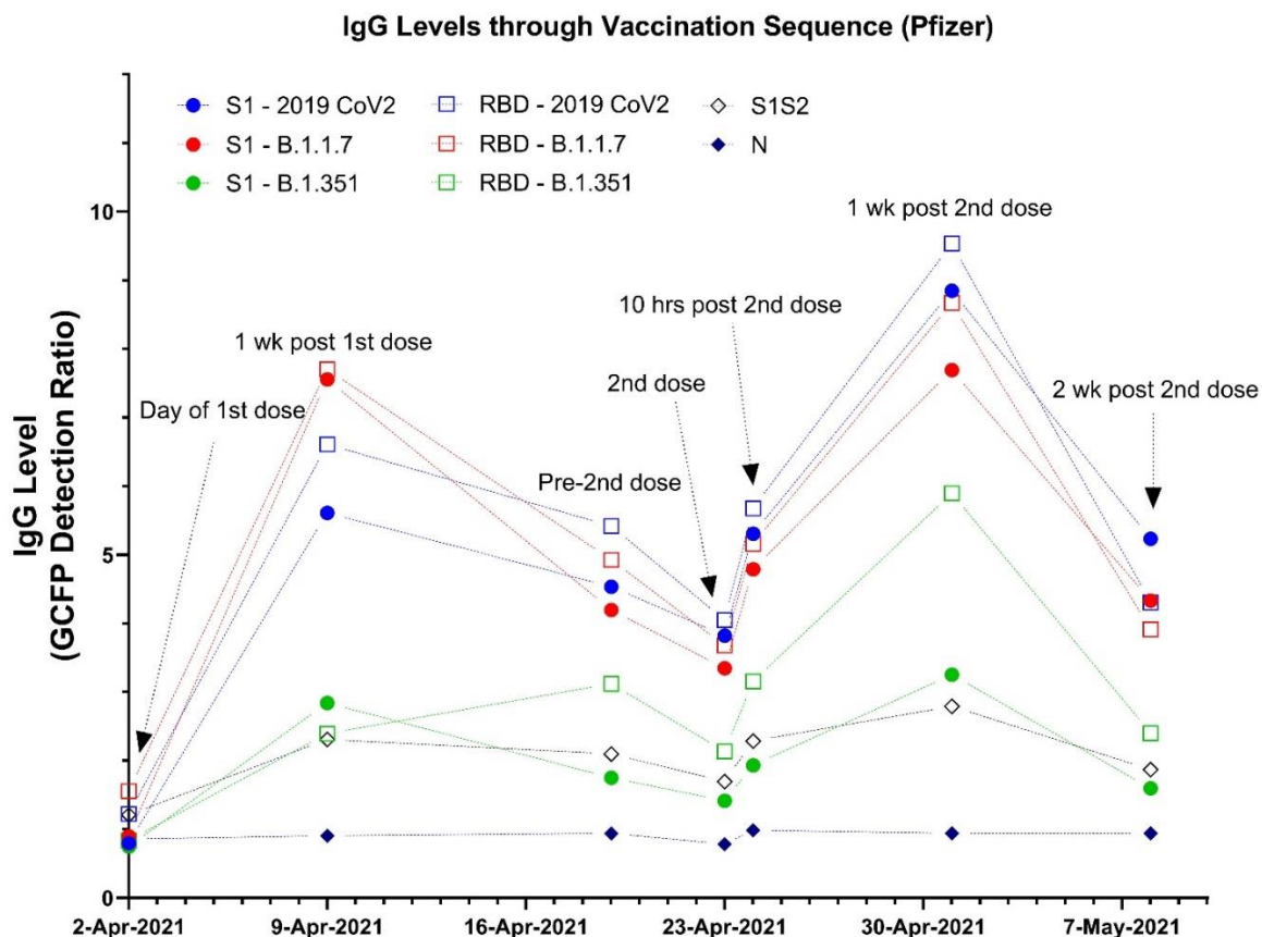
Figure 2. Human IgG levels for a single individual over the course of vaccination with the Pfizer-BioNTech vaccine, measured with GC-FP.
