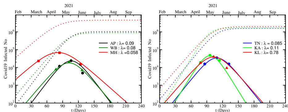
Figure 3: Same as Fig. (2) for second wave.
