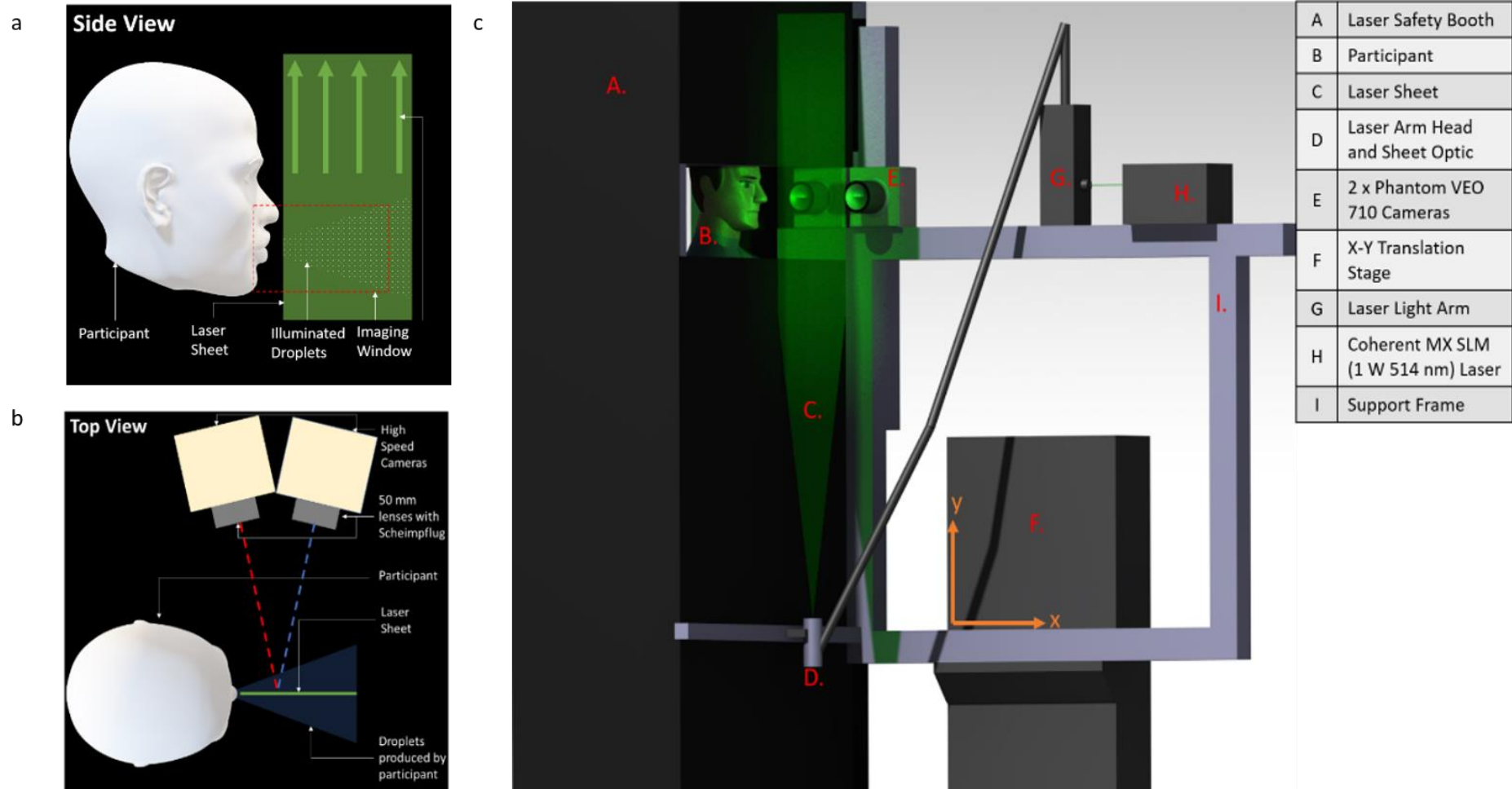
Figure 1: Diagram demonstrating a) side view and b) top view of laser sheet and camera alignment. Panel c) demonstrates the custom rig built for the experiment, including a laser safety booth for the participant.
