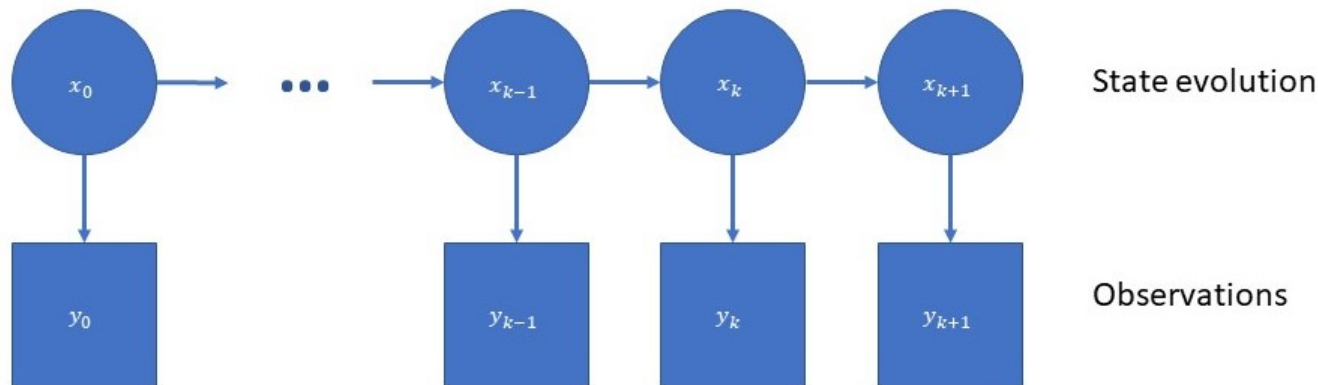
Figure 6: Dependency structure of Bayesian filter
