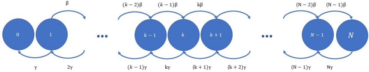
Figure 5: Continuous Time Markov Chain for Cluster-5 infected.
