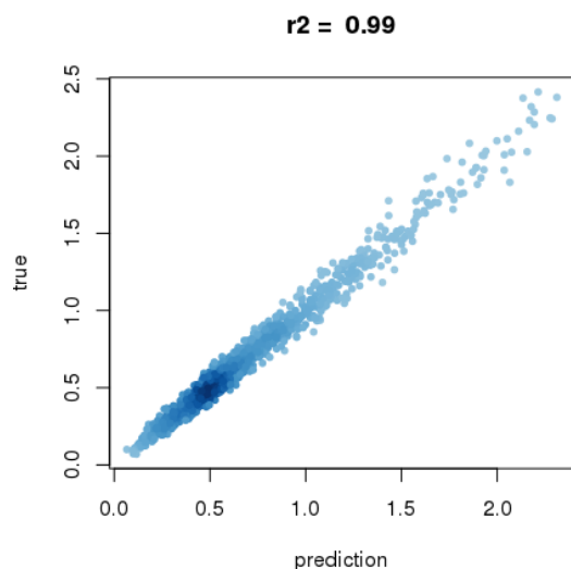
1027 Figure S 11: True over predicted RSS of the GP.
