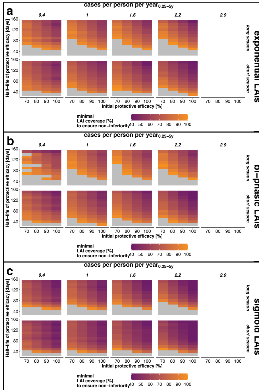
972 Figure S9: Estimated minimal LAI coverage required during implementation stages to achieve non- 973 inferiority in a given setting. Heatmap of the estimated minimal coverage (colour) of LAIs at which non- 974 inferiority to SMC-SP+AQ (assuming a fixed SMC coverage of 60% in each of the 3 or 4 rounds) is 975 achieved for different combinations of protective efficacy decay, initial protective efficacy and protective 976 efficacy half-life. The results are displayed for intervention scenarios with a high access to care ( E_{14}=0.5 ) 977 in the two seasonal settings. In the grey area, non-inferiority could not be established for any combination 978 of tool properties. The LAI coverage could not be optimized for high transmission settings (initial cases per 979 person per year 0.25-5y =2.9) because they fail to sufficiently protect the targeted population from clinical
