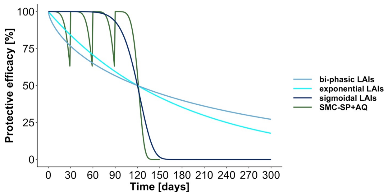
868 Figure S 3: Simulated protective efficacy decay shapes of long acting injectables (LAI) and seasonal 869 malaria chemoprevention (SMC) over one transmission season. The LAI decay shapes were chosen 870 such that they represent the three possible development streams of mAb (sigmoid decay), drug based 871 (exponential decay), or vaccine like (bi-phasic) LAIs (blue solid line). Here, we illustrated a LAI protective 872 efficacy half-life of 120 days and initial protective efficacy of 100 %. SMC – SP+AQ was parameterised 873 as specified below and administered up to four times over the transmission season (green solid line). The 874 parameterisation of the interventions is further specified in Table 1.
