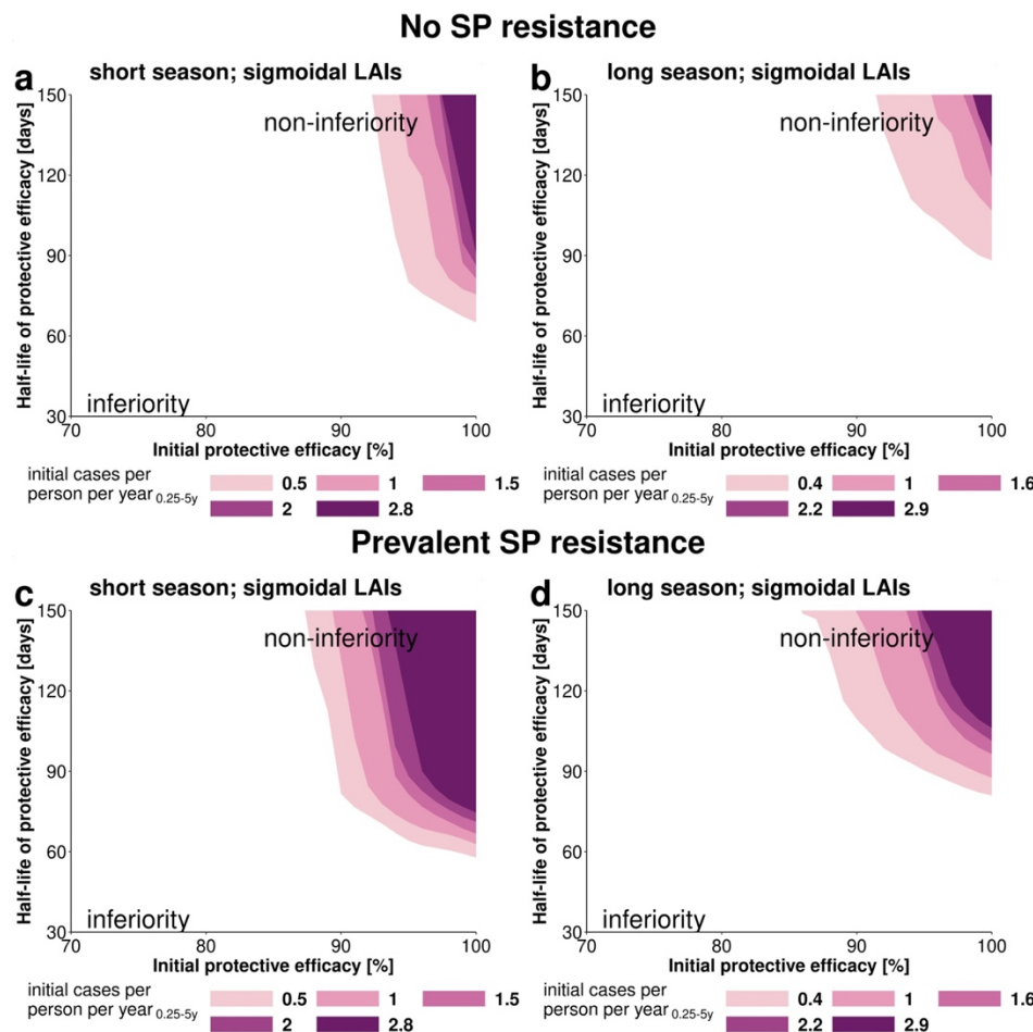
639 640 Figure 3: Parameter space under which sigmoidal LAIs achieve non-inferiority compared to SMC- 641 SP+AQ in the clinical trial stage. We investigated the ability of sigmoidal LAIs to establish non-inferiority 642 in clinical trials with an optimal deployment coverage (100%) in settings with a short (a, c) and long (b, d) 643 malaria season and over varying initial malaria incidence (initial cases per person per year 0.25-5y ). (a, b) 644 SMC-SP+AQ has an initial protective efficacy of 100% and a half-life of 32 days parameterised from 645 previous clinical trial data 1 . The influence of prevalent SP-resistance (c, d) was analyzed by decreasing the 646 protective efficacy half-life of SP from 32 days to 20 days (see Supplementary Information). The coloured 647 area defines the limits of the parameter space where non-inferiority could be established through 648 comparison of the difference hazard ratio \delta between Kaplan-Meier survival estimates (see Supplementary 649 information). The white area describes the parameter space where LAIs are inferior. Sigmoidal LAIs can 650 achieve non-inferiority compared to SMC for lower durations of protection in a shorter malaria transmission 651 season. Exponential LAIs and bi-phasic LAIs could not establish non-inferiority to SMC-SP+AQ. 652
