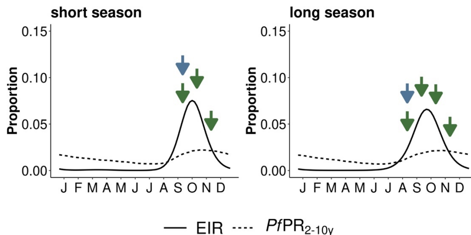
860 Figure S 2: Modelled malaria transmission pattern and simulated prevalence defining seasonality 861 settings. The seasonality in malaria transmission is defined through the proportional EIR (solid line) in 862 relation to the yearly EIR (input into the simulator). Here shown for a yearly EIR of 100 infectious bites 863 per person per year. The dotted line represents the resulting scaled yearly prevalence profile. The arrows 864 illustrate the administration of the preventative interventions of SMC-SP+AQ (green) and LAI (blue) in the 865 two seasonal settings. Following WHO recommendations 1 , SMC-SP+AQ was implemented monthly with 866 the first dose administered before the peak and the second dose with the peak in malaria transmission.
