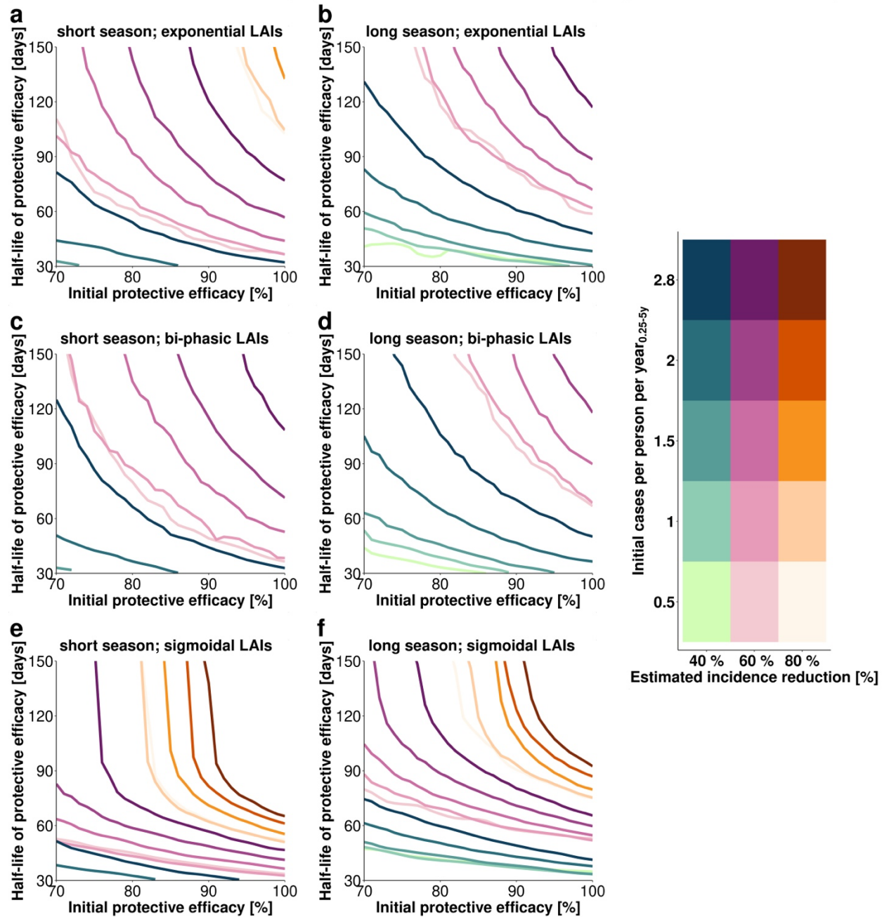
623 Figure 2: Achieving targeted malaria incidence reduction depends on the decay shape of the LAIs 624 protective efficacy. Estimated relationships between initial protective efficacy and efficacy half-life for 625 different incidence reduction criteria (40%, 60% and 80%, line style and color) and clinical incidence 626 settings (increasing color intensity indicates an initial clinical incidence measured in cases per person per 627 year in the target age group of 0.5, 1, 1.5, 2, and 2.8). Each line shows the minimum required LAI 628 characteristics to reach the desired health goal at a 100% LAI deployment coverage at clinical trial stage , 629 with all parameter combinations below a line failing to meet those requirements. The panels show 630 the parameter space of attainable incidence reductions within the specified constrained ranges of initial 631 protective efficacy and half-life for exponential LAIs (a, b), bi-phasic LAIs (c, d) and sigmoidal LAIs (e, f) 632 in settings with a short (Senegal-like a, c, e) or long (Mali-like b, d, f) malaria season. The incidence 633 reduction was calculated by comparing the incidence over one transmission season after application of the
