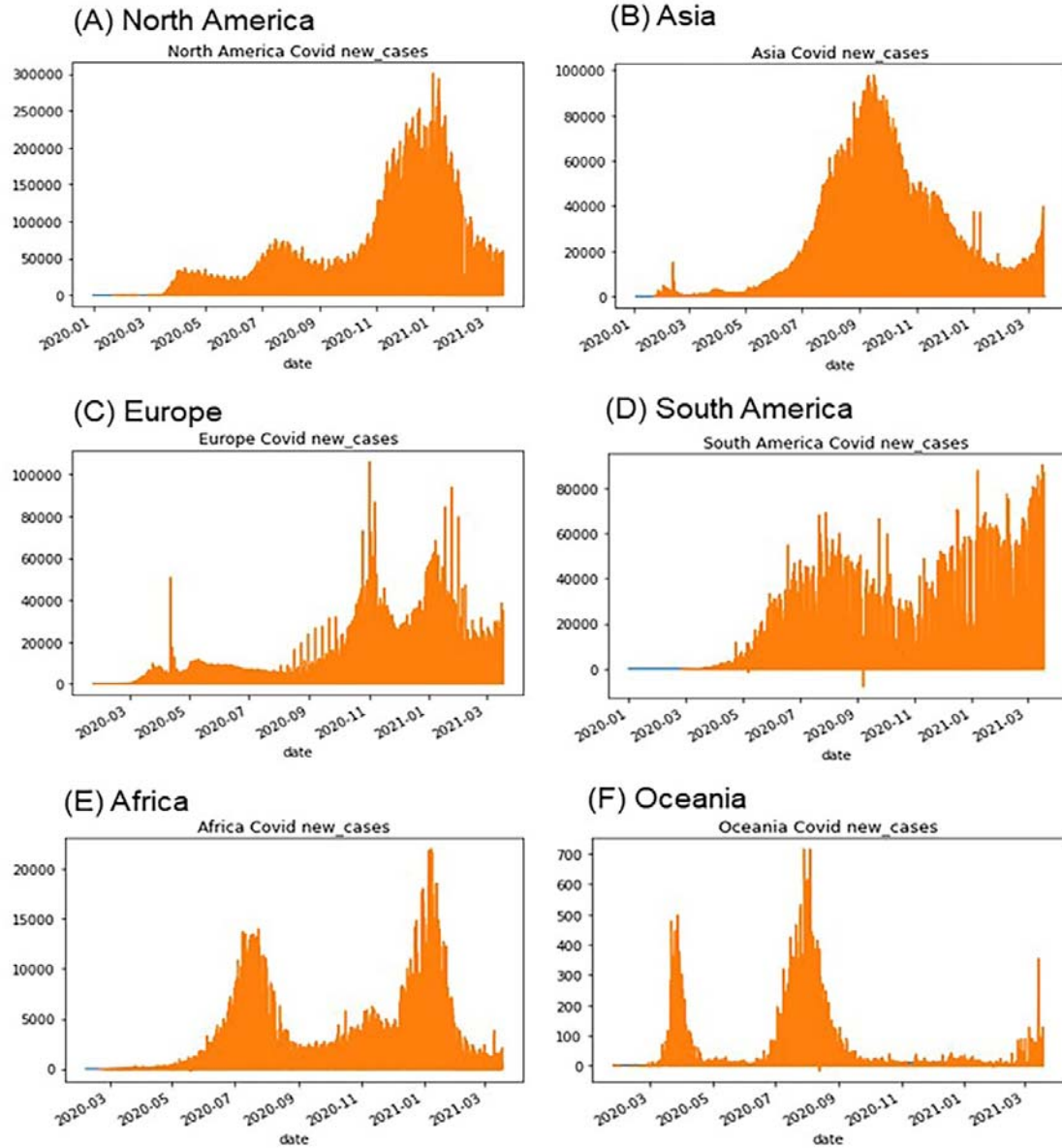
Figure-5 Histogrammic representation of COVID-19 updated cases in various regions.
