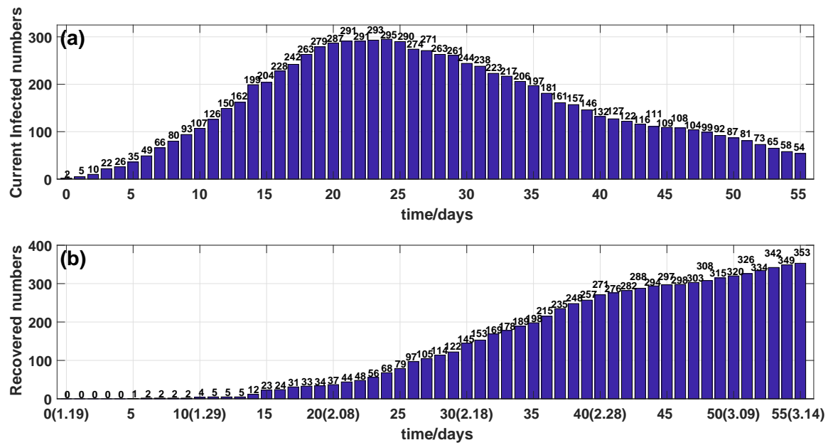
Figure 2: (a) Outcome of the number of current infected individuals. (b) Outcome of the number of cumulative recovered individuals.
