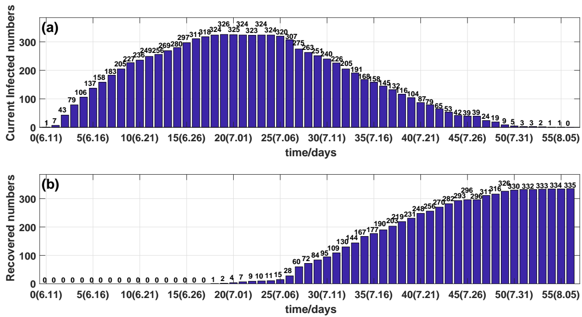
Figure 7: (a) Outcome of the number of current symptomatic infected individuals. (b) Outcome of the number of cumulative recovered symptomatic infected individuals.
