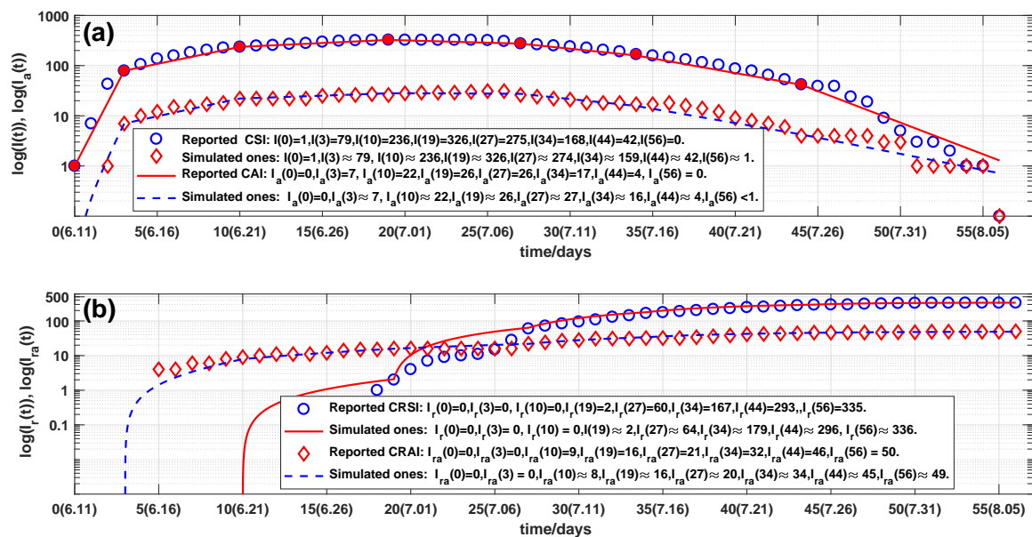
Figure 9: Outcomes of the numbers of: (a) current symptomatic individuals (CSI) and current asymptomatic individuals (CAI), representing by circles and diamonds. Solid line and dash line are the corresponding stimulated ones of system (18). Outcomes of the numbers of: (b) cumulative recovered symptomatic individuals (CRSI) and cumulative recovered asymptomatic individuals (CRAI), representing by circles and diamonds, respectively. Solid line and dash line are corresponding simulations of system (18).
