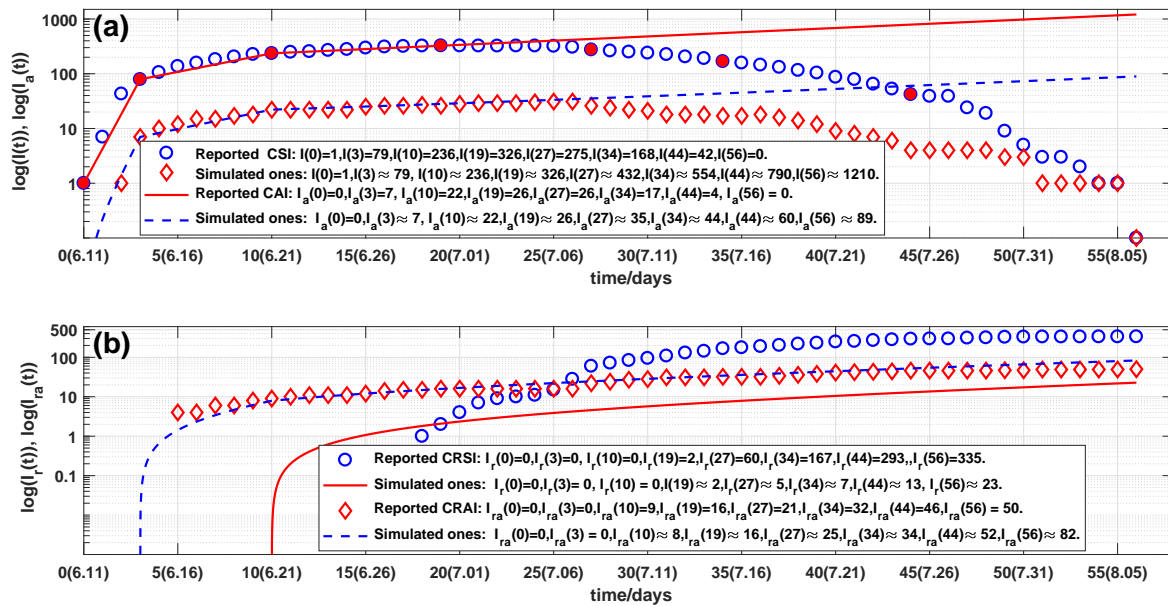
Figure 10: Virtual simulations. Outcomes of the numbers of: (a) current symptomatic individuals (CSI) and current asymptomatic individuals (CAI), representing by circles and diamonds. Solid line and dash line are the corresponding stimulated ones of system (18). Outcomes of the numbers of: (b) cumulative recovered symptomatic individuals (CRSI) and cumulative recovered asymptomatic individuals (CRAI), representing by circles and diamonds, respectively. Solid line and dash line are corresponding simulations of system (18).
