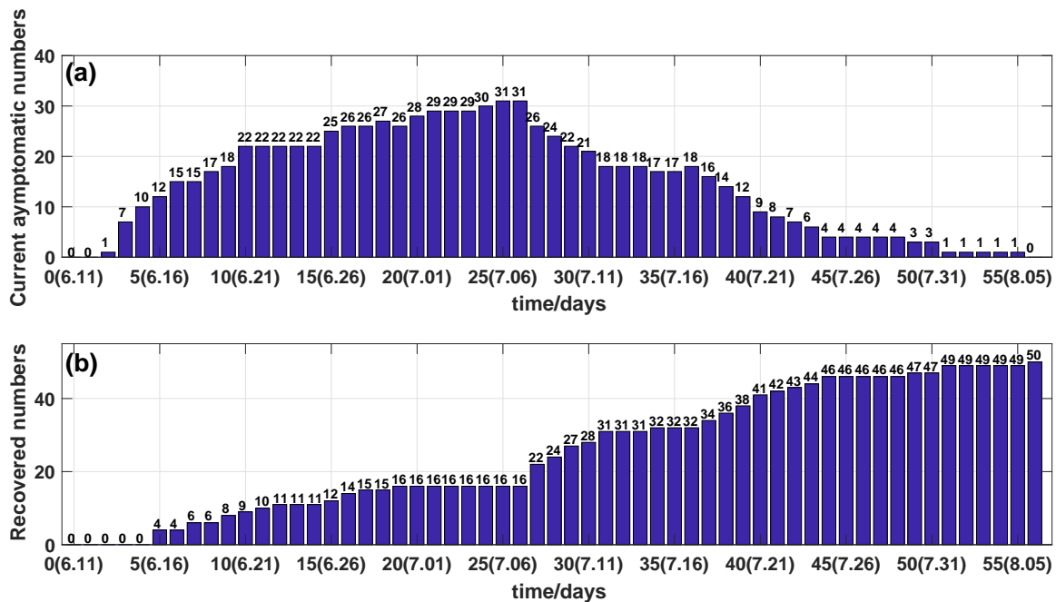
Figure 8: (a) Outcome of the number of current asymptomatic infected individuals. (b) Outcome of the number of cumulative recovered asymptomatic infected individuals.
