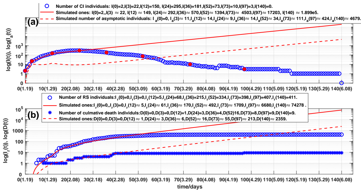
Figure 4: Virtual simulations: (a) Outcome of the number of current symptomatic individuals, representing by circles. Solid line and dash line are outcomes of stimulated current symptomatic and asymptomatic individuals of system (1). (b) Outcomes of the numbers of cumulative recovered symptomatic and died individuals, representing by circles and stars, respectively. Solid line and dash line are corresponding simulations of system (1).
