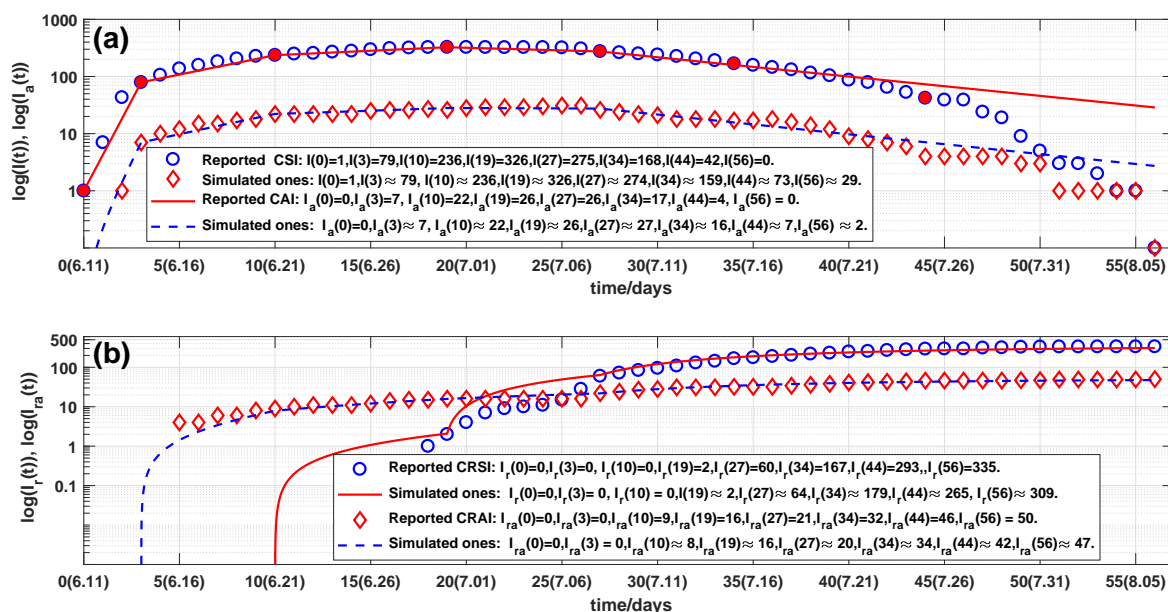
Figure 11: Virtual simulations. Outcomes of the numbers of: (a) current symptomatic individuals (CSI) and current asymptomatic individuals (CAI), representing by circles and diamonds. Solid line and dash line are the corresponding stimulated ones of system (18). Outcomes of the numbers of: (b) cumulative recovered symptomatic individuals (CRSI) and cumulative recovered asymptomatic individuals (CRAI), representing by circles and diamonds, respectively. Solid line and dash line are corresponding simulations of system (18).
