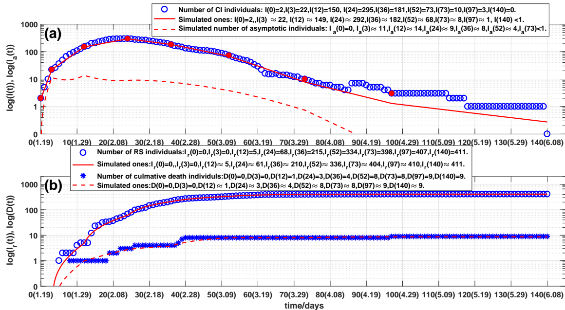
Figure 3: (a) Outcome of the number of current symptomatic individuals, representing by circles. Solid line and dash line are outcomes of stimulated current symptomatic individuals and stimulated current asymptomatic individuals of system (1). (b) Outcomes of the numbers of cumulative recovered symptomatic and died individuals, representing by circles and stars, respectively. Solid line and dash line are corresponding simulations of system (1).
