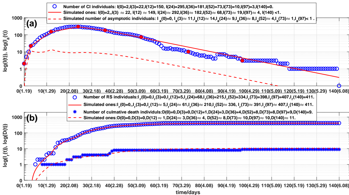
Figure 5: Virtual simulations: (a) Outcome of the number of current symptomatic individuals, representing by circles. Solid line and dash line are outcomes of stimulated current symptomatic asymptomatic individuals of system (1). (b) Outcomes of the numbers of cumulative recovered symptomatic and died individuals, representing by circles and stars, respectively. Solid line and dash line are corresponding simulations of system (1).
