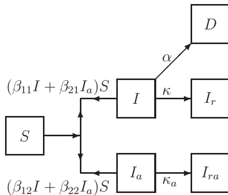
Figure 1: Flowchart of disease transmission among susceptible population S , current symptomatic infected individuals I , current asymptomatic but infected individuals I_a , recovered symptomatic infected individuals I_r , recovered asymptomatic but infected individuals I_{ra} , and died individuals D .
