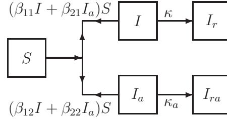
Figure 6: Flowchart of disease transmission among susceptible population S , current symptomatic infected individuals I , current asymptomatic but infected individuals I_a recovered symptomatic infected individuals I_r , recovered asymptomatic but infected individuals I_{ra} .
