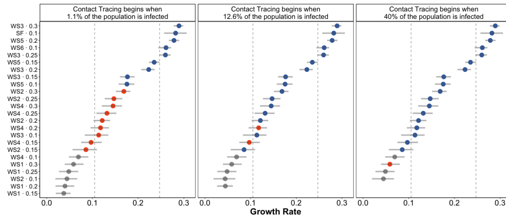
Fig. 4. Classifications of the phases for variations of starting points of contact tracing. Vertical dashed lines represent boundaries between phases under the default setting, i.e., contact tracing is initiated when the first individual tests positive. We follow the same color code as in Figure 3. When the starting point is at 1.1%, we find some red circles at the left of the left vertical dashed lines, and some blue circles at the left of the right vertical dashed lines. This phenomenon is more pronounced as contact tracing is delayed. Points and bars indicate the mean and 5th-95th percentiles.
