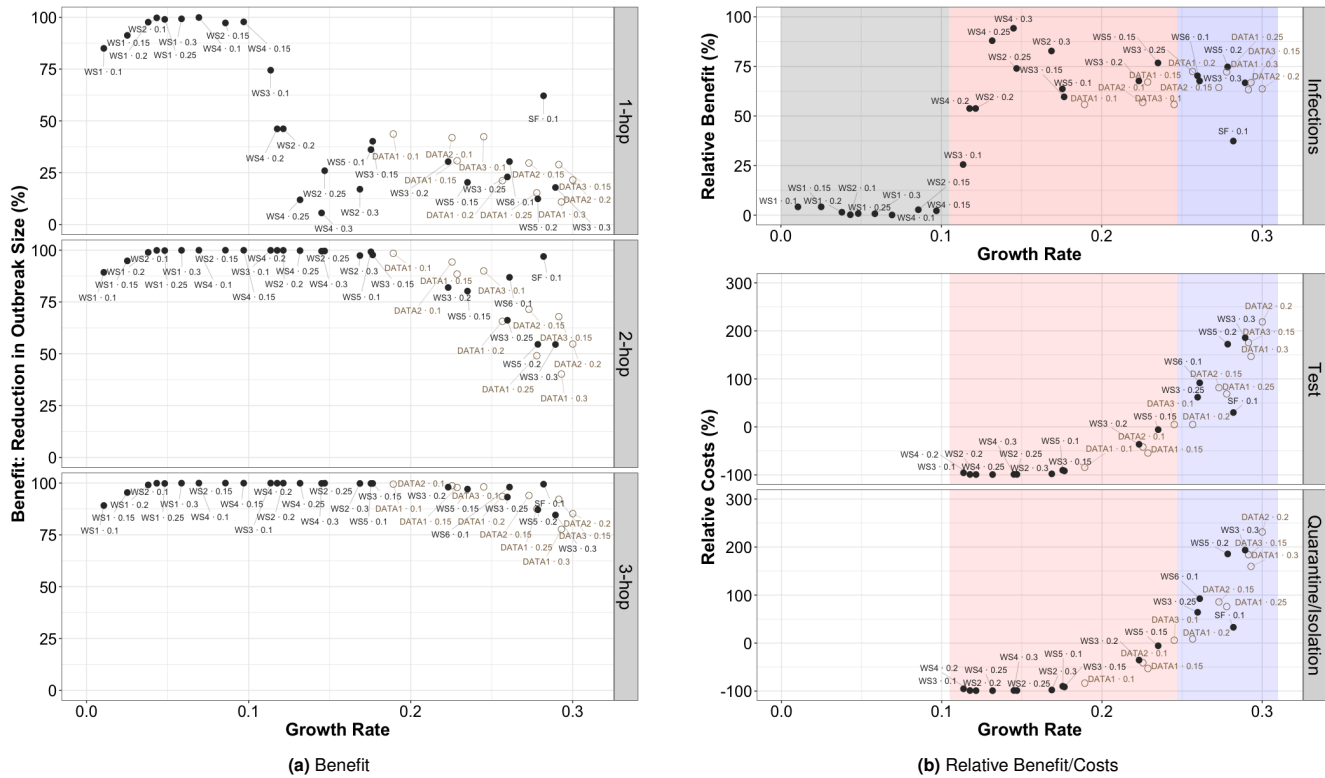
Fig. 2. (a) Benefit each policy provides, from 1-hop to 3-hop contact tracing under the default setting. This represents the percentage of reduction in the number of infections when k -hop contact tracing was performed compared to when no contact tracing was performed. (b) Relative benefit and relative costs for 3-hop contact tracing under the default setting. These respectively represent the incremental benefits and costs 3-hop contact tracing provides/incurs as compared to 1-hop contact tracing. The gray, red, and blue shaded regions respectively represent phase A, B, and C under the default setting. For both (a) and (b), each point represents one of a combination of contact pattern and transmission probability. For example, WS1 · 0.1 represents that the contact pattern corresponds to WS1 network (among the networks listed in Table 1) and the transmission probability is 0.1. Regardless of types of contact tracing scheme, the contact pattern and the transmission probability uniquely determine the growth rate ( x -axis) that characterizes the intrinsic speed of virus spread in the absence of any public health intervention. The filled and open circles correspond to synthetic networks and data-driven networks, respectively.
