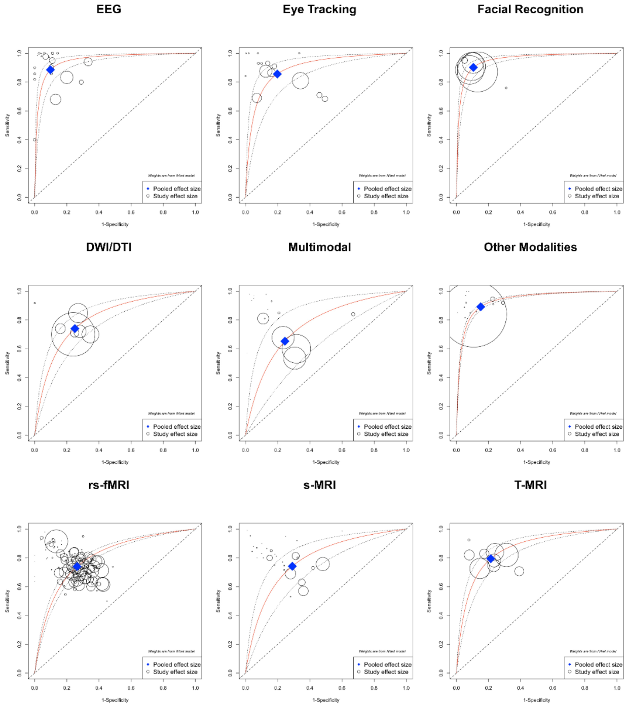
Figure 5 | Summary Receiver Operating Characteristics (SROC) curves for SCS analysis of 232 included studies. The confidence limits of the DOR are also shown in the plot. Individual study Se/Sp pairs are indicated on the plot as open circles with size proportional to the inverse of the variance of the study's logarithm of DOR. For better visualization purposes, the size proportions of open circles are different between graphs.
