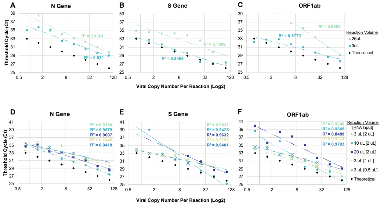
Fig S1. (A-C) RT-qPCR performance of miniaturized (3 \mu L) and full-scale (25 \mu L) reactions as compared to theoretical results, for three targeted regions of the SARS-CoV-2 genome: (A) N Gene; (B) S Gene; (C) ORF1ab. (D-F) RT-qPCR performance of different reactions (varied total reaction volume and RNA input volume) as compared to theoretical results, for three targeted regions of the SARS-CoV-2 genome: (A) N Gene; (B) S Gene; (C) ORF1ab. Every point in each graph represents the average of 3 technical replicates.
