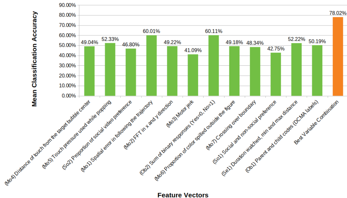
Figure 4: Bar graphs showing comparison of mean classification accuracies of the feature vectors taken from the eight tasks included in the START battery. The figure also represents the best classification accuracy achieved by a combination of these features. (Prefixes on x-axis in brackets refer to corresponding feature IDs). Note that some features are designed as multidimensional vectors with different measures along its dimensions
