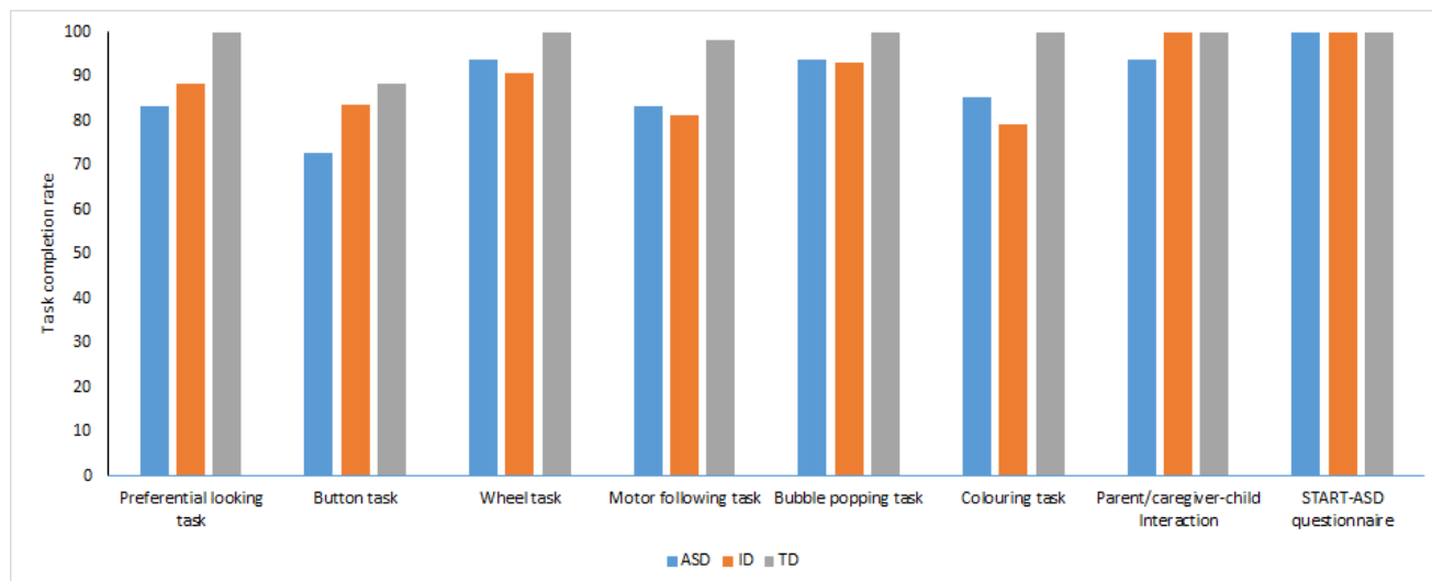
Figure 5: Task completion rate for each START task for each of the three groups of children (ASD, ID and TD)
