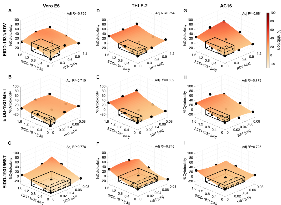
Fig. 5. Validation of EIDD-1931 drug interactions affecting %Cytotoxicity. (A-I) Surface plots of EIDD-1931 interactions with remdesivir (RDV), baricitinib (BRT) and masitinib (MST), in the validation interaction space, clinically actionable interaction space (black, solid line border) and the interaction space from the IDentif.AI analysis (black, dotted line border), based on the experimentation in Vero E6 cells (A-C), THLE-2 (D-F) and AC16 (G-I). (A-I) All experiments were performed with N = 3 to 4 replicates, which were independently included in the surface construction. Black, round markers indicate an average %Cytotoxicity of the replicates for each data point. Adjusted R^2 (Adj R^2 ) indicates goodness of the fit for each interaction surface.
