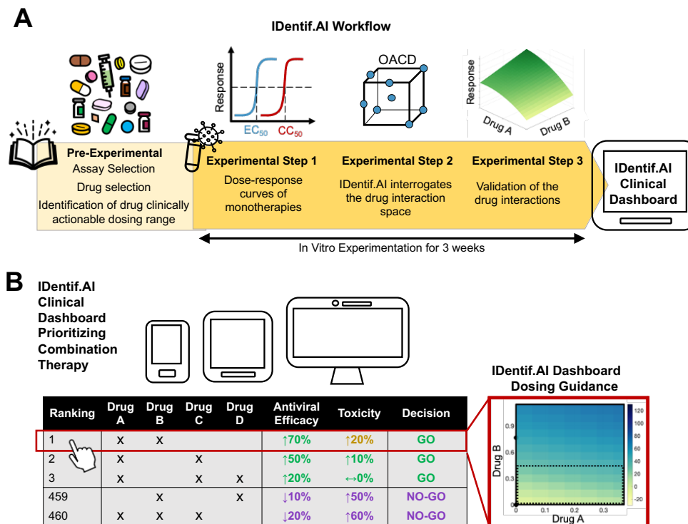
Fig. 1. IDentif.AI workflow and actionable outcome. A) IDentif.AI workflow for optimizing drug combinations. Clinical applicability considerations are integrated into IDentif.AI workflow to pre-emptively best position the optimized combinations for a clinical translation. B) The outcome of the IDentif.AI workflow is a list of ranked combinations for prioritizing drug combinations for go/no-go decisions.
