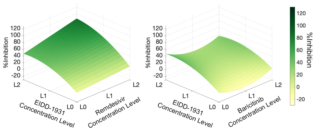
Fig. 2. Identif.AI interaction analysis. The analysis indicates that EIDD-1931 interacts differently with remdesivir and baricitinib. EIDD-1931/remdesivir interaction surface had a convex shape indicating a synergistic interaction, while EIDD-1931/baricitinib had a concave interaction surface had a concave shape indicating a dose-dependent, mildly antagonistic interaction. L0, L1, L2 correspond to concentration Level 0, Level 1 and Level 2.
