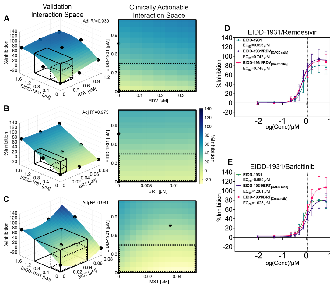
Fig. 3. Validation of EIDD-1931 drug interactions affecting %Inhibition. (A-C) Surface plots of EIDD-1931 interactions with remdesivir (RDV), baricitinib (BRT) and masitinib (MST) in the validation interaction space, clinically actionable interaction space (black, solid line border) and the interaction space from the IDentif.AI 2.0 analysis (black, dotted line border). The latter two are also shown as 2-dimensional maps. All experiments were performed with N = 3 to 4 replicates, which were independently included in the surface construction. Black, round markers indicate an average %Inhibition of the replicates for each treatment. Adjusted R^2 (Adj R^2 ) indicates goodness of the fit for each interaction surface. (D-E) Dose-response curves (D-R curves) of EIDD-1931 in monotherapy and in a combination with RDV and BRT at two concentration ratios: the ratio tested in the IDentif.AI 2.0 experimental set (OACD ratio) and the ratio dictated by the C_{\text{max}} values of the drugs ( C_{\text{max}} ratio). Half maximal absolute effective concentration ( EC_{50} ) was derived from the D-R curves. The vertical line marks the 10% C_{\text{max}} of EIDD-1931. Please note that the EIDD-1931-only EC_{50} values (Green) were provided in both subfigures D and E to enable direct comparisons with both combinations (EIDD-1931/RDV and EIDD-1931/BRT). The entire assay was completed in 1 experiment, realizing all data points in a single global study and enabling comprehensive derivation of combinations and direct comparisons between monotherapies and combinations. Error bars represent propagated SD ( N = 3 to 4 replicates). Of note, this propagated SD did not arise from the replicates' spread, but from plate-to-plate variation (SD of the controls).
