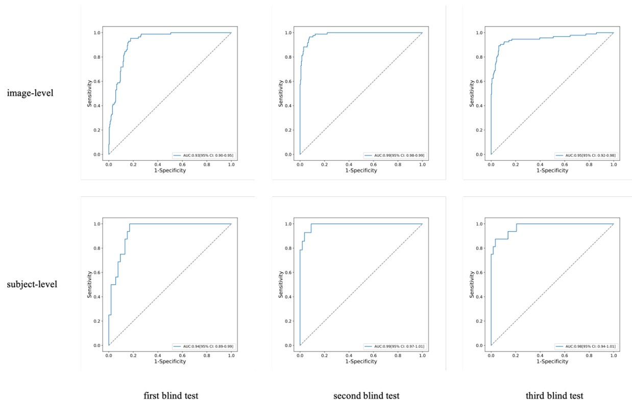
Figure 4. COVID-19 vs. Non-COVID-19 ROC curves on the three blind tests. The first row is image-level and the second row is subject-level.
