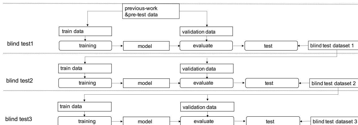
Figure 2. Study design and workflow of this study.
