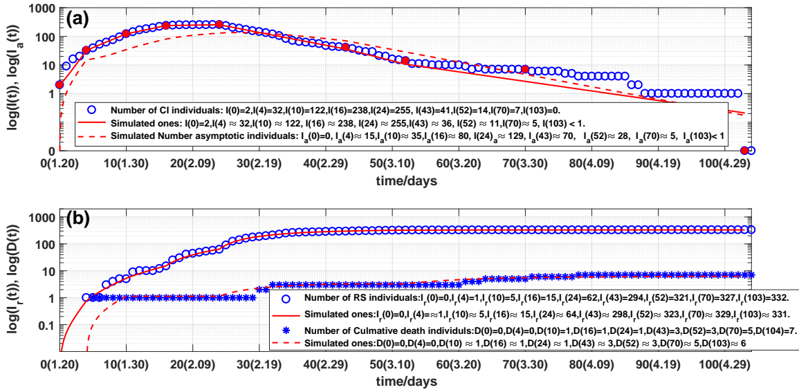
Figure 3: (a) Outcome of the number of current symptomatic individuals, representing by circles. Solid line and dash line are outcomes of stimulated current symptomatic individuals and stimulated current asymptomatic individuals of system (1). (b) Outcomes of the numbers of cumulative recovered symptomatic and died individuals, representing by circles and stars, respectively. Solid line and dash line are corresponding simulations of system (1).
