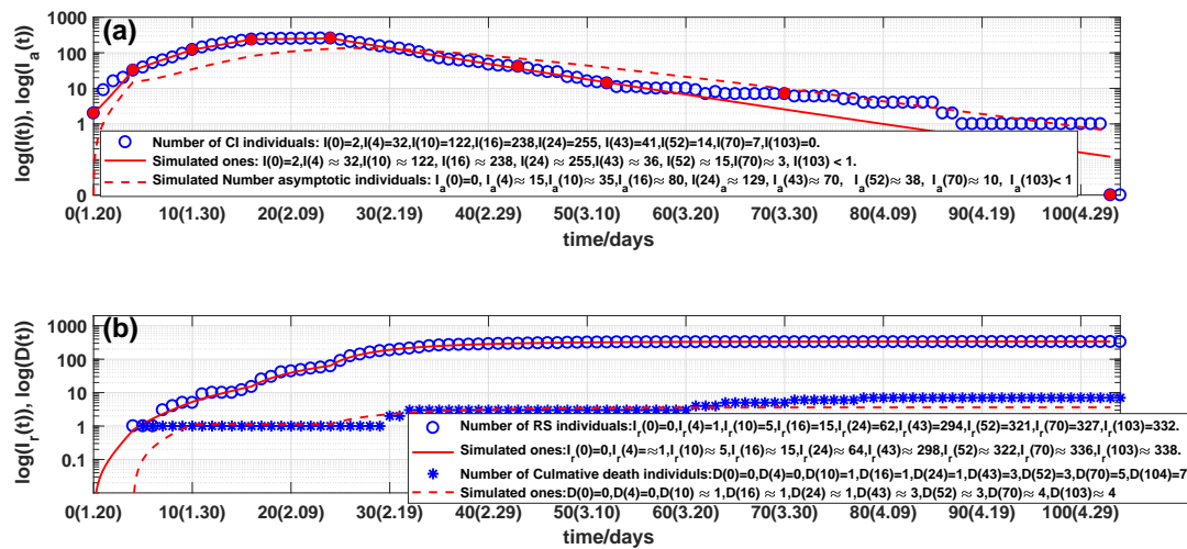
Figure 5: Outcomes of the numbers of:(a) current symptomatic individuals, representing by circles. Solid line and dash line are the stimulated current symptomatic and asymptomatic of system (1); (b) cumulative recovered symptomatic and died individuals, representing by circles and stars, respectively. Solid line and dash line are corresponding simulations of system (1).
