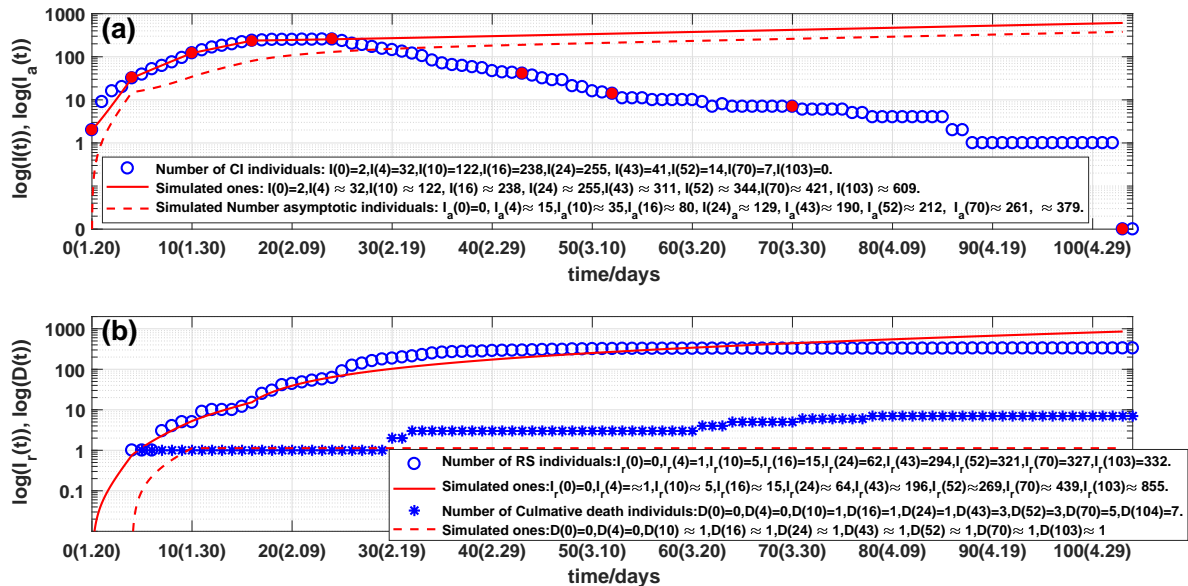
Figure 4: Outcomes of the numbers of:(a) current symptomatic individuals, representing by circles. Solid line and dash line are the stimulated current symptomatic and asymptomatic individuals of system (1); (b) cumulative recovered symptomatic and died individuals, representing by circles and stars, respectively. Solid line and dash line are corresponding simulations of system (1).
