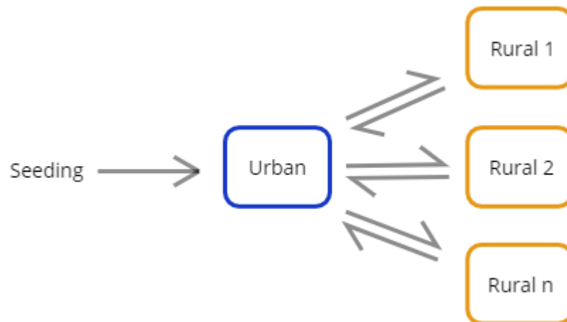
Figure 6: Model schematic showing sample node and migration. Infected individuals were seeded in the urban node and infection spread to rural nodes via urban-rural migration.
