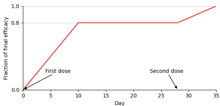
Figure 8: Ramp-up of protective effect within a vaccinated individual in the model
