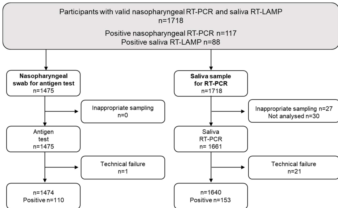
Figure 1. Study flowchart.
