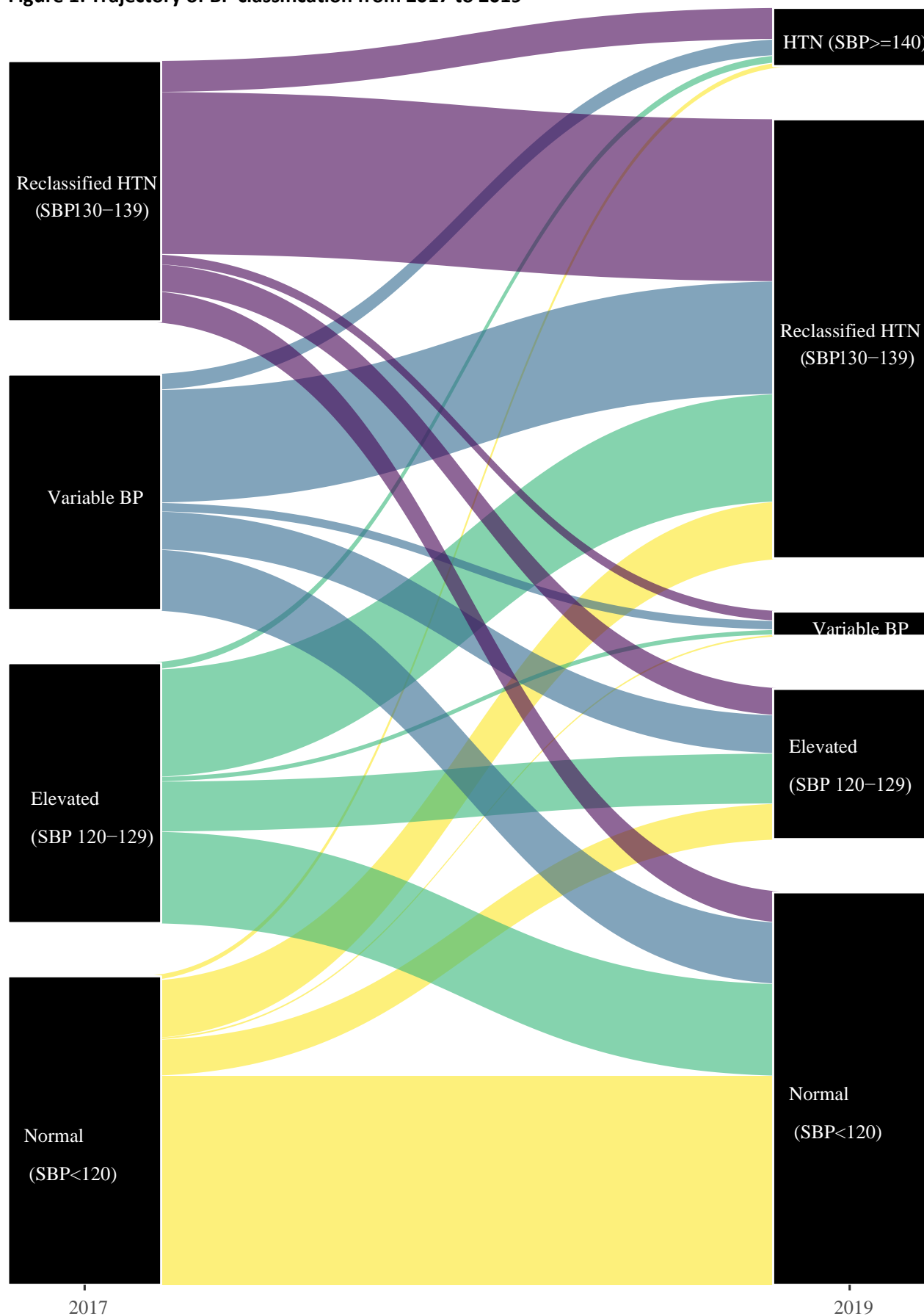
Figure 1: Trajectory of BP classification from 2017 to 2019
